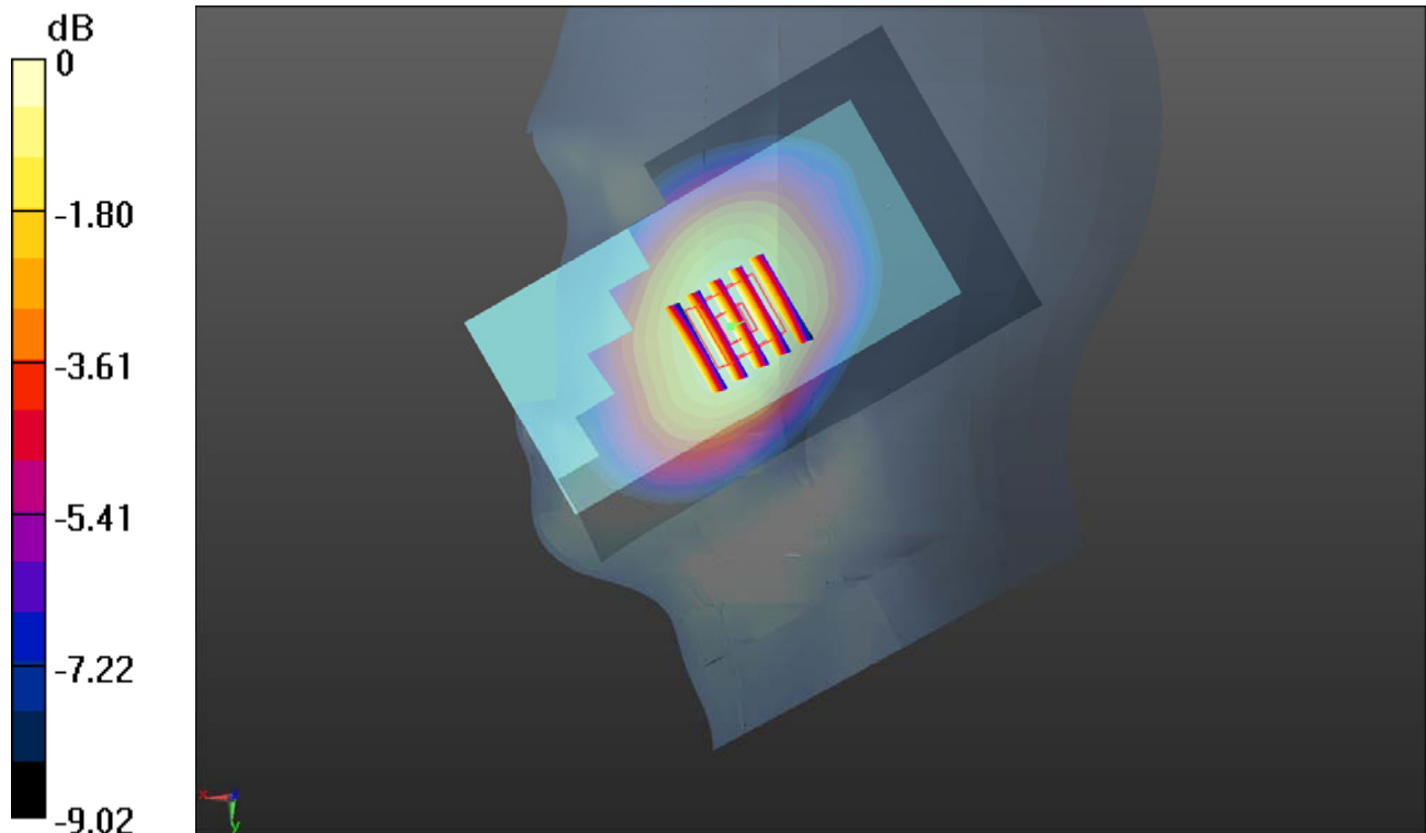
0 dB = 0.392 W/kg
