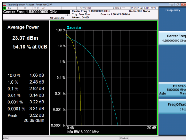
Channel 9400 / 1880.0 MHz
