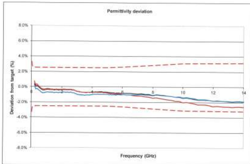
Fig. 4.1 HSL permittivity deviation from target, 200 MHz – 14 GHz
