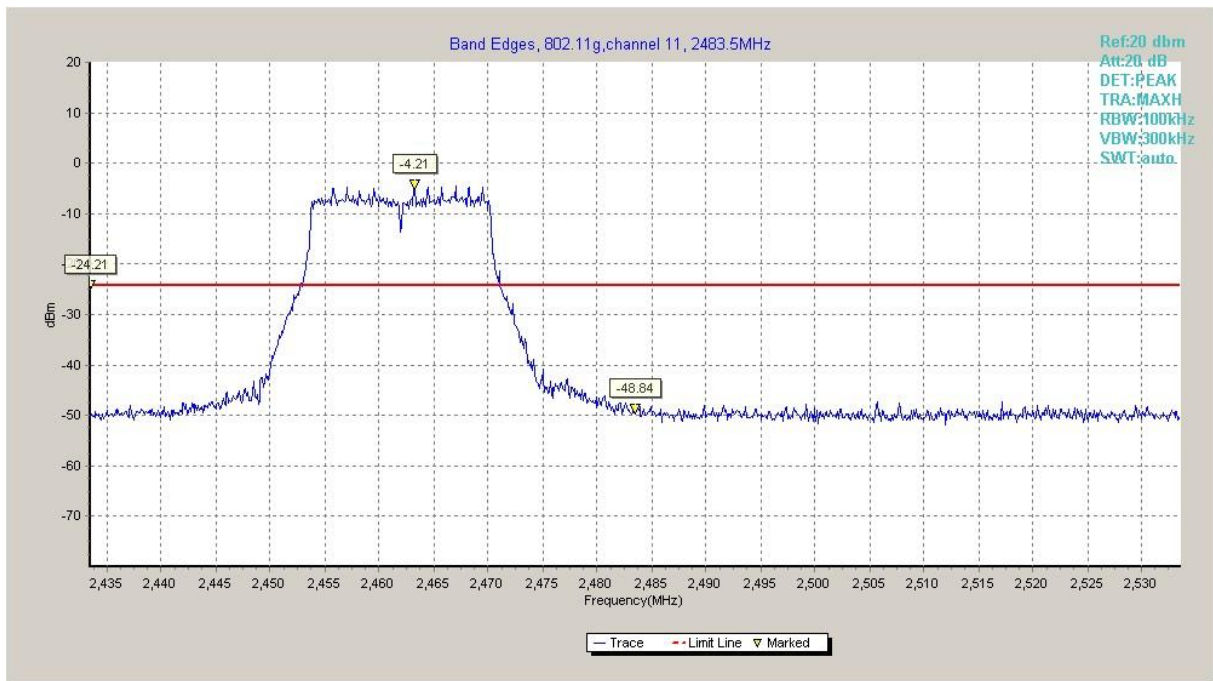
Fig.A.5.7 Band Edges (802.11g, Ch 11)
