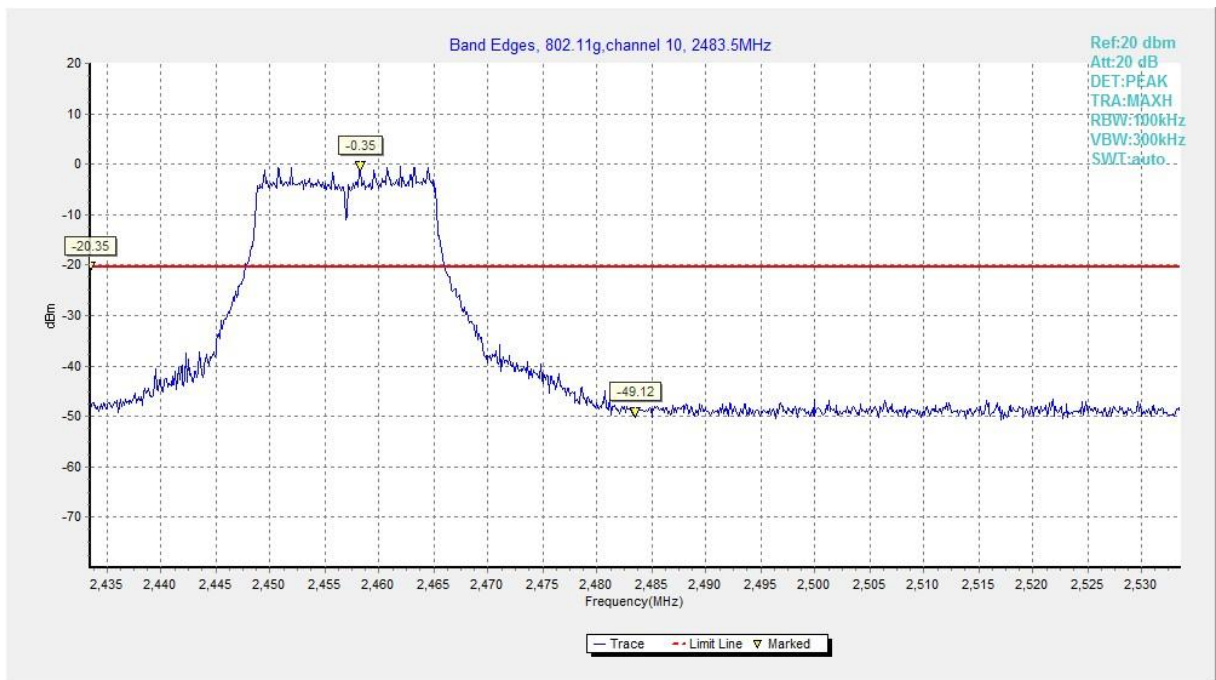
Fig.A.5.6 Band Edges (802.11g, Ch 10)
