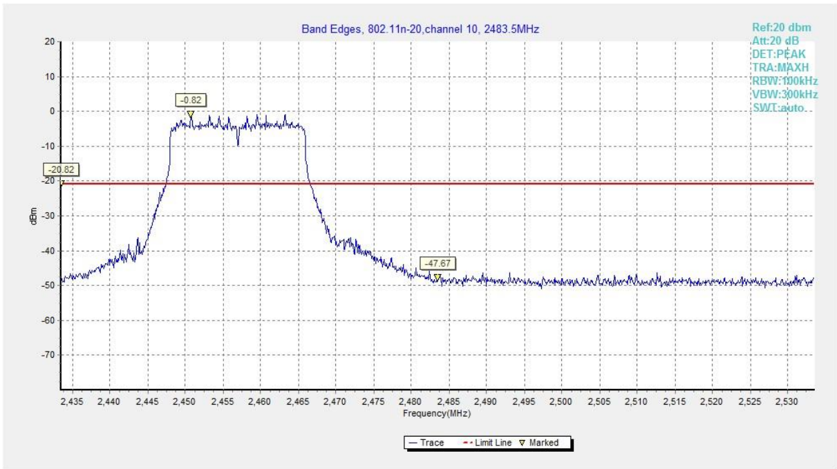
Fig.A.5.11 Band Edges (802.11n-HT20, Ch 10)
