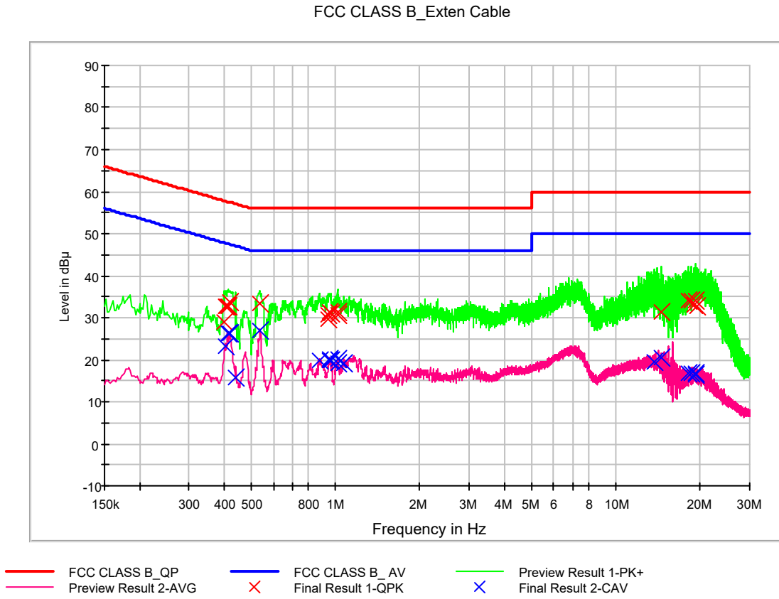
Figure 2: Conducted Emission (0.15 to 30) MHz, Line (N)
