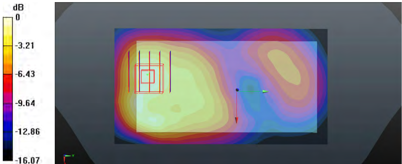
0 dB = 0.645 W/kg
