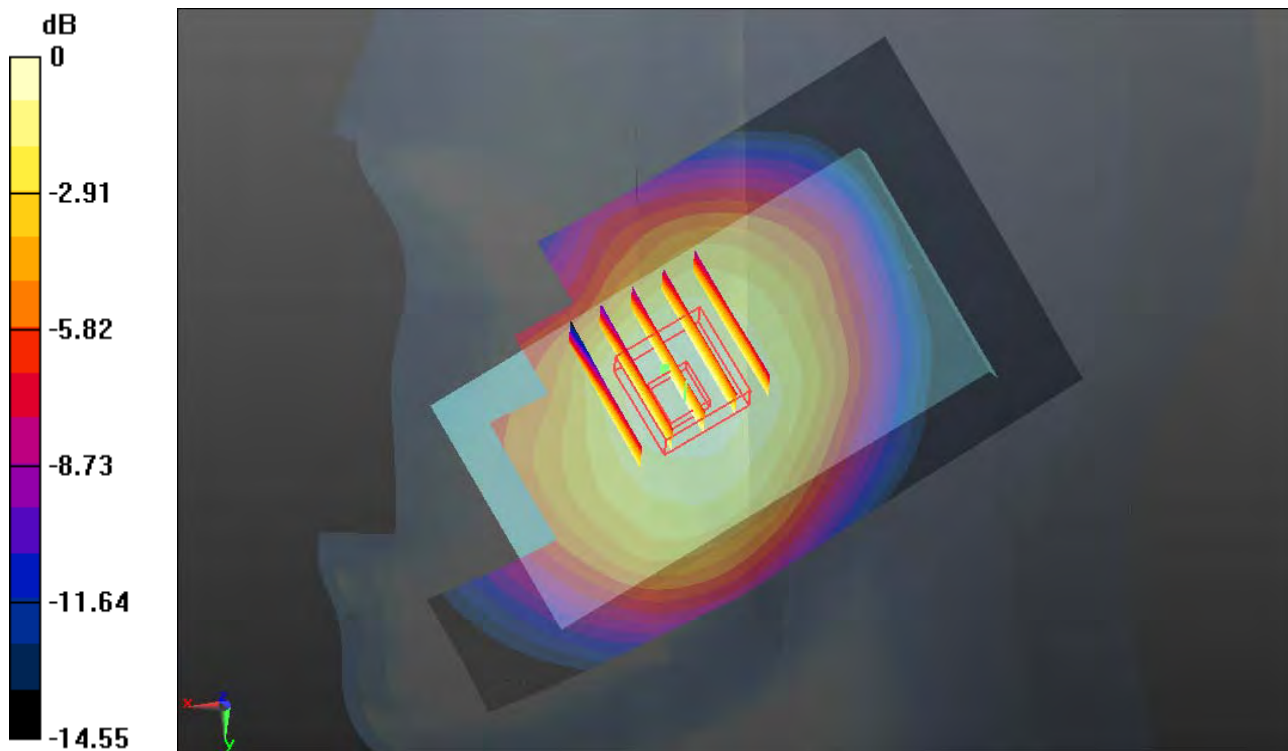
0 dB = 0.590mW/g
