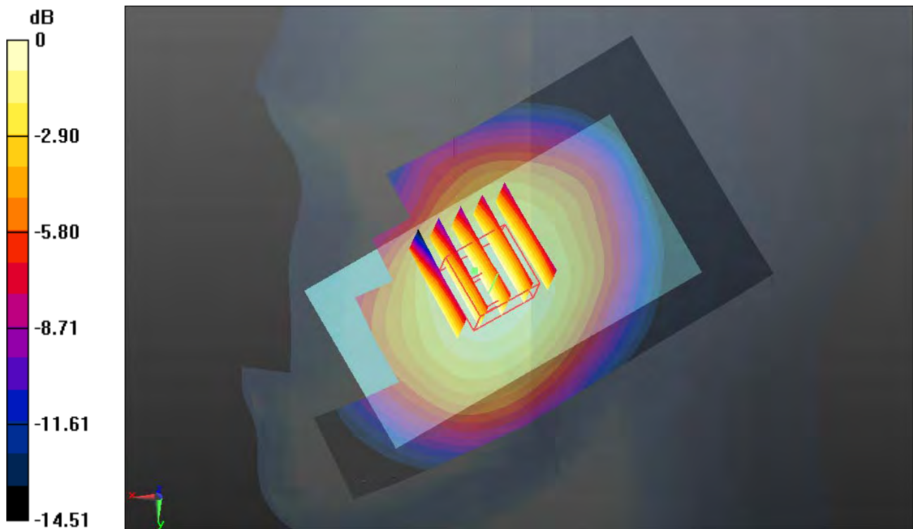
0 dB = 0.630mW/g
