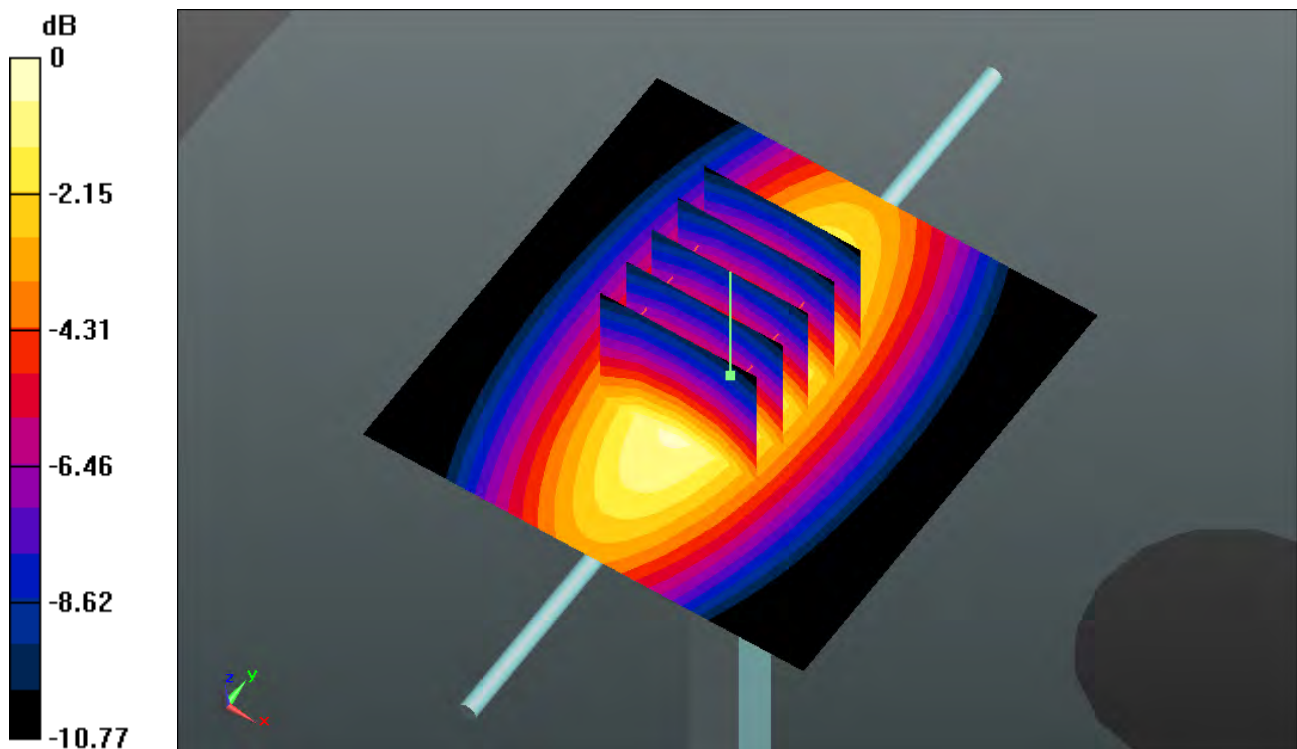
0 dB = 3.090\text{mW/g}
