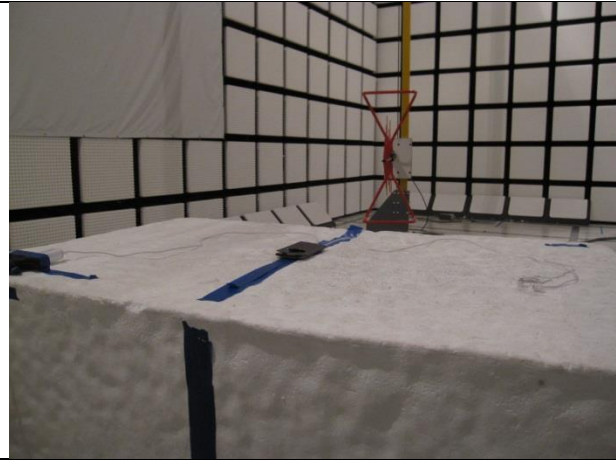
RADIATED EMISSION Smart Cover PHOTO
