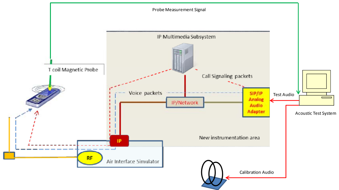
Figure 7-1 Test Setup for VoLTE T-Coil Measurements
