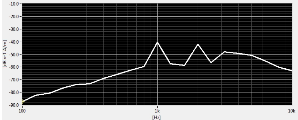
Figure 8-5 Worst-case ABM2 Plot for WD, LTE
