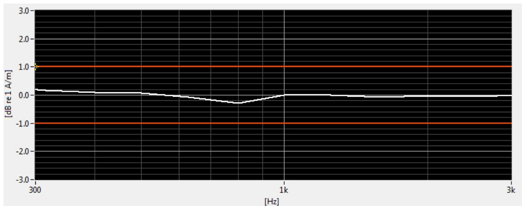
Figure 8-6 Helmholtz Coil Validation for Frequency Response
