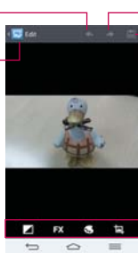
Editing Screen
