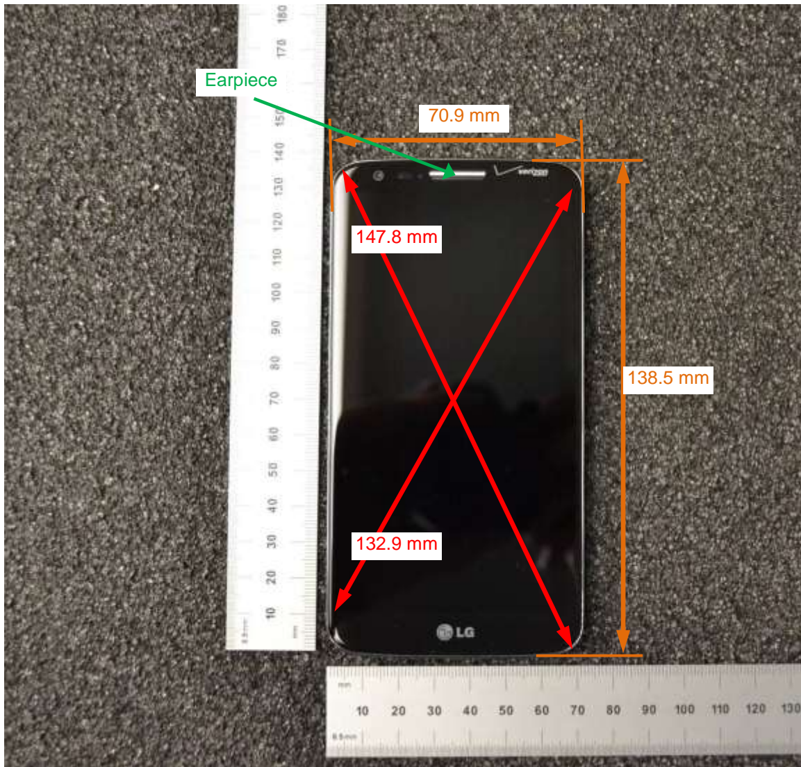
Overall Dimensions
