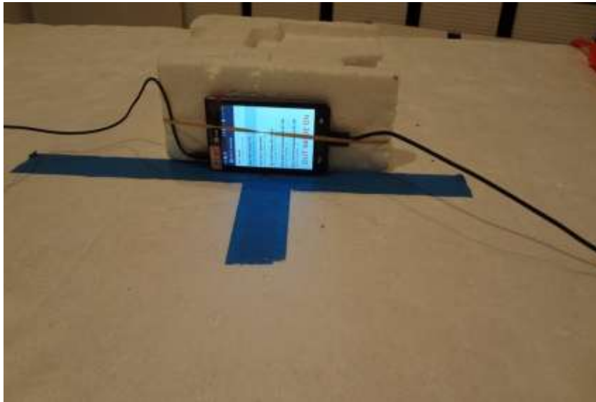
Z-AXIS PHOTO
