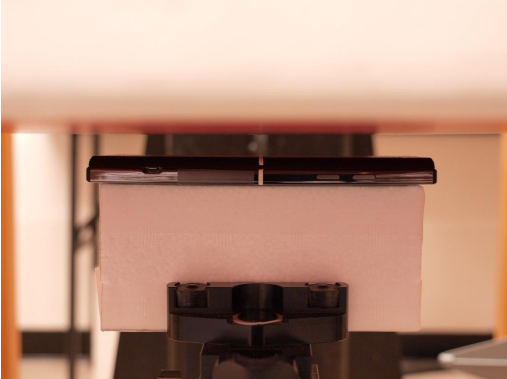
Body & Hotspot - Rear with 10 mm Separation (with Wireless Charging Battery Cover)
