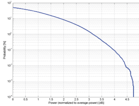
Complementary Cumulative Distribution Function (CCDF)
