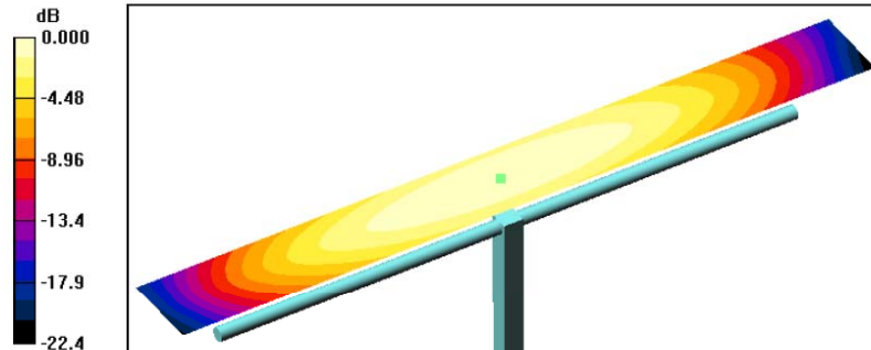
0 dB = 0.465A/m
