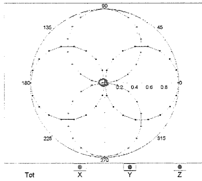
f=600 MHz,TEM,0°
