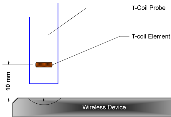
Figure 5-10 Measurement Distance
