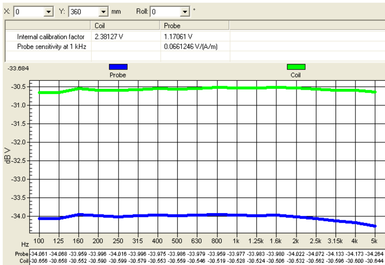
Figure 3: Frequency Response measured in AMCC
