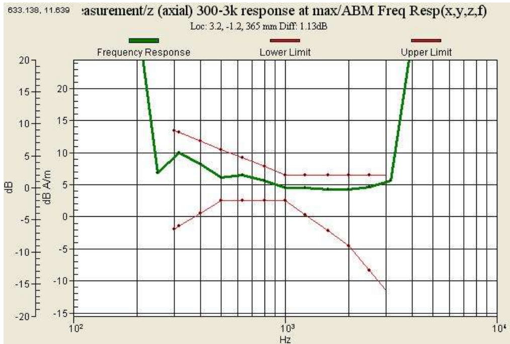
Graph 7 : CDMA 800 (CH 384) Frequency Response
