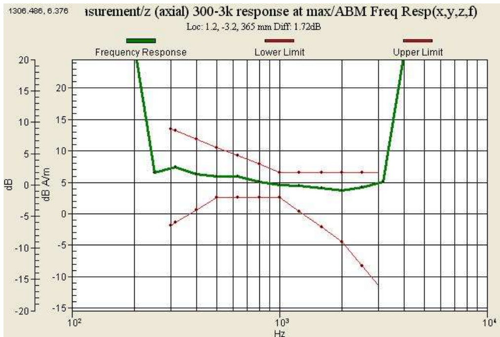
Graph 8 : PCS 1900 (CH 25) Frequency Response
