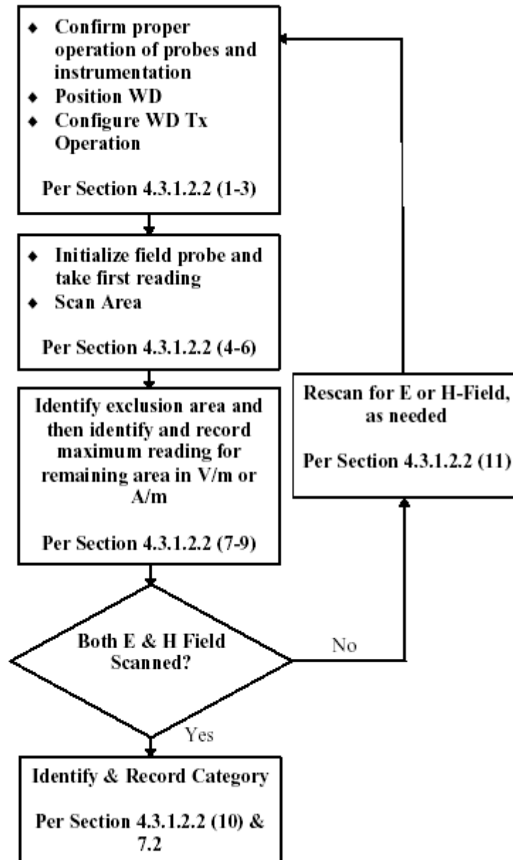
Figure 9. WD near-field emission automated test flowchart
