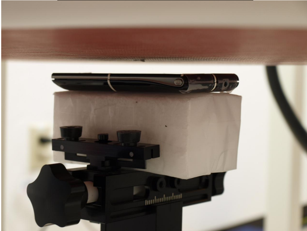
Body-worn & hotspot - Front w/ 10 mm Separation
