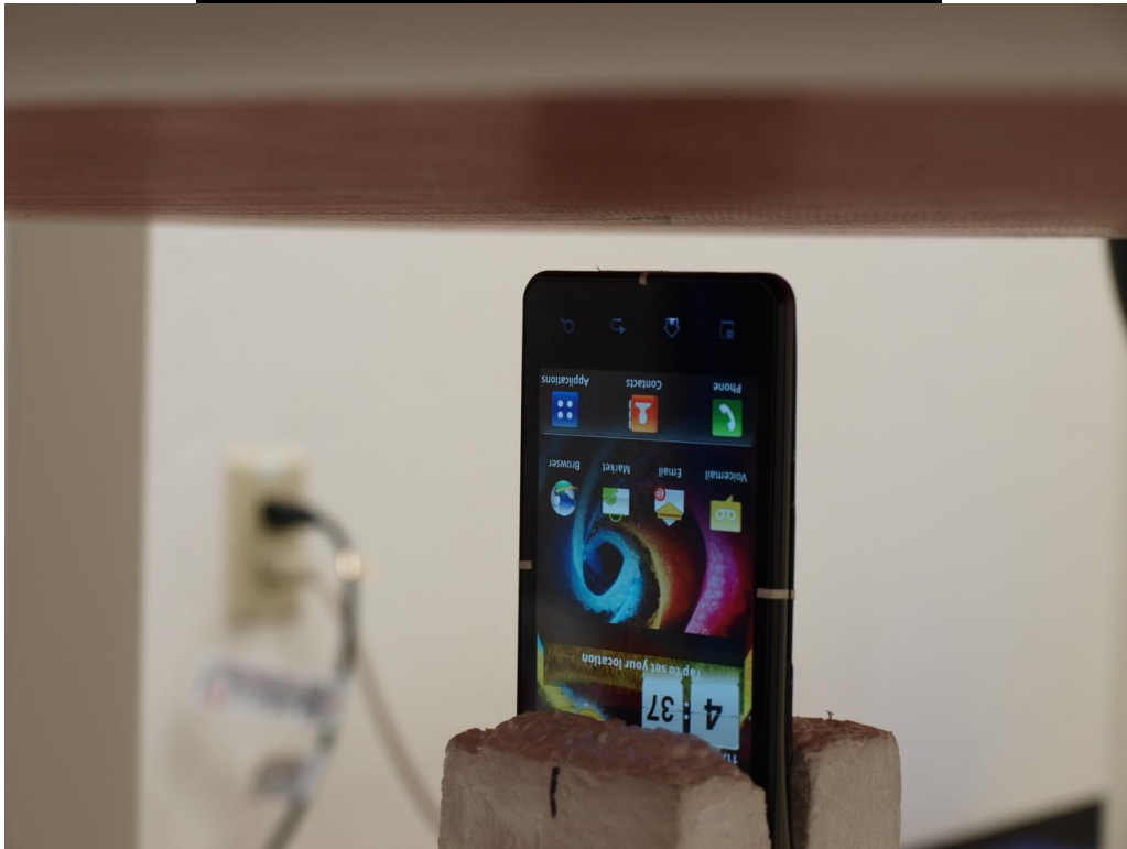
Body-worn & hotspot - Bottom w/ 10 mm Separation
