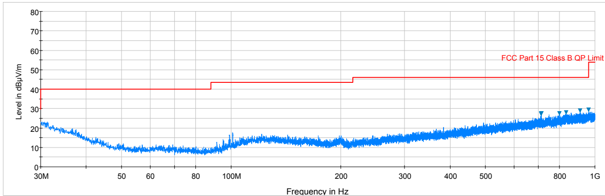
Plot 7-17. Radiated Spurious Plot below 1GHz (Pol. H)
