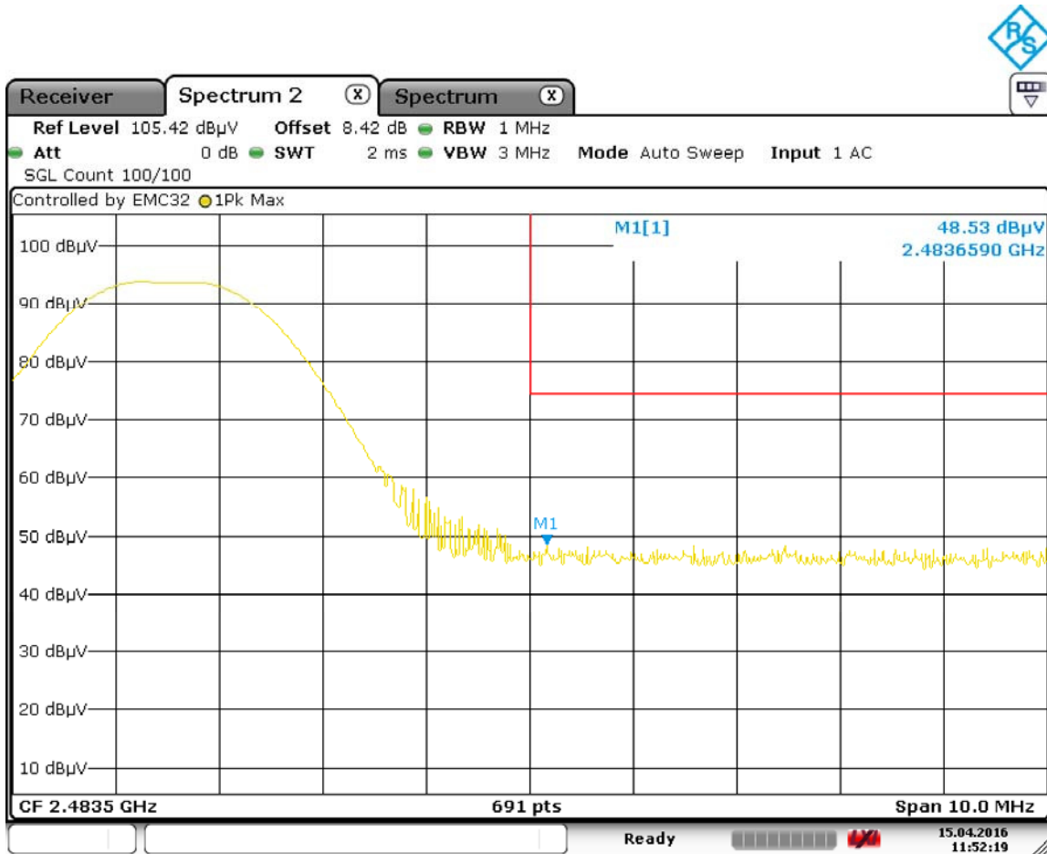
Plot 7-2. Radiated Restricted Upper Band Edge Measurement (Peak)
