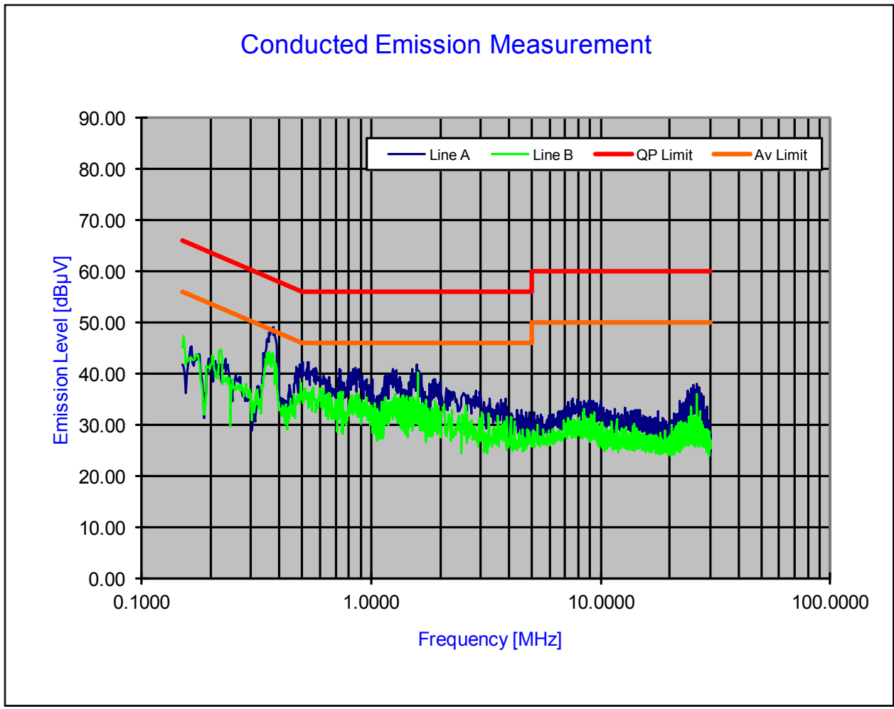
Plot 6-20. Line Conducted Plot with Bluetooth (LE)
