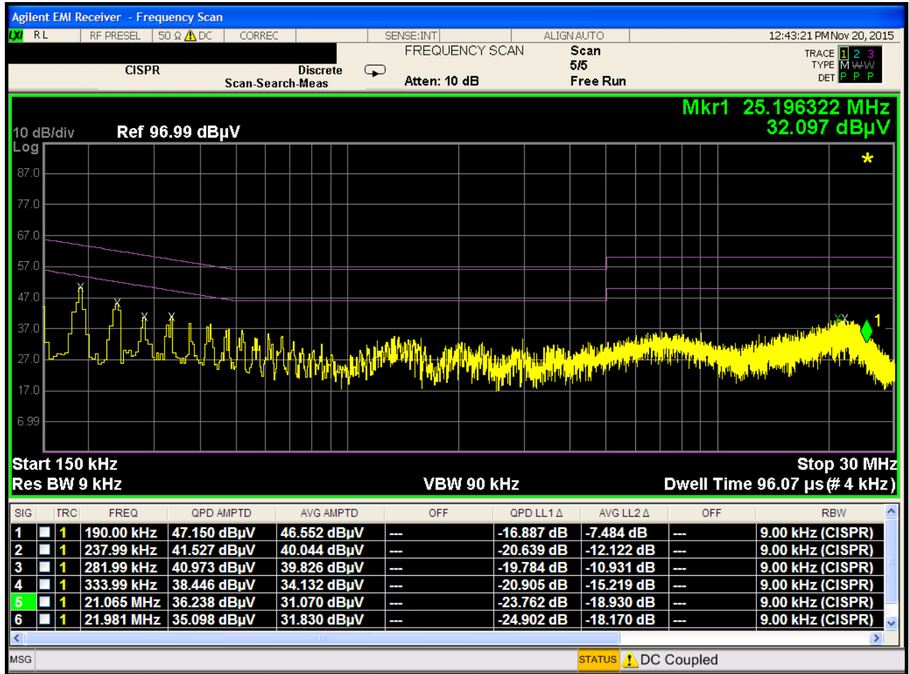
Plot 7-57. Line Conducted Plot with 802.11b (L1) Additional AC Adapter EAY64329102
