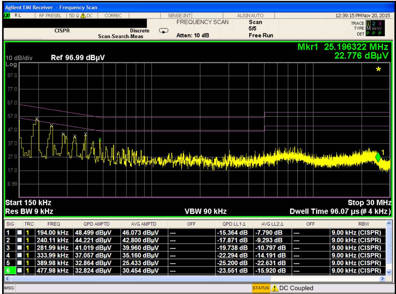
Plot 7-58. Line Conducted Plot with 802.11b (N) Additional AC Adapter EAY64329102
