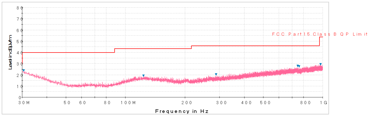
Plot 6-14. Radiated Spurious Plot below 1GHz (Pol. V)
