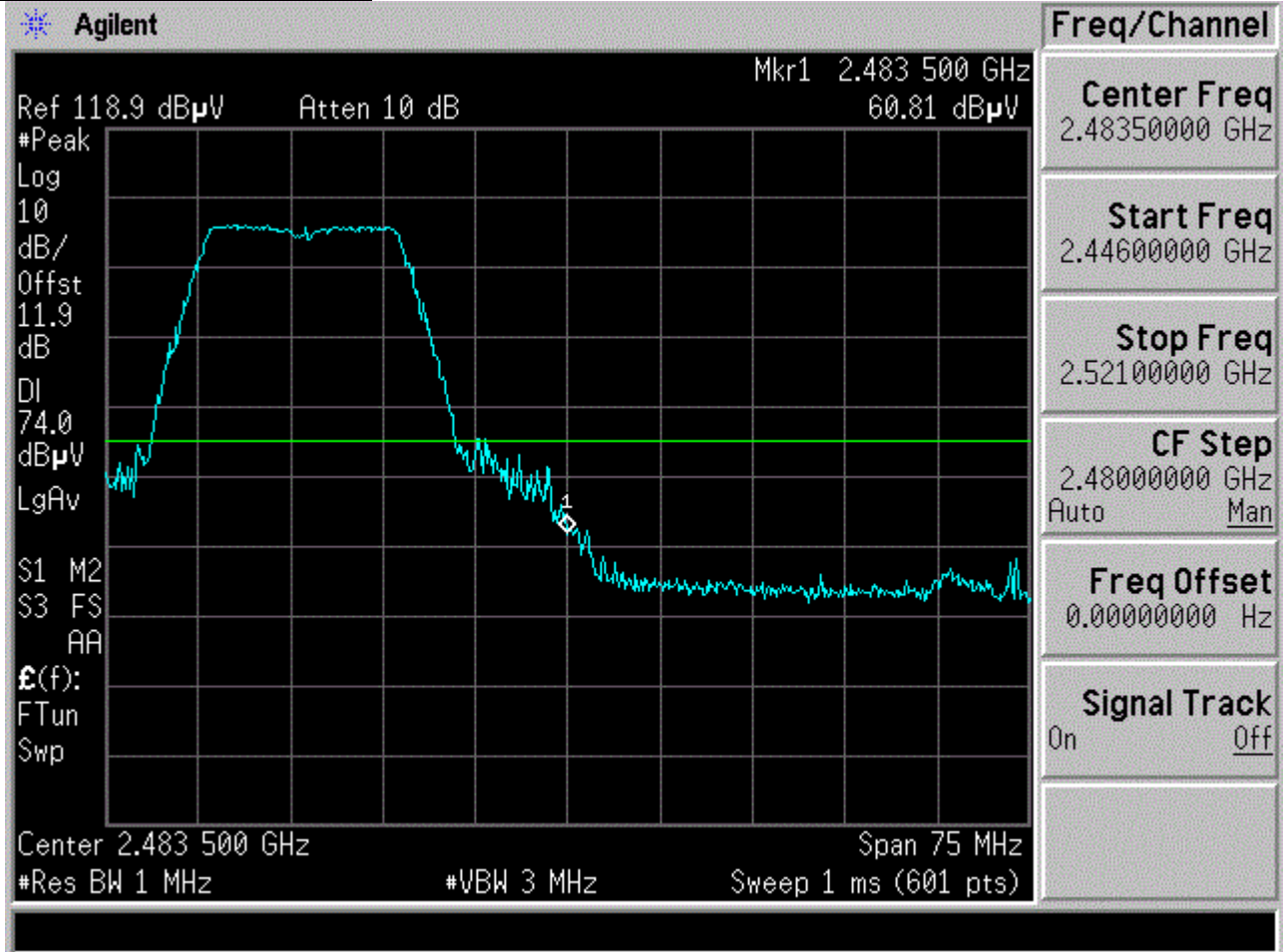
Plot 6-4. Radiated Restricted Upper Band Edge Measurement (Peak)
