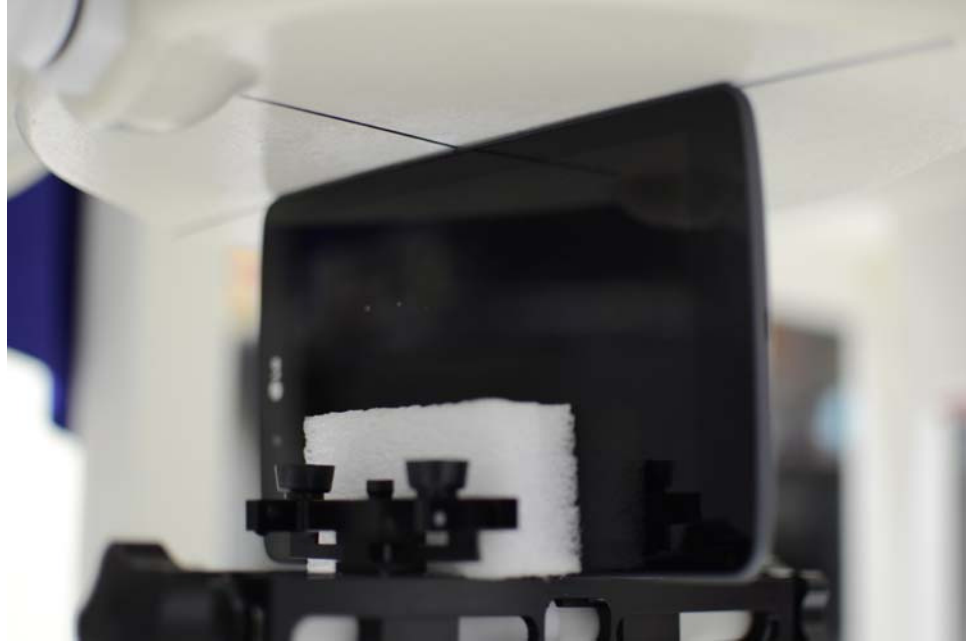
SAR Test Setup Photo 5: Right Edge at 0 mm
