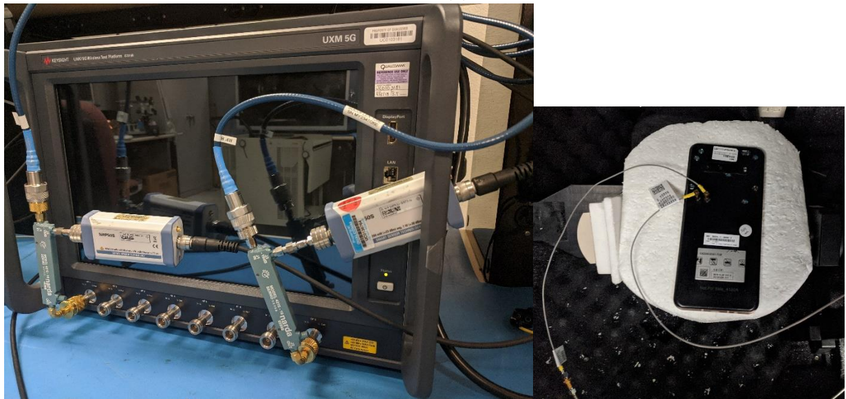
Figure 5-1 Conducted power measurement setup
