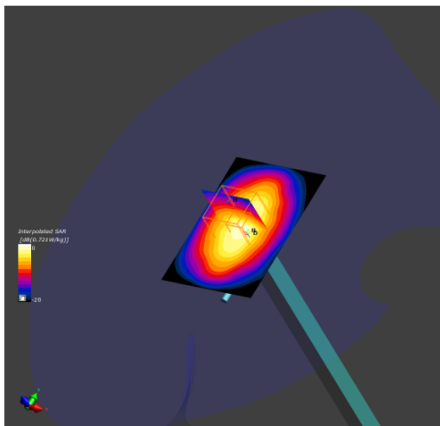
Figure C-5 SAR measurement system verification plot for 1800MHz performed on 3/11/2020. Input power = 10.0mW.
