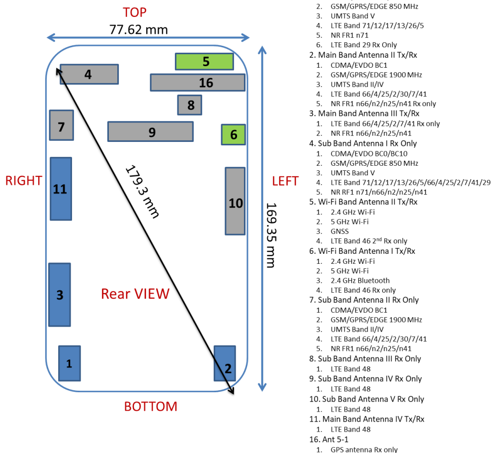
Figure E-1 DUT Antenna Locations
