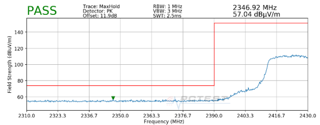
Plot 7-144. Radiated Restricted Lower Band Edge Measurement MIMO (Peak)
