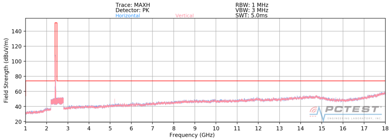
Plot 7-117. Radiated Spurious Plot above 1GHz MIMO/CDD (802.11g – Ch. 1)
