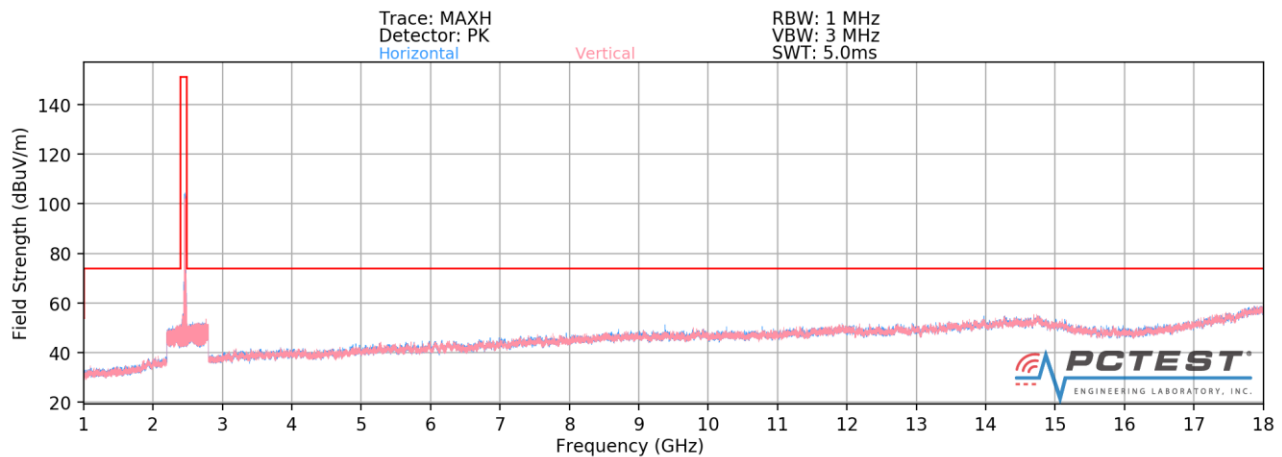
Plot 7-115. Radiated Spurious Plot above 1GHz SISO ANT2 (802.11b – Ch. 11)
