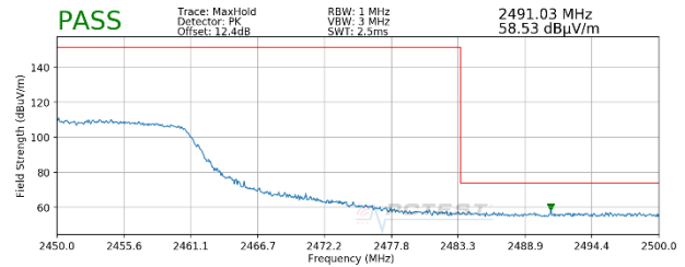
Plot 7-146. Radiated Restricted Upper Band Edge Measurement MIMO (Peak)
