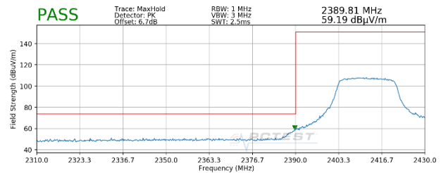
Plot 7-122. Radiated Restricted Lower Band Edge Measurement SISO ANT1 (Peak)
