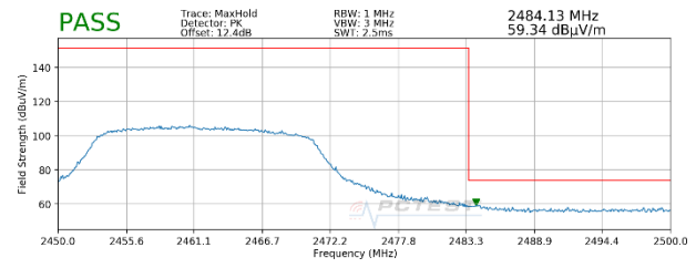
Plot 7-138. Radiated Restricted Upper Band Edge Measurement SISO ANT2 (Peak)
