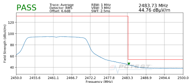
Plot 7-129. Radiated Restricted Band Edge Measurement SISO ANT1 with WCP (Average)
