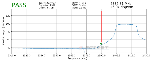
Plot 7-121. Radiated Restricted Lower Band Edge Measurement SISO ANT1 (Average)
