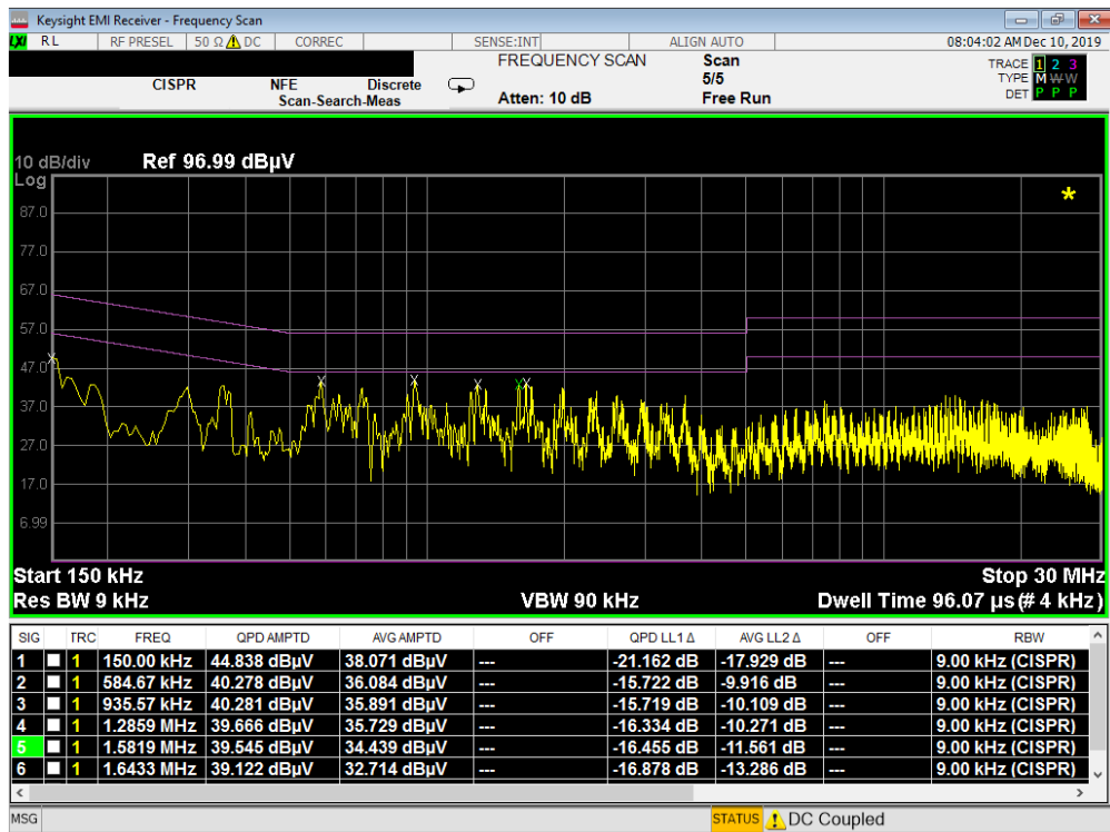
Plot 7-154. Line Conducted Plot with 802.11b (L1)
