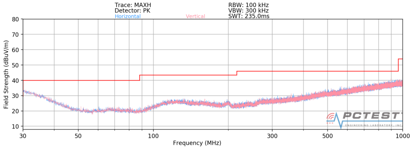
Plot 7-151. Radiated Spurious Plot below 1GHz SISO ANT1
