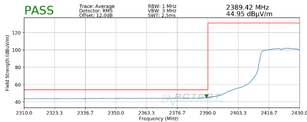
Plot 7-143. Radiated Restricted Lower Band Edge Measurement MIMO (Average)
