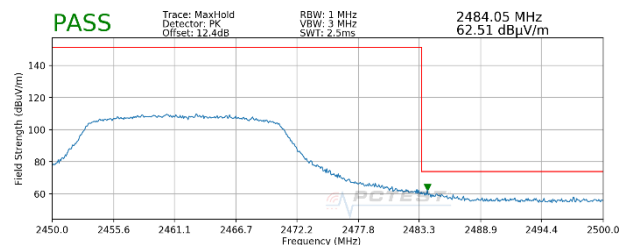
Plot 7-128. Radiated Restricted Upper Band Edge Measurement SISO ANT1 (Peak)
