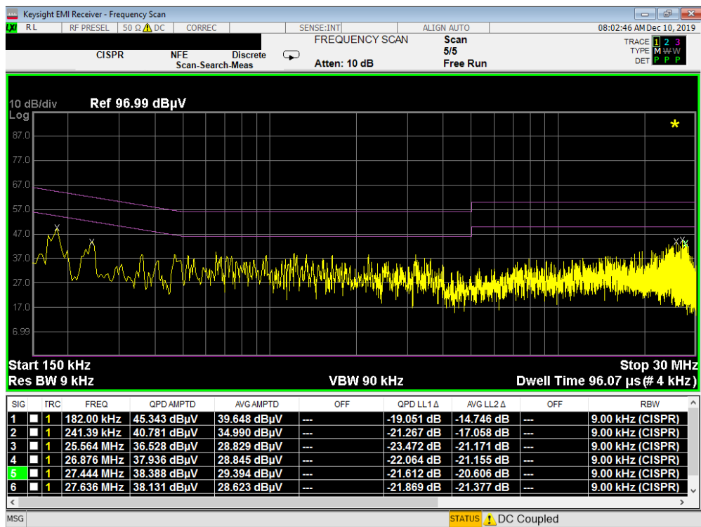
Plot 7-155. Line Conducted Plot with 802.11b (N)
