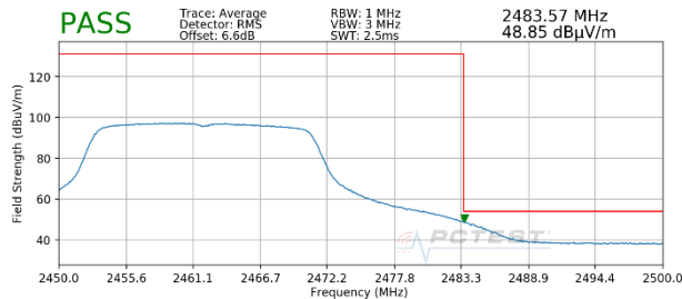
Plot 7-149. Radiated Restricted Band Edge Measurement MIMO with WCP (Average)
