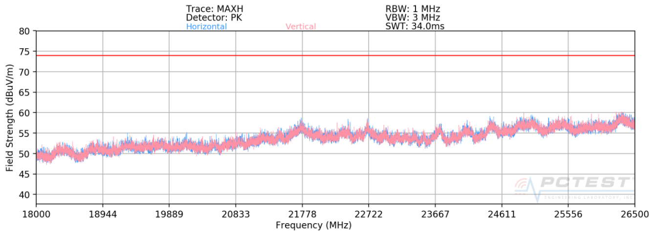
Plot 7-112. Radiated Spurious Plot above 18GHz SISO ANT1
