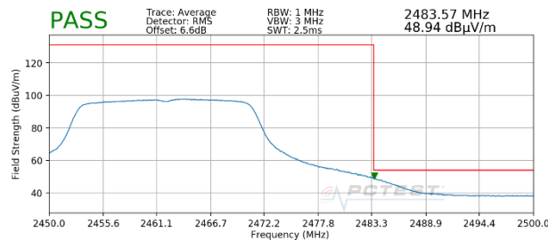
Plot 7-147. Radiated Restricted Upper Band Edge Measurement MIMO (Average)
