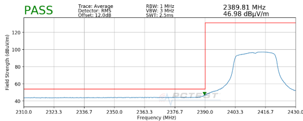
Plot 7-131. Radiated Restricted Lower Band Edge Measurement SISO ANT2 (Average)
