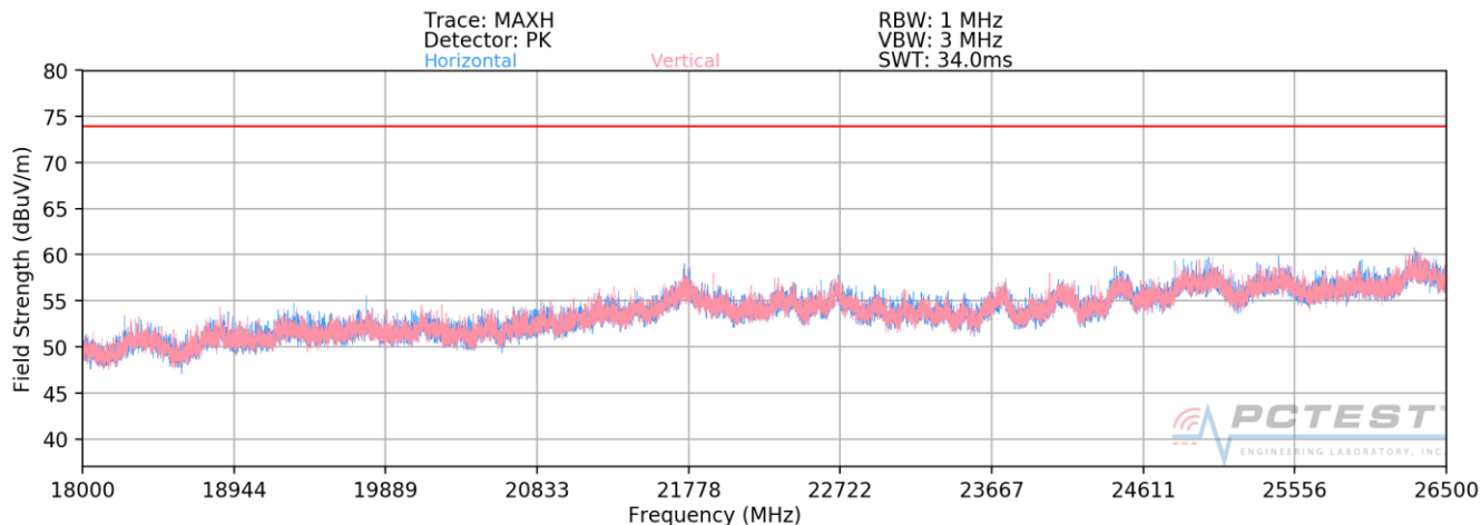
Plot 7-116. Radiated Spurious Plot above 18GHz SISO ANT2
