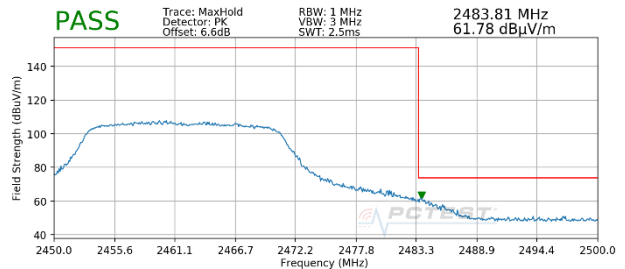
Plot 7-150. Radiated Restricted Band Edge Measurement MIMO with WCP (Peak)
