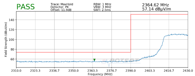
Plot 7-124. Radiated Restricted Upper Band Edge Measurement SISO ANT1 (Peak)
