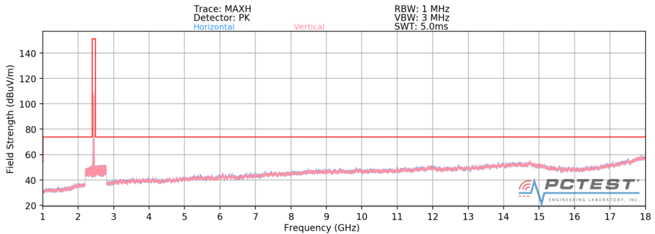
Plot 7-118. Radiated Spurious Plot above 1GHz MIMO/CDD (802.11g – Ch. 6)
