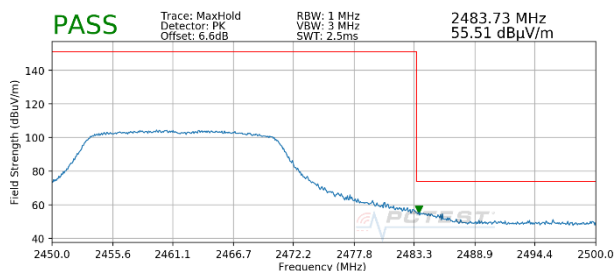
Plot 7-130. Radiated Restricted Band Edge Measurement SISO ANT1 with WCP (Peak)
