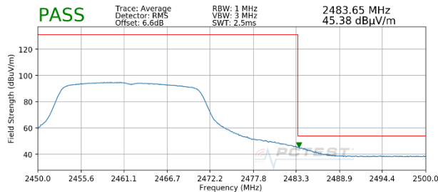
Plot 7-139. Radiated Restricted Band Edge Measurement SISO ANT1 with WCP (Average)
