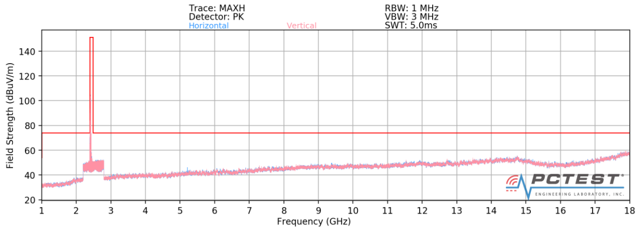
Plot 7-113. Radiated Spurious Plot above 1GHz SISO ANT2 (802.11b – Ch. 1)
