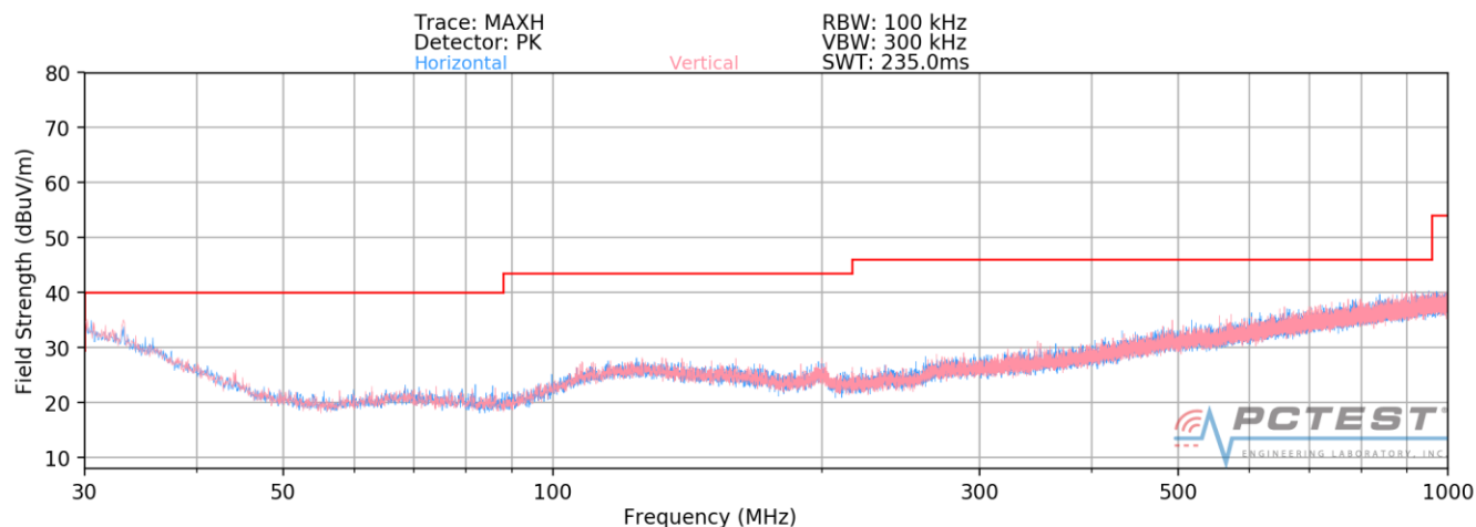
Plot 7-152. Radiated Spurious Plot below 1GHz SISO ANT2
