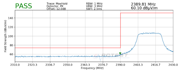
Plot 7-142. Radiated Restricted Lower Band Edge Measurement MIMO (Peak)
