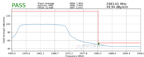
Plot 7-127. Radiated Restricted Upper Band Edge Measurement SISO ANT1 (Average)
