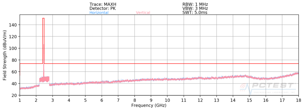
Plot 7-119. Radiated Spurious Plot above 1GHz MIMO/CDD (802.11g – Ch. 11)
