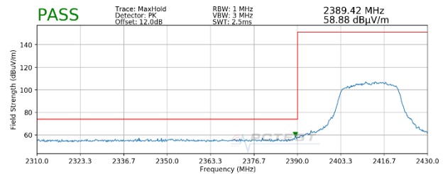
Plot 7-132. Radiated Restricted Lower Band Edge Measurement SISO ANT2 (Peak)
