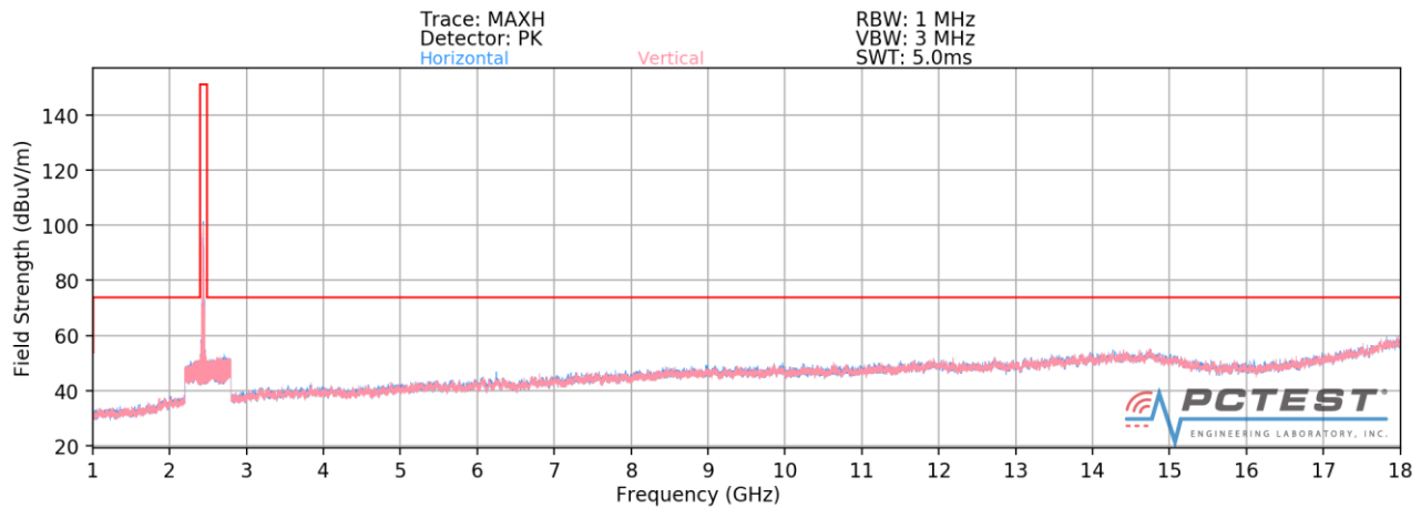
Plot 7-114. Radiated Spurious Plot above 1GHz SISO ANT2 (802.11b – Ch. 6)
