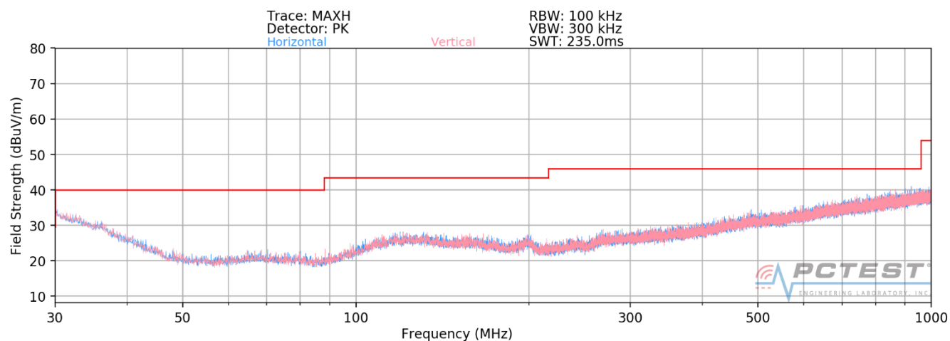
Plot 7-153. Radiated Spurious Plot below 1GHz MIMO
