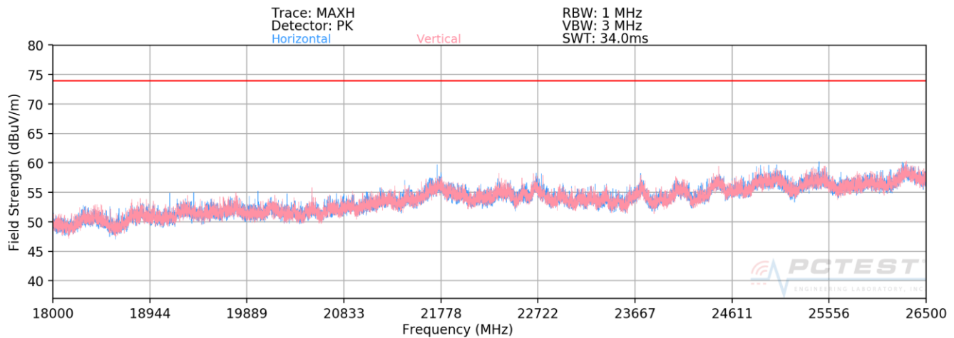
Plot 7-120. Radiated Spurious Plot above 18GHz MIMO/CDD
