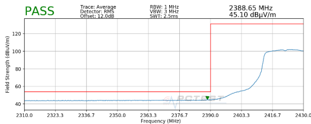
Plot 7-123. Radiated Restricted Upper Band Edge Measurement SISO ANT1 (Average)
