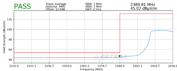
Plot 7-133. Radiated Restricted Upper Band Edge Measurement SISO ANT2 (Average)
