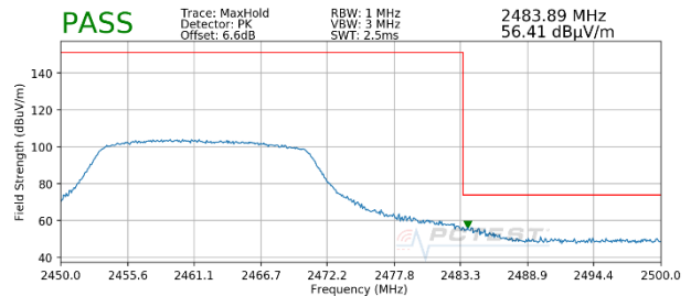
Plot 7-140. Radiated Restricted Band Edge Measurement SISO ANT1 with WCP (Peak)
