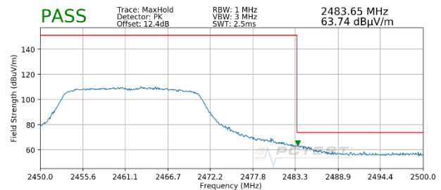
Plot 7-148. Radiated Restricted Upper Band Edge Measurement MIMO (Peak)
