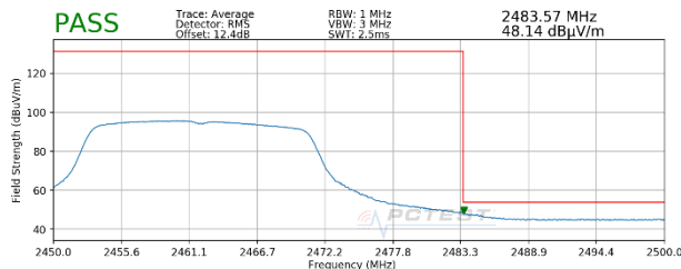
Plot 7-137. Radiated Restricted Upper Band Edge Measurement SISO ANT2 (Average)
