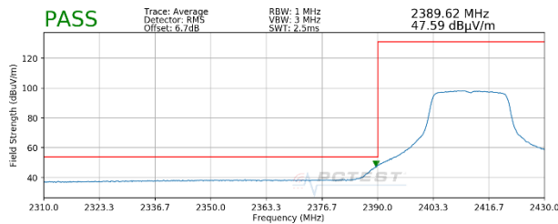
Plot 7-141. Radiated Restricted Lower Band Edge Measurement MIMO (Average)
