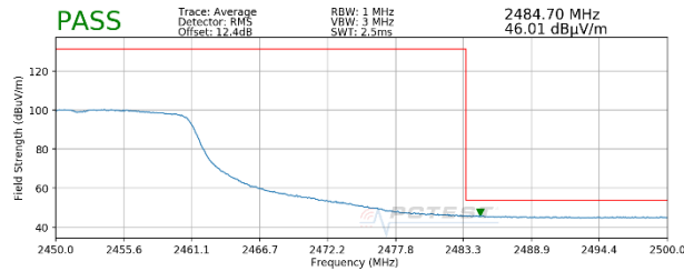
Plot 7-145. Radiated Restricted Upper Band Edge Measurement MIMO (Average)
