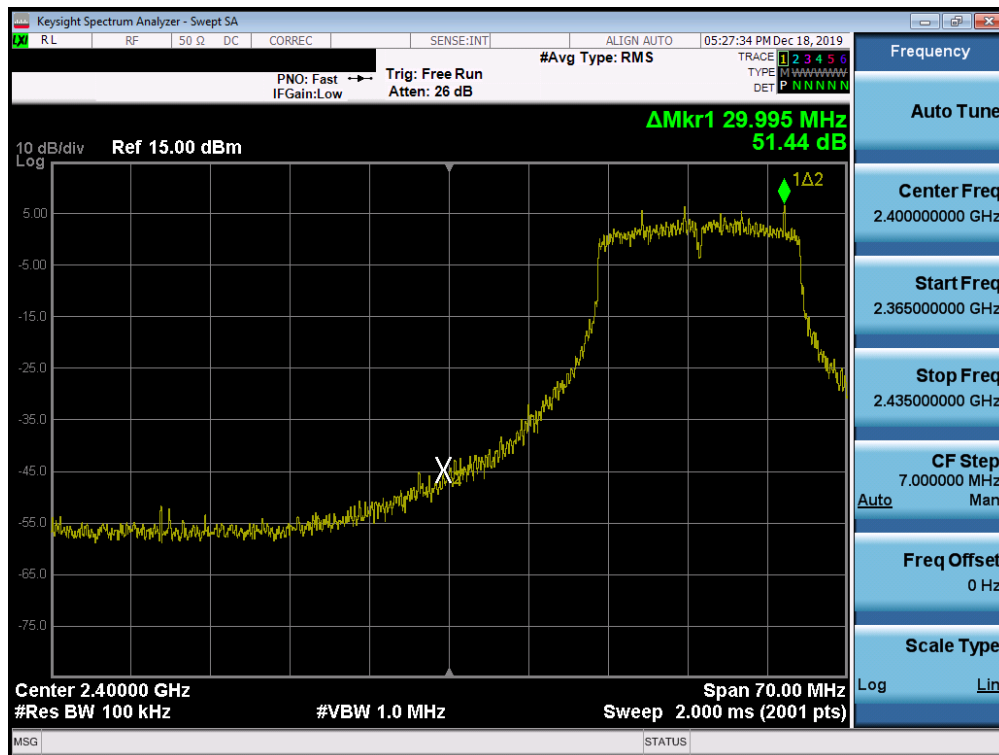
Plot 7-86. Band Edge Plot SISO ANT2 (802.11n– Ch. 3)
