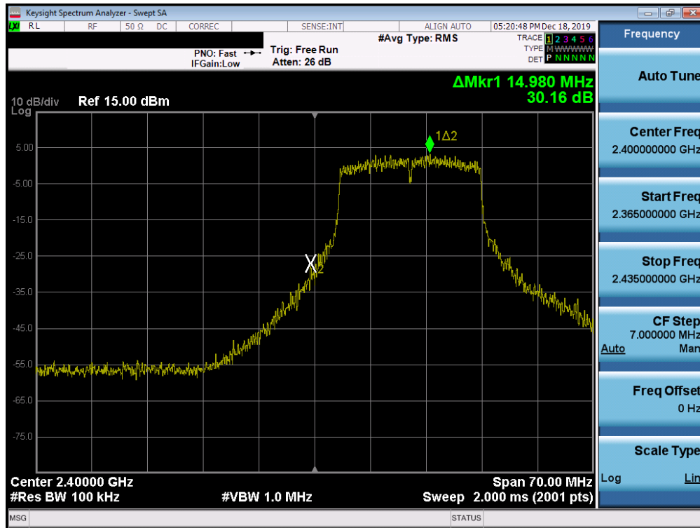
Plot 7-85. Band Edge Plot SISO ANT2 (802.11n (2.4GHz) – Ch. 1)
