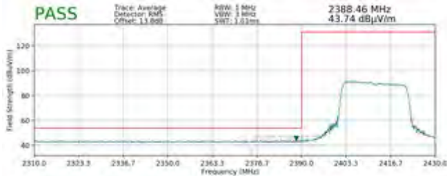
Plot 7-101. Radiated Restricted Lower Band Edge Measurement MIMO (Average – 242 Tones)
