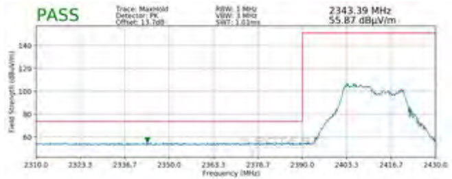
Plot 7-98. Radiated Restricted Lower Band Edge Measurement MIMO (Peak – 106 Tones)
