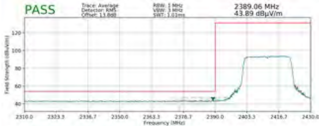
Plot 7-85. Radiated Restricted Lower Band Edge Measurement SISO ANT1 (Average – 242 Tones)
