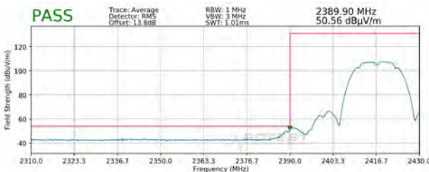
Plot 7-109. Radiated Restricted Lower Band Edge Measurement SISO ANT1 (Average)
