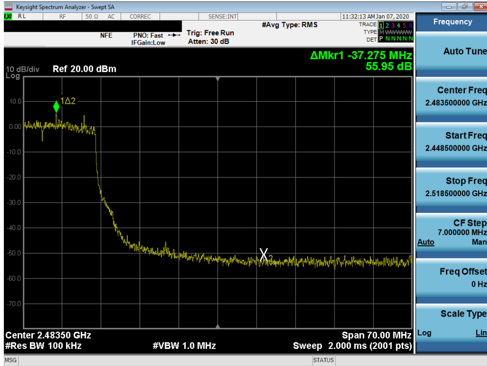
Plot 7-80. Band Edge Plot SISO ANT2 (802.11ax – Ch. 9)
