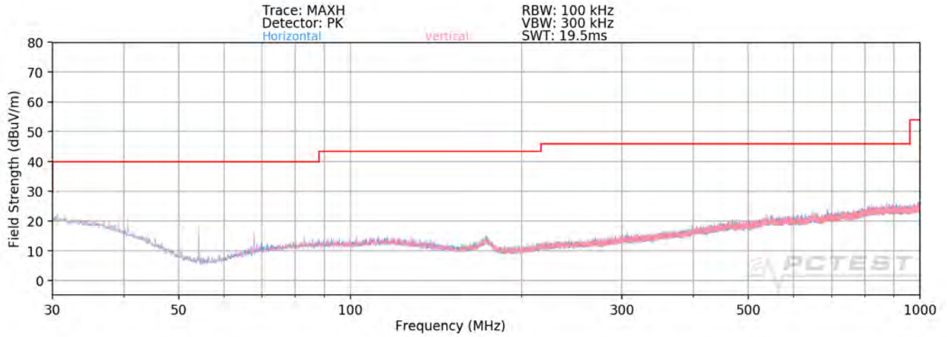
Plot 7-139. Radiated Spurious Plot below 1GHz SISO ANT1
