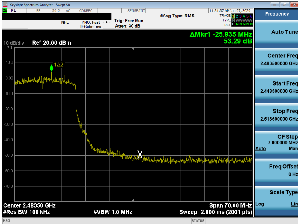
Plot 7-81. Band Edge Plot SISO ANT2 (802.11ax – Ch. 10)
