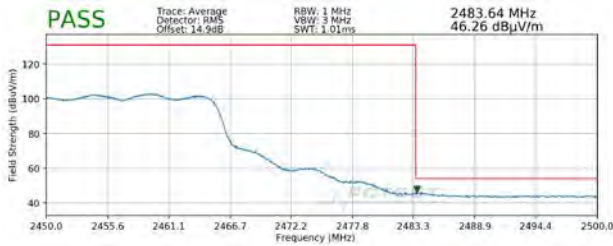
Plot 7-133. Radiated Restricted Upper Band Edge Measurement MIMO/CDD (Average)
