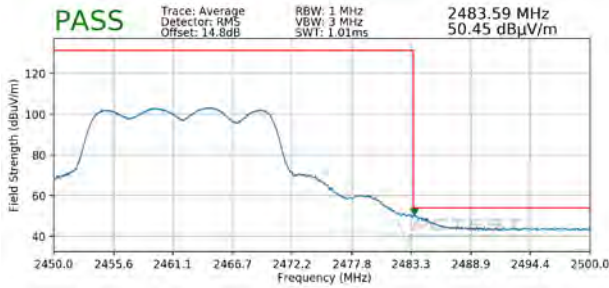
Plot 7-135. Radiated Restricted Upper Band Edge Measurement MIMO/CDD (Average)
