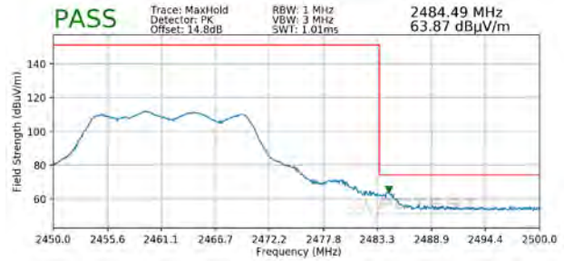
Plot 7-136. Radiated Restricted Upper Band Edge Measurement MIMO/CDD (Peak)
