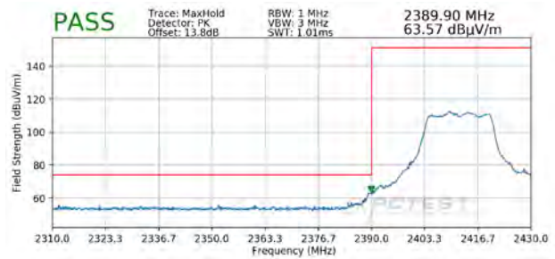
Plot 7-128. Radiated Restricted Lower Band Edge Measurement MIMO/CDD (Peak)
