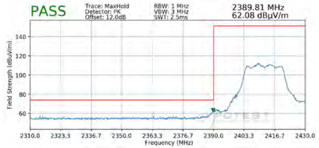
Plot 7-138. Radiated Restricted Band Edge Measurement MIMO/CDD with WCP + DD (Peak)
