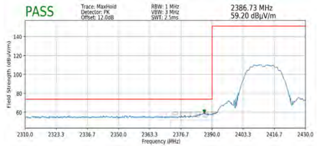
Plot 7-108. Radiated Restricted Lower Band Edge Measurement SISO ANT1 (Peak)
