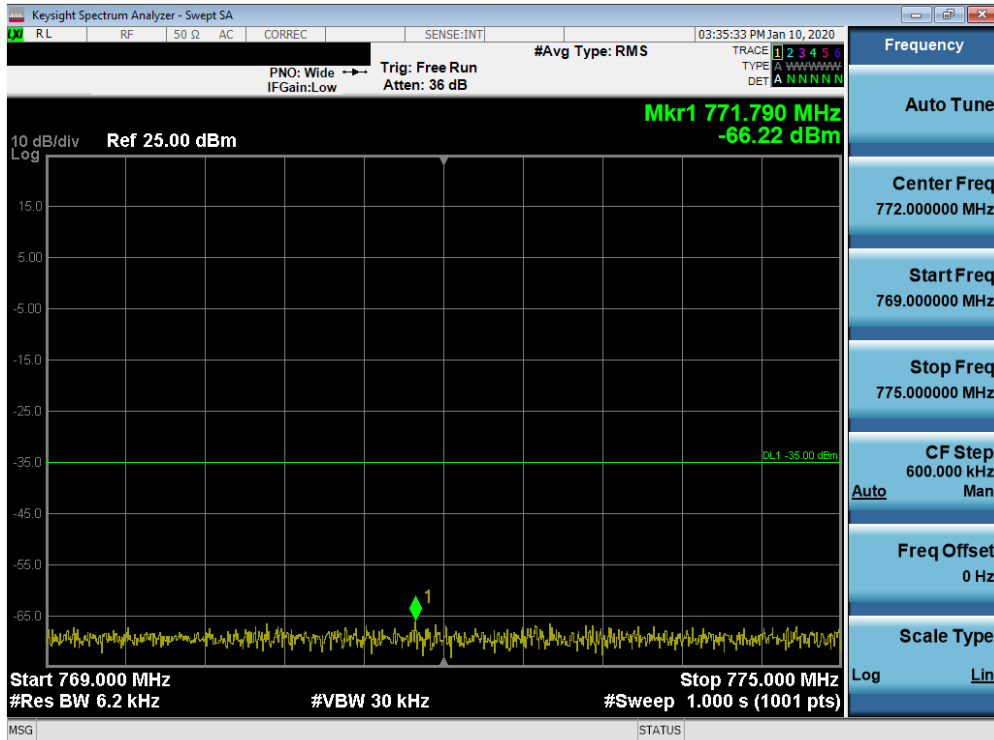
Plot 7-13. Lower Extended Band Edge Plot (Band 14 - 10MHz QPSK - Full RB Configuration)
