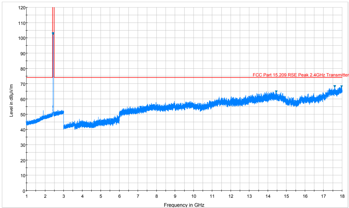
Plot 7-34. Radiated Spurious Plot above 1GHz (802.11b – Ch. 6, Ant. Pol. V)
