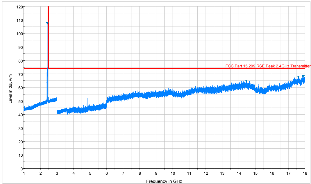
Plot 7-31. Radiated Spurious Plot above 1GHz (802.11b – Ch. 1, Ant. Pol. H)
