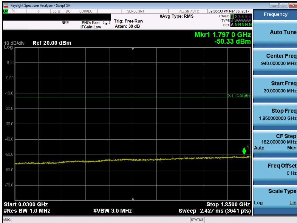
Plot 7-70. Conducted Spurious Plot (Band 2 – 15MHz QPSK – RB Size 1, RB Offset 0 – Mid Channel)
