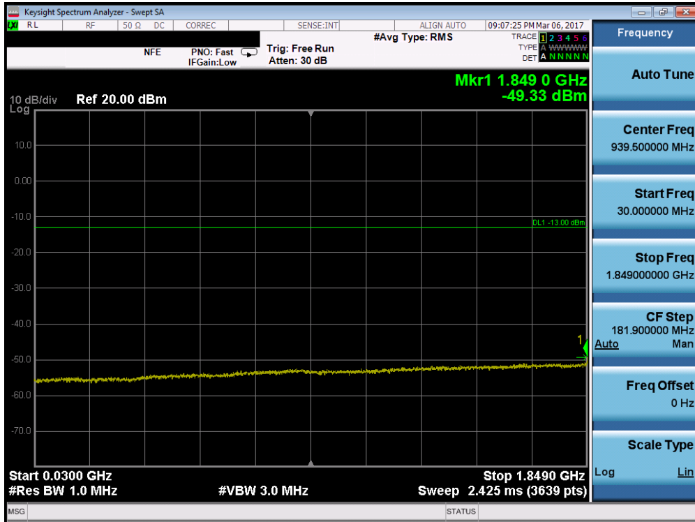
Plot 7-67. Conducted Spurious Plot (Band 2 – 15MHz QPSK – RB Size 1, RB Offset 0 – Low Channel)
