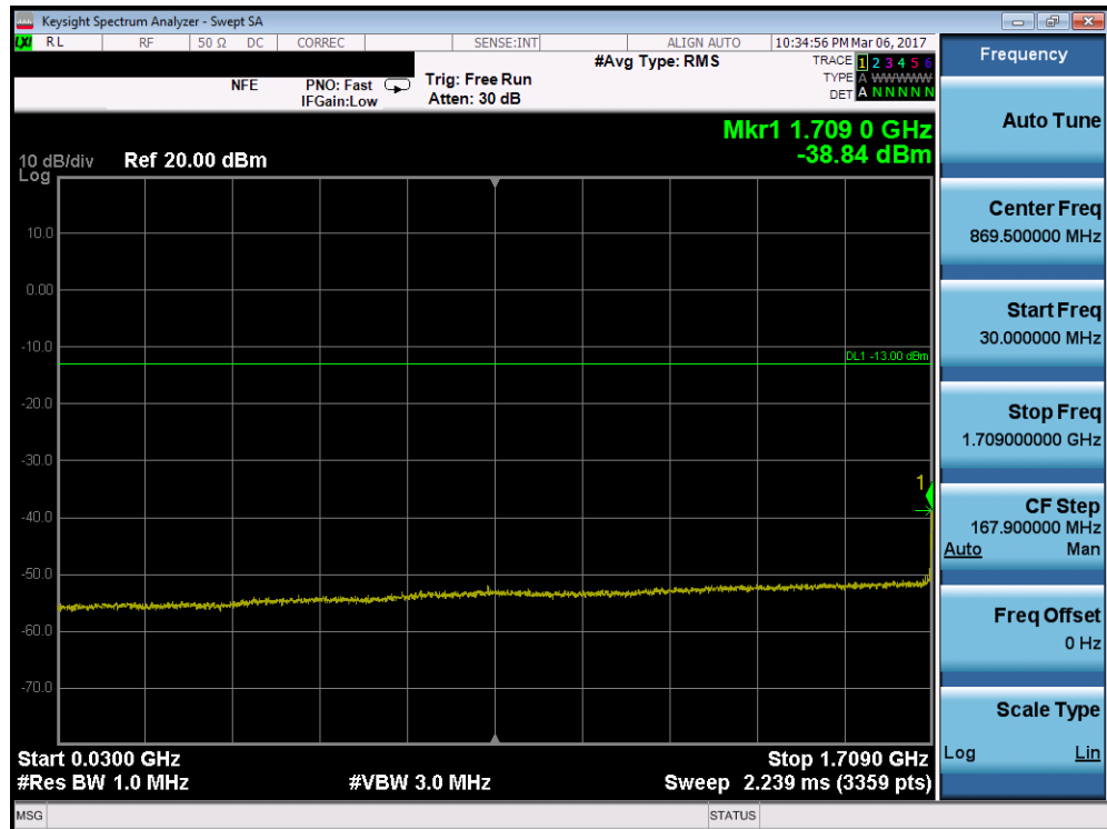
Plot 7-76. Conducted Spurious Plot (Band 66 – 5.0MHz QPSK – RB Size 1, RB Offset 0 – Low Channel)
