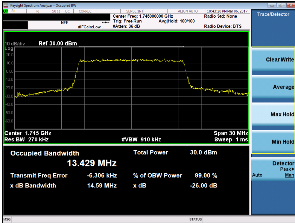
Plot 7-38. Occupied Bandwidth Plot (Band 66 – 15.0MHz 16-QAM – RB Size 75)
