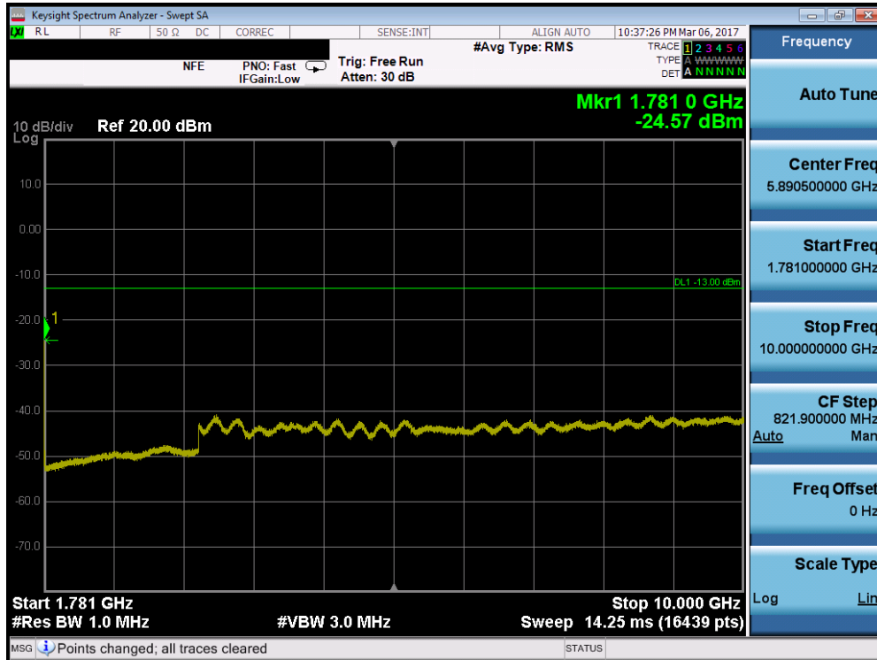
Plot 7-83. Conducted Spurious Plot (Band 66 – 5.0MHz QPSK – RB Size 1, RB Offset 0 – High Channel)
