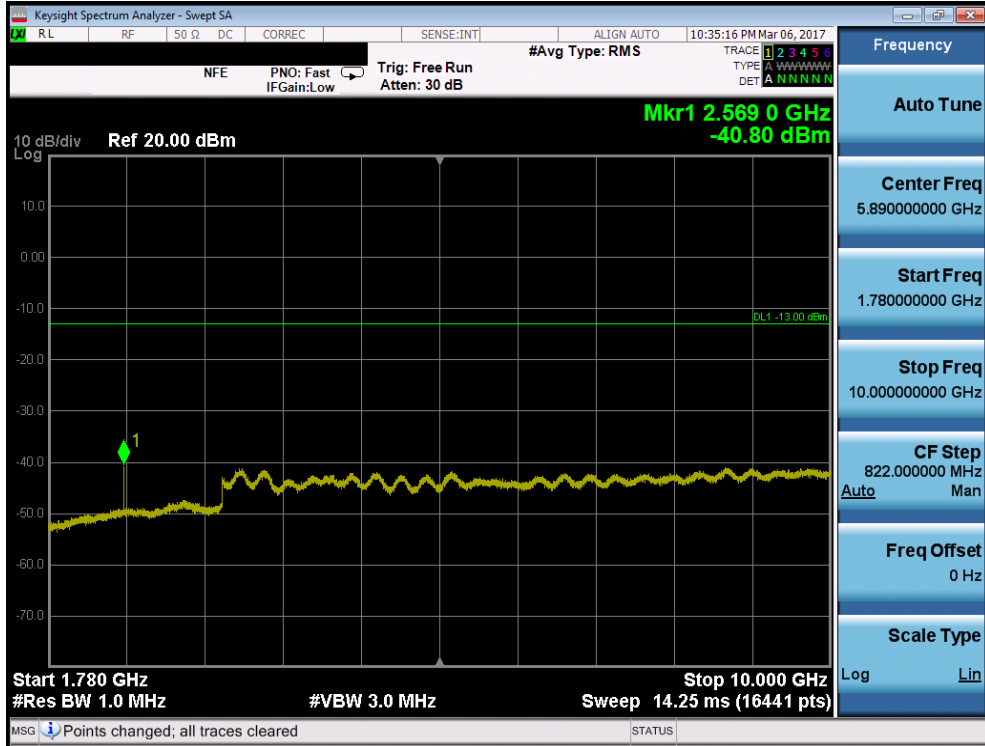
Plot 7-77. Conducted Spurious Plot (Band 66 – 5.0MHz QPSK – RB Size 1, RB Offset 0 – Low Channel)
