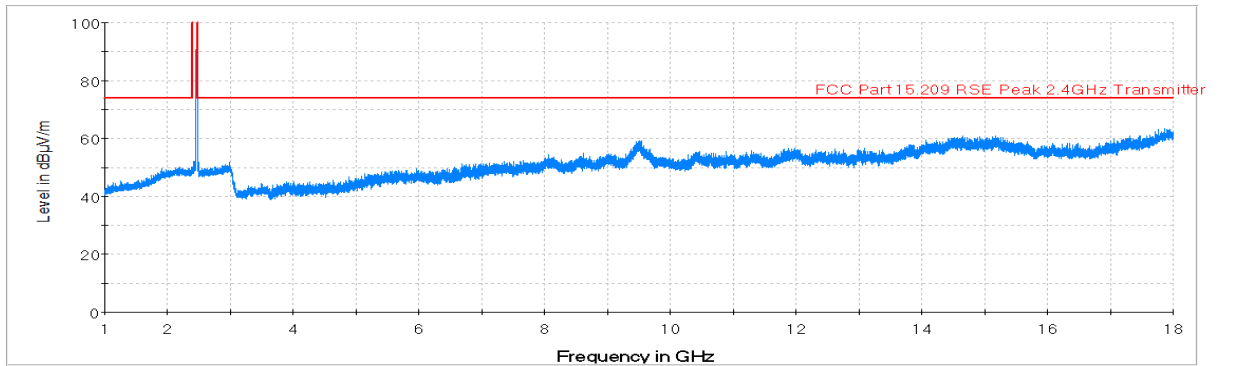
Plot 7-36. Radiated Spurious Plot above 1GHz (802.11b – Ch. 11, Ant. Pol. V)
