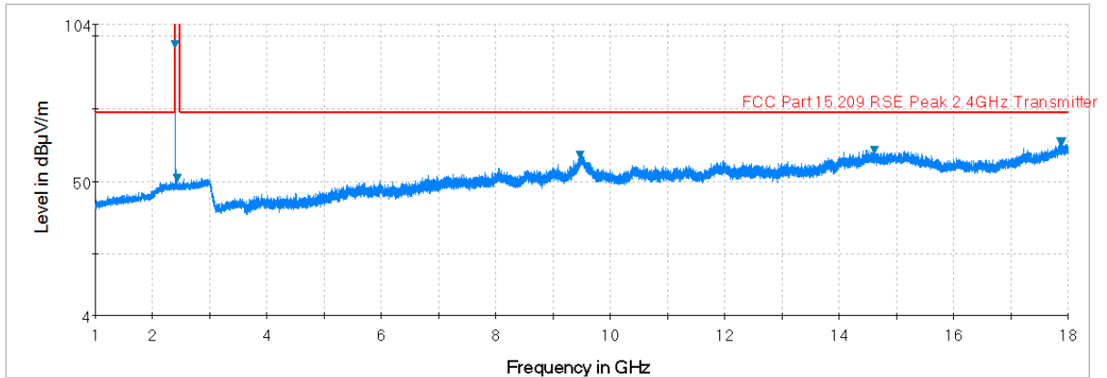
Plot 7-19. Radiated Spurious Plot above 1GHz (BT – Ch. 0, Ant. Pol. V)
