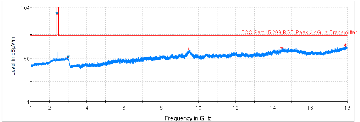
Plot 7-18. Radiated Spurious Plot above 1GHz (BT – Ch. 0, Ant. Pol. H)
