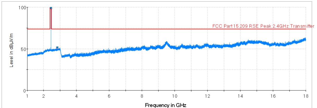
Plot 7-20. Radiated Spurious Plot above 1GHz (BT – Ch. 39, Ant. Pol. H)
