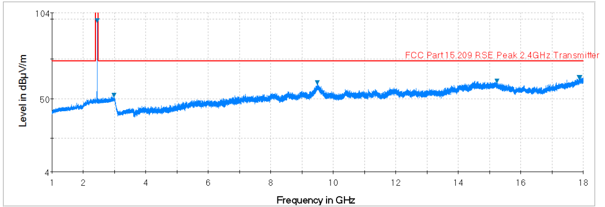
Plot 7-21. Radiated Spurious Plot above 1GHz (BT – Ch. 39, Ant. Pol. V)
