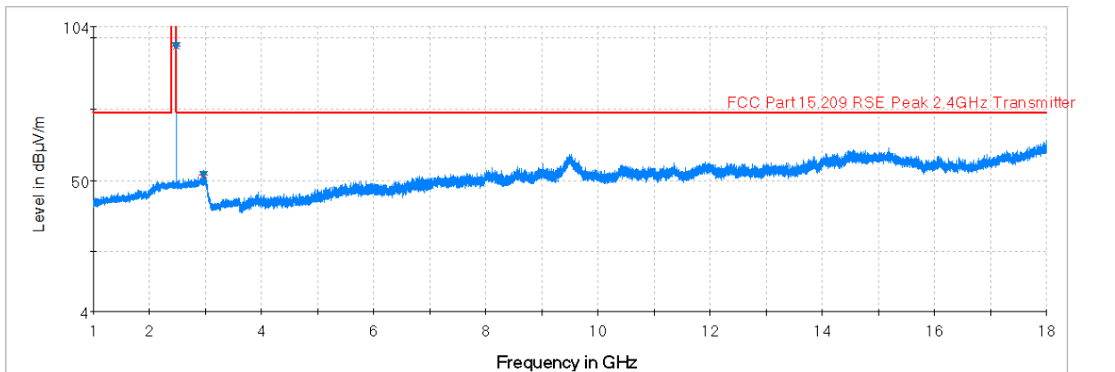
Plot 7-23. Radiated Spurious Plot above 1GHz (BT – Ch. 78, Ant. Pol. V)
