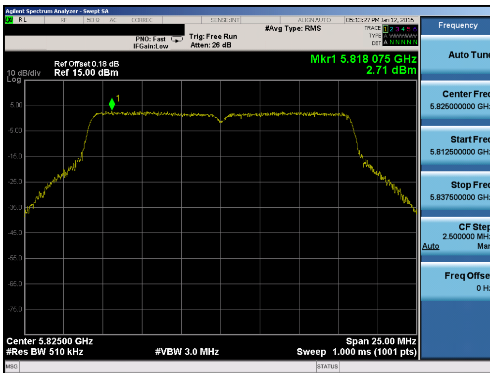
Plot 7-68. Power Spectral Density Plot (802.11a (UNII Band 3) – Ch. 165)
