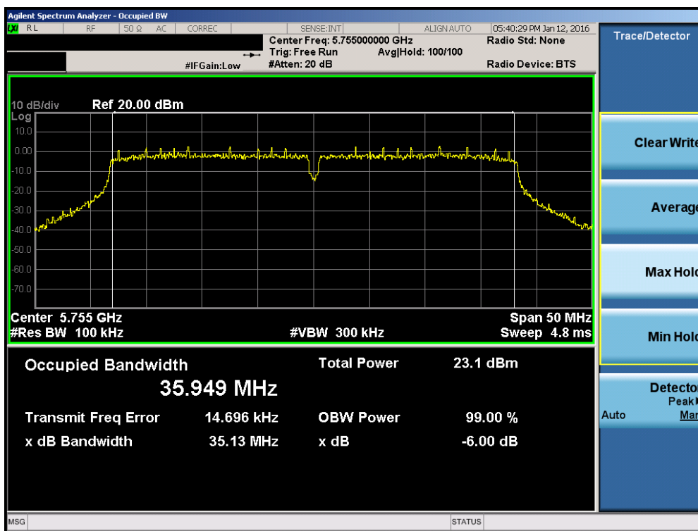
Plot 7-35. 6dB Bandwidth Plot (40MHz BW 802.11n (UNII Band 3) – Ch. 151)
