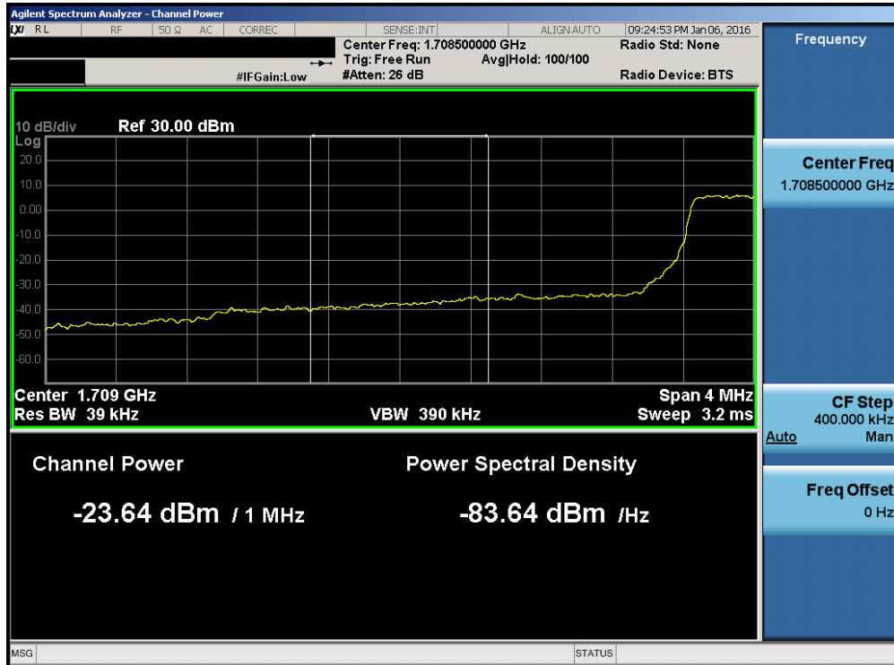
Plot 7-140. Lower Extended Band Edge Plot (Band 4 – 3.0MHz QPSK – RB Size 15)
