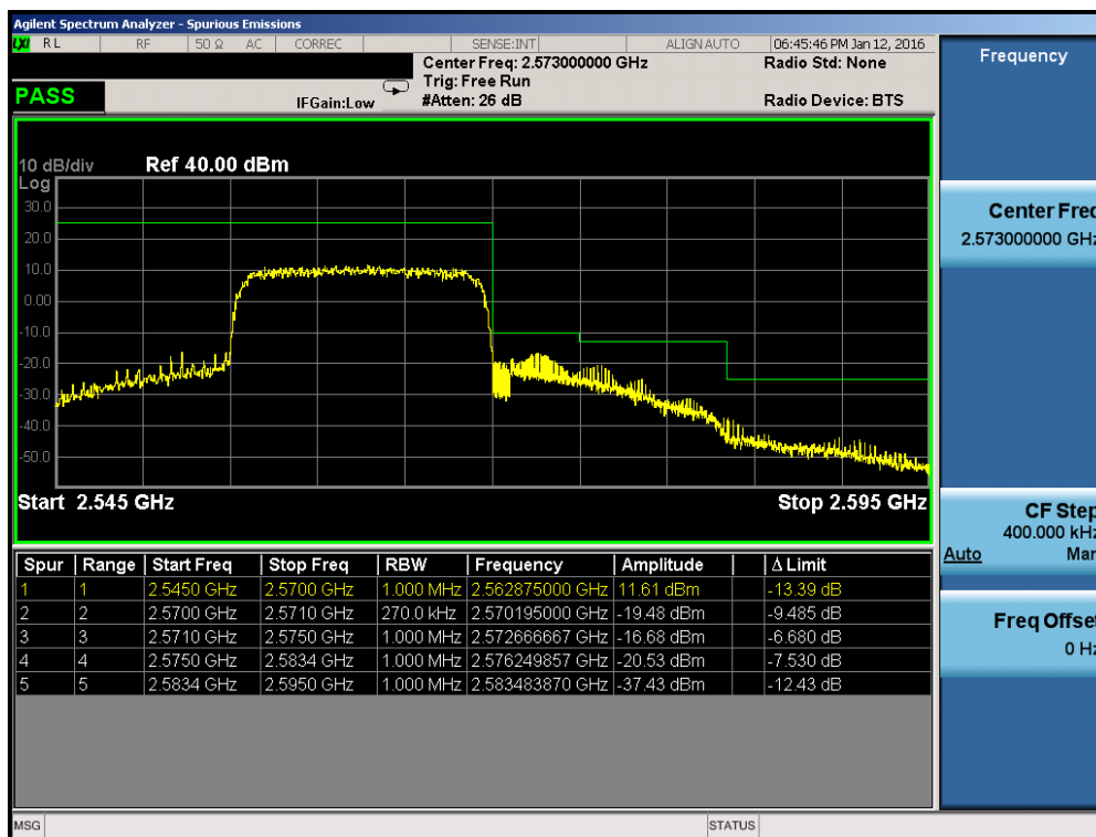
Plot 7-196. Upper ACP Plot (Band 7 – 15.0MHz QPSK – RB Size 75)
