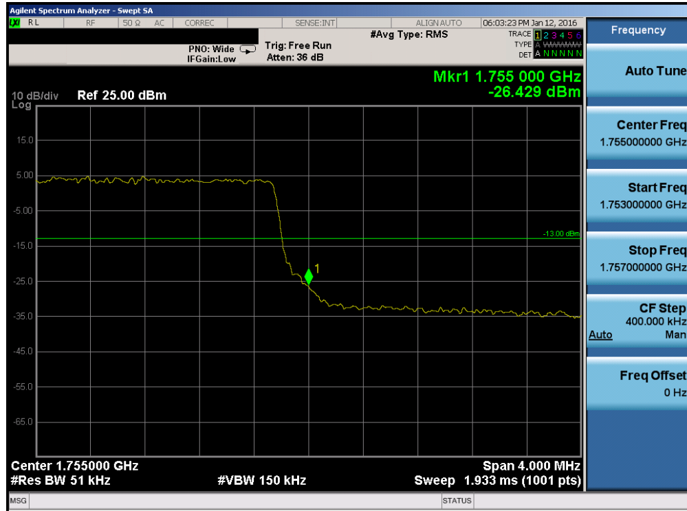
Plot 7-145. Upper Band Edge Plot (Band 4 – 5.0MHz QPSK – RB Size 25)
