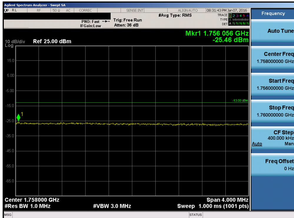
Plot 7-158. Upper Extended Band Edge Plot (Band 4 – 20.0MHz QPSK – RB Size 100)
