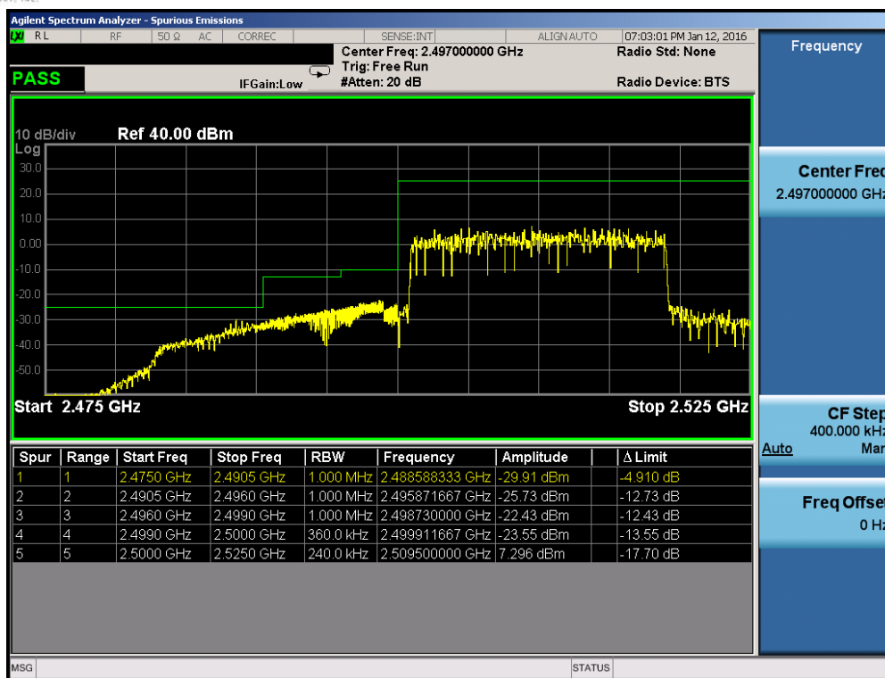
Plot 7-197. Lower ACP Plot (Band 7 – 20.0MHz QPSK – RB Size 100)
