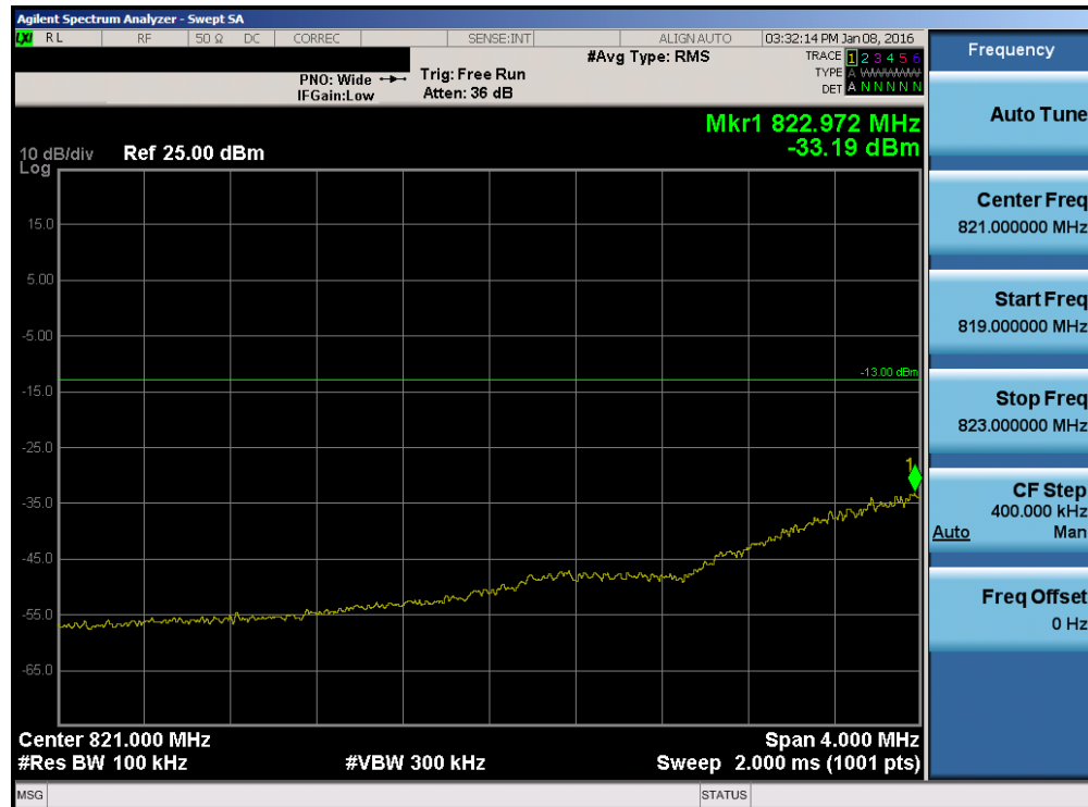
Plot 7-122. Lower Extended Band Edge Plot (Band 5 – 1.4MHz QPSK – RB Size 6)
