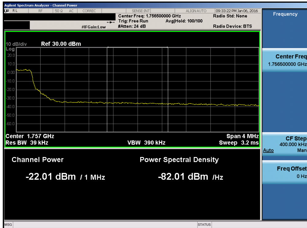
Plot 7-146. Upper Extended Band Edge Plot (Band 4 – 5.0MHz QPSK – RB Size 25)
