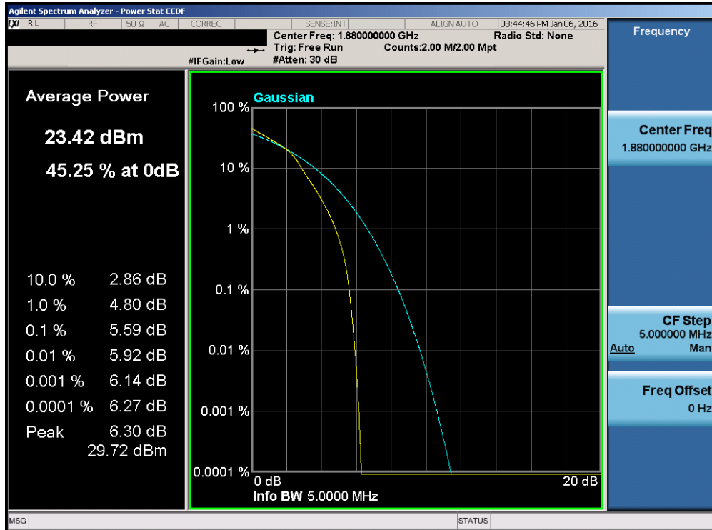
Plot 7-204. PAR Plot (Band 2 – 5.0MHz 16-QAM – RB Size 25)
