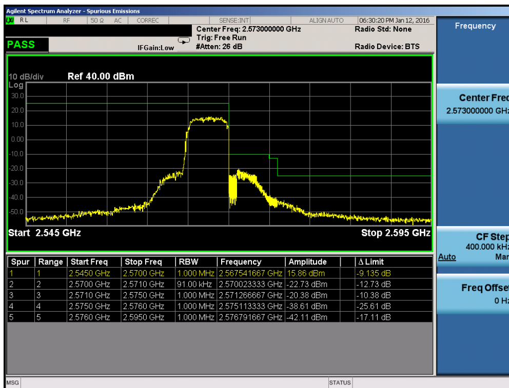
Plot 7-192. Upper ACP Plot (Band 7 – 5.0MHz QPSK – RB Size 25)
