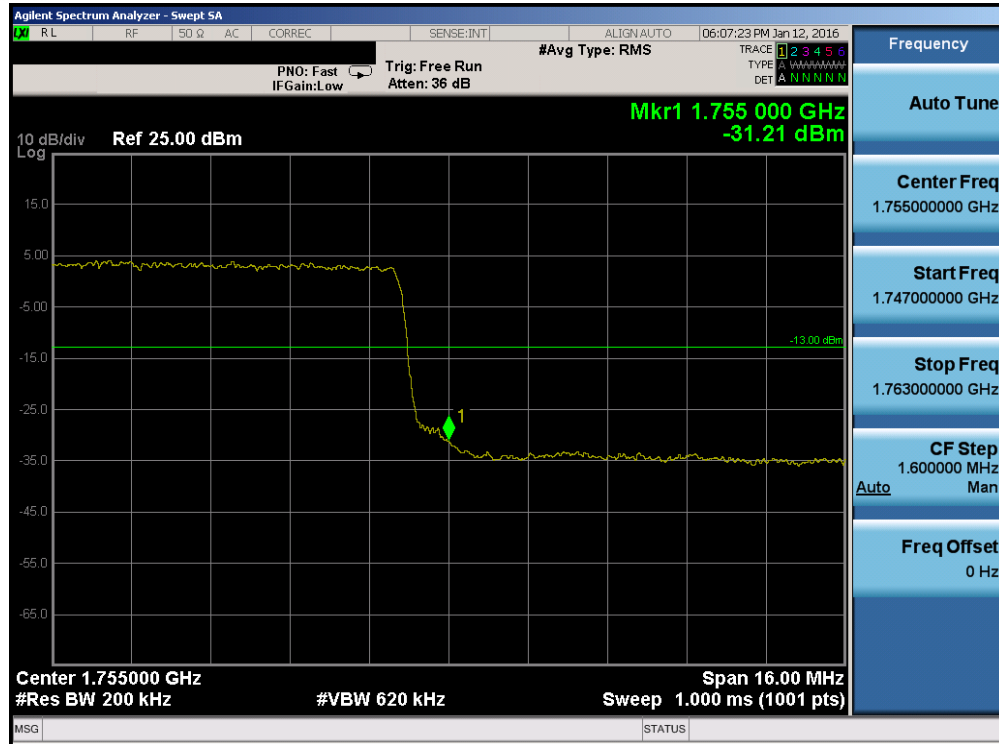
Plot 7-157. Upper Band Edge Plot (Band 4 – 20.0MHz QPSK – RB Size 100)
