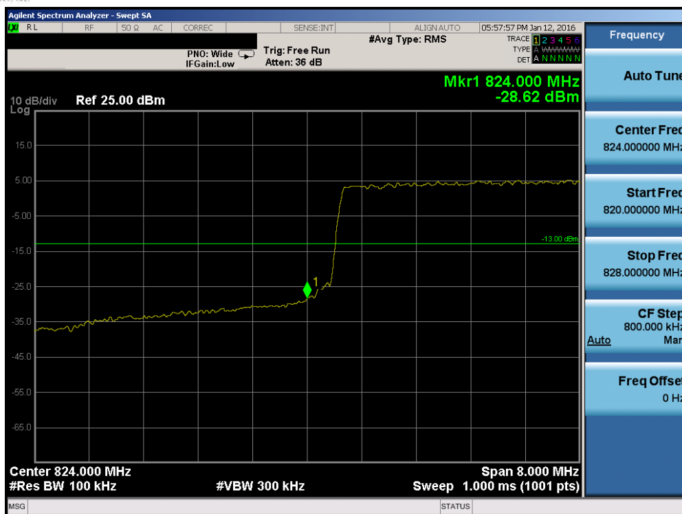
Plot 7-133. Lower Band Edge Plot (Band 5 – 10.0MHz QPSK – RB Size 50)
