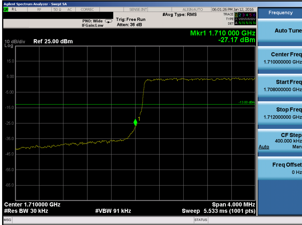
Plot 7-139. Lower Band Edge Plot (Band 4 – 3.0MHz QPSK – RB Size 15)
