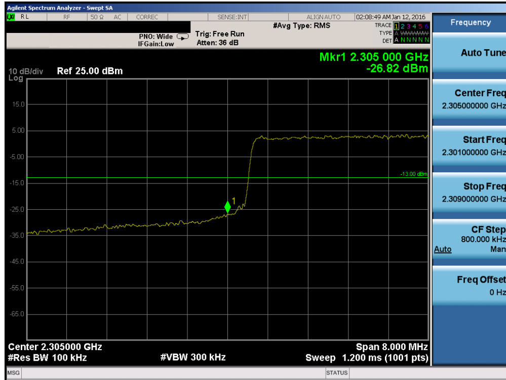
Plot 7-187. Lower Band Edge Plot (Band 30 – 10.0MHz QPSK – RB Size 50)
