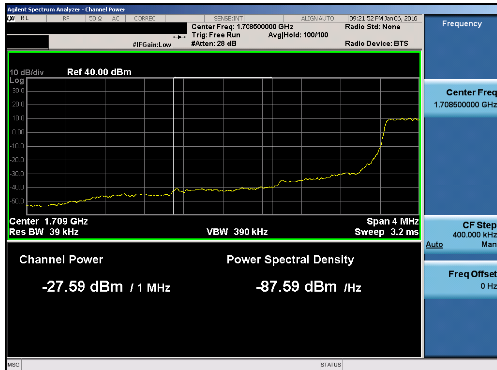
Plot 7-136. Lower Extended Band Edge Plot (Band 4 – 1.4MHz QPSK – RB Size 6)
