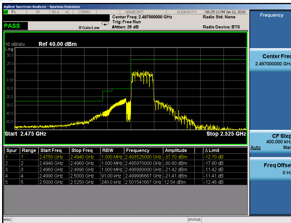
Plot 7-191. Lower ACP Plot (Band 7 – 5.0MHz QPSK – RB Size 25)
