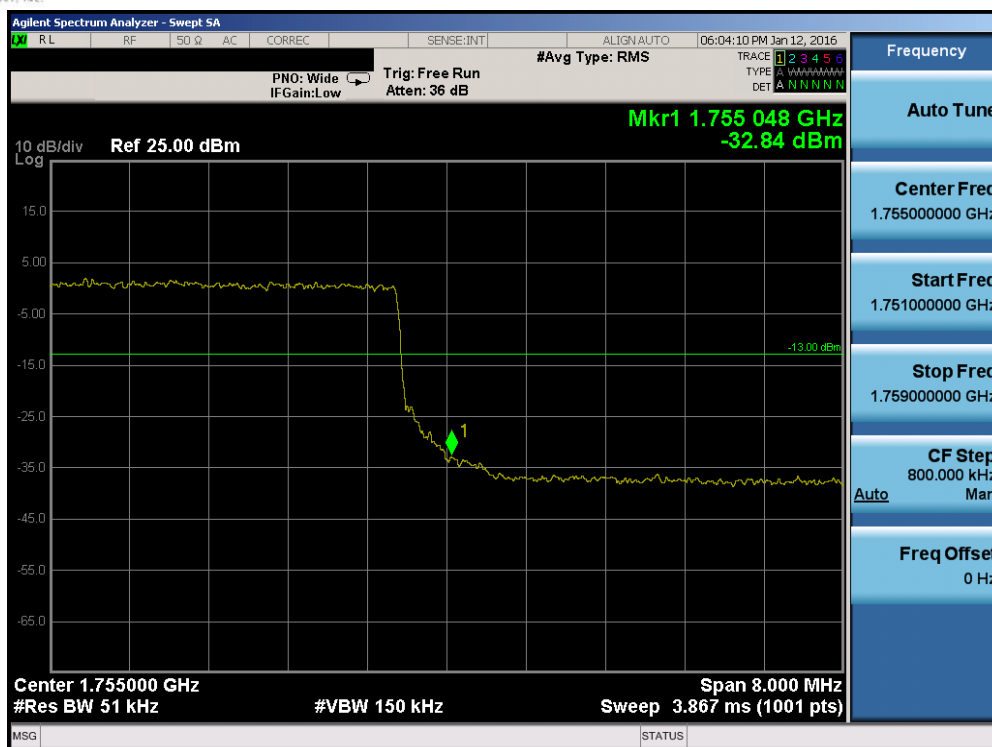
Plot 7-149. Upper Band Edge Plot (Band 4 – 10.0MHz QPSK – RB Size 50)
