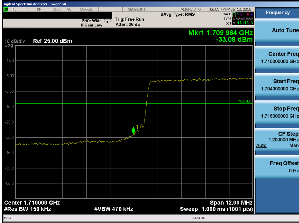
Plot 7-151. Lower Band Edge Plot (Band 4 – 15.0MHz QPSK – RB Size 75)
