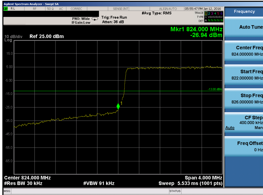
Plot 7-125. Lower Band Edge Plot (Band 5 – 3.0MHz QPSK – RB Size 15)
