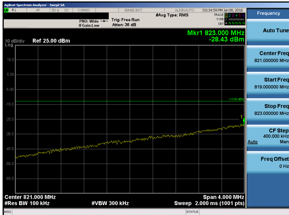
Plot 7-126. Lower Extended Band Edge Plot (Band 5 – 3.0MHz QPSK – RB Size 15)
