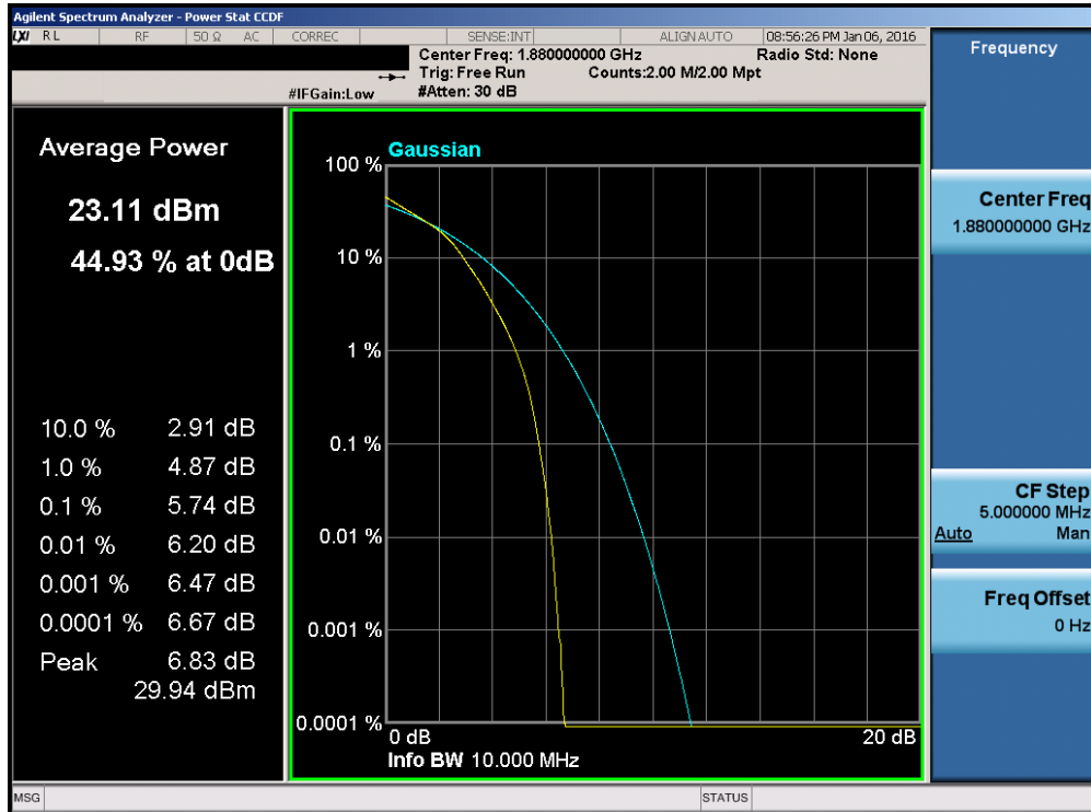
Plot 7-206. PAR Plot (Band 2 – 10.0MHz 16-QAM – RB Size 50)
