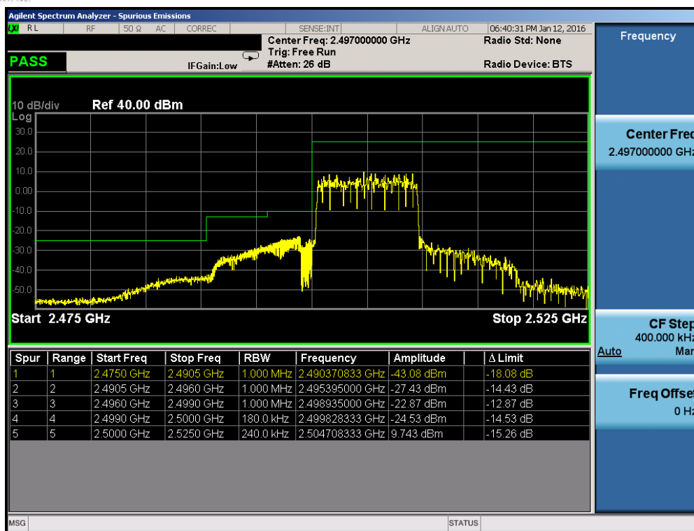
Plot 7-193. Lower ACP Plot (Band 7 – 10.0MHz QPSK – RB Size 50)
