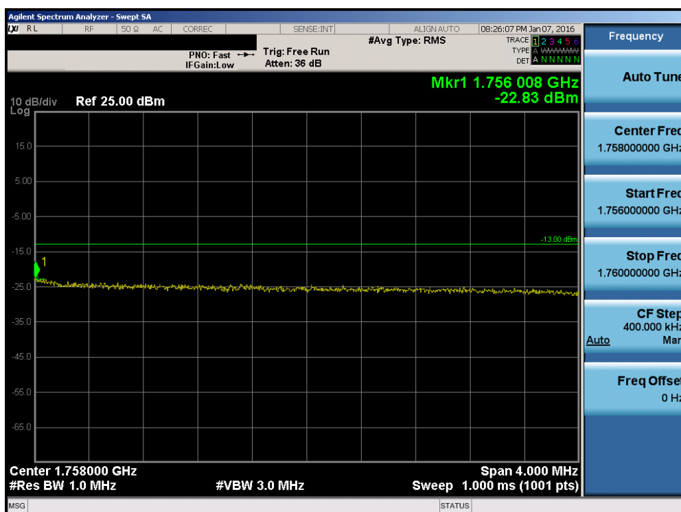
Plot 7-150. Upper Extended Band Edge Plot (Band 4 – 10.0MHz QPSK – RB Size 50)
