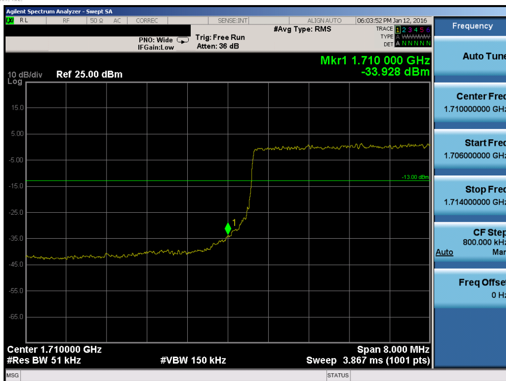
Plot 7-147. Lower Band Edge Plot (Band 4 – 10.0MHz QPSK – RB Size 50)
