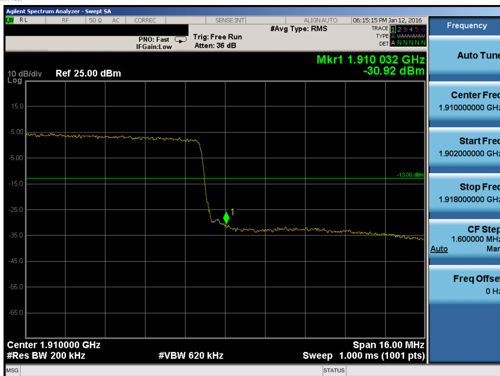
Plot 7-181. Upper Band Edge Plot (Band 2 – 20.0MHz QPSK – RB Size 100)
