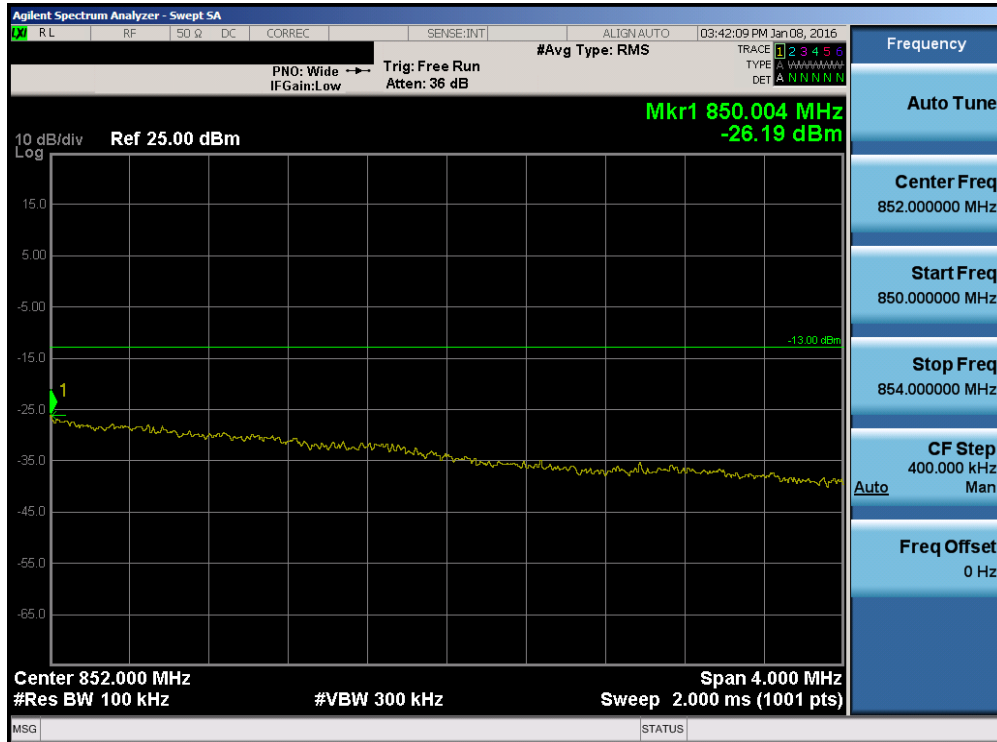
Plot 7-132. Upper Extended Band Edge Plot (Band 5 – 5.0MHz QPSK – RB Size 25)
