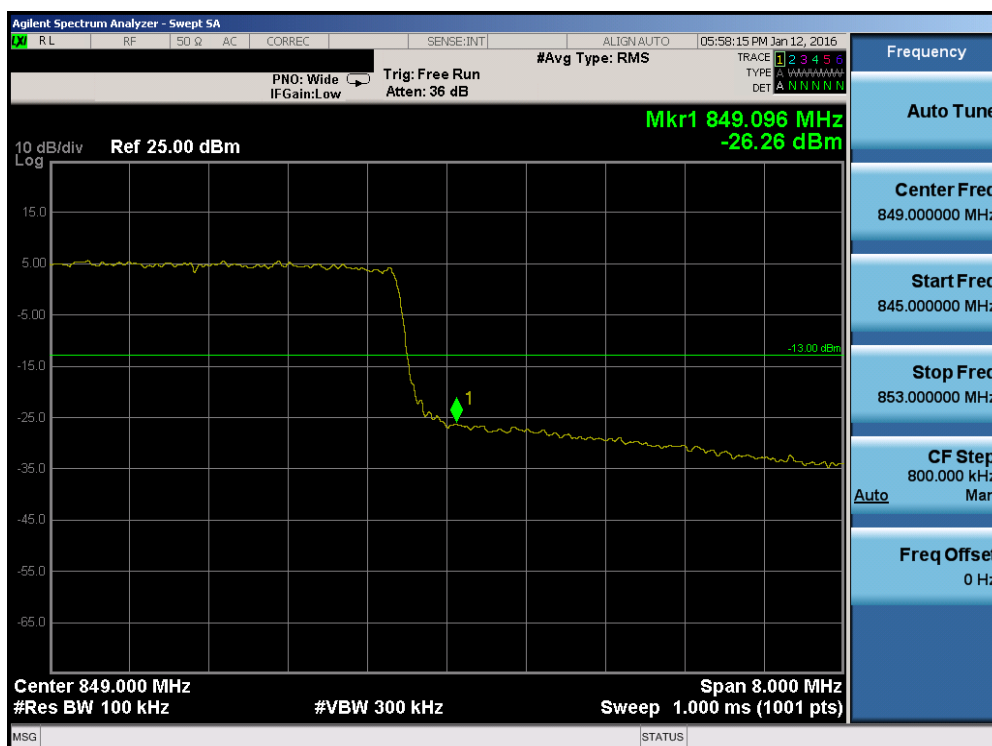
Plot 7-134. Upper Band Edge Plot (Band 5 – 10.0MHz QPSK – RB Size 50)
