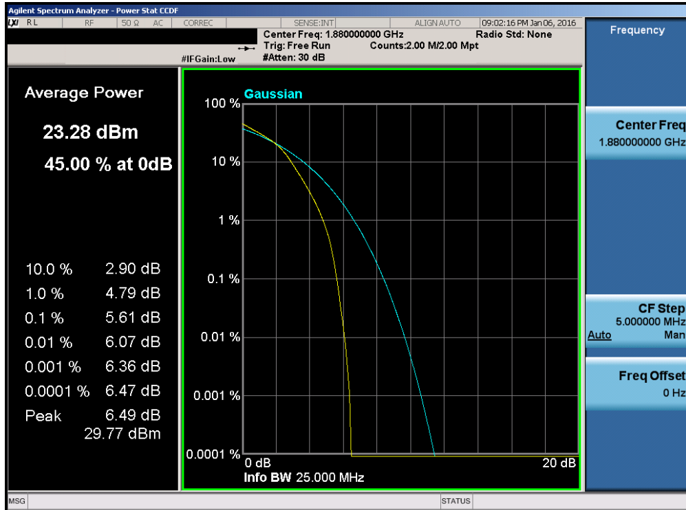
Plot 7-210. PAR Plot (Band 2 – 20.0MHz 16-QAM – RB Size 100)
