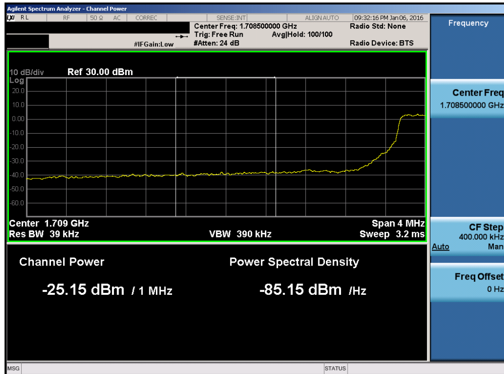
Plot 7-144. Lower Extended Band Edge Plot (Band 4 – 5.0MHz QPSK – RB Size 25)
