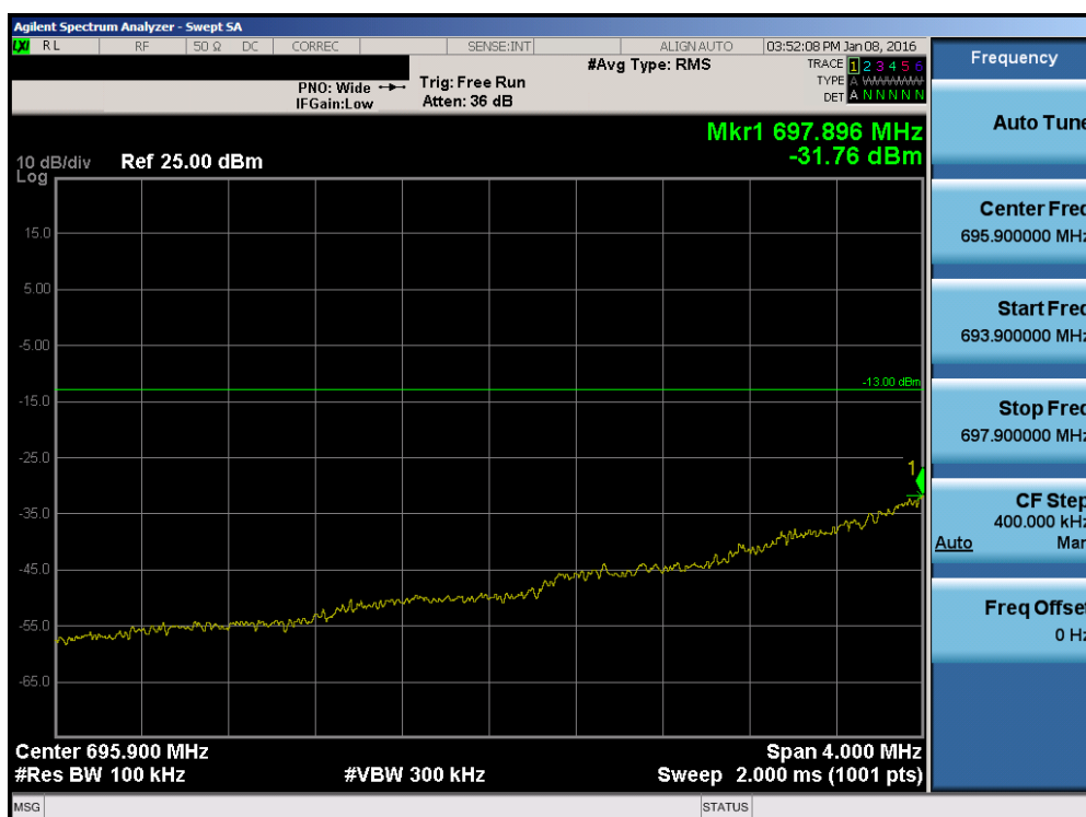
Plot 7-108. Lower Extended Band Edge Plot (Band 12 – 1.4MHz QPSK – RB Size 6)
