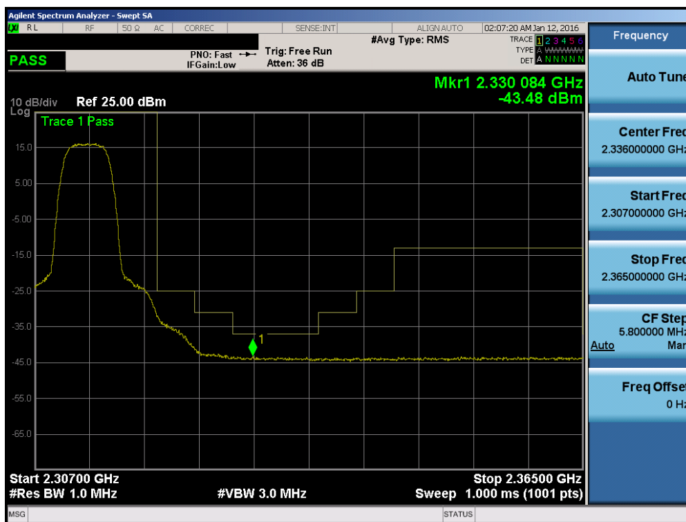
Plot 7-186. Upper Extended Band Edge Plot (Band 30 – 5.0MHz QPSK – RB Size 25)
