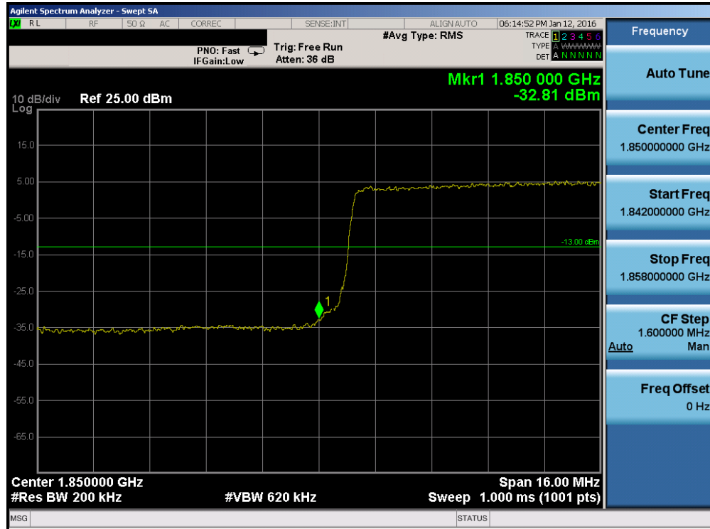
Plot 7-179. Lower Band Edge Plot (Band 2 – 20.0MHz QPSK – RB Size 100)
