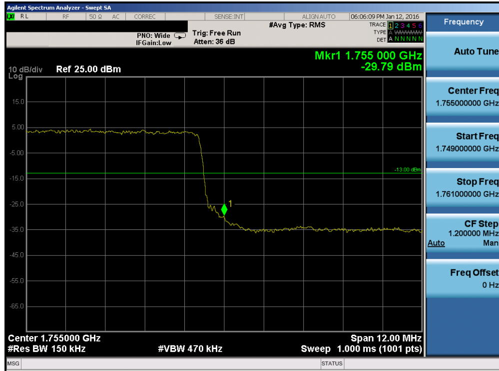
Plot 7-153. Upper Band Edge Plot (Band 4 – 15.0MHz QPSK – RB Size 75)
