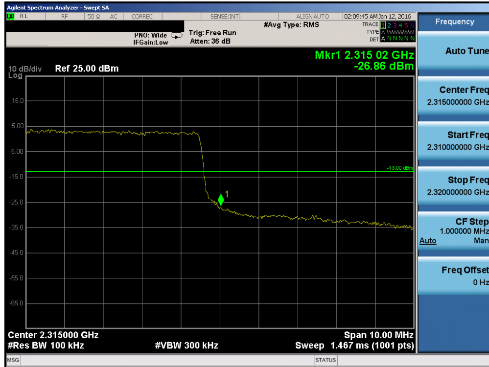
Plot 7-189. Upper Band Edge Plot (Band 30 – 10.0MHz QPSK – RB Size 50)
