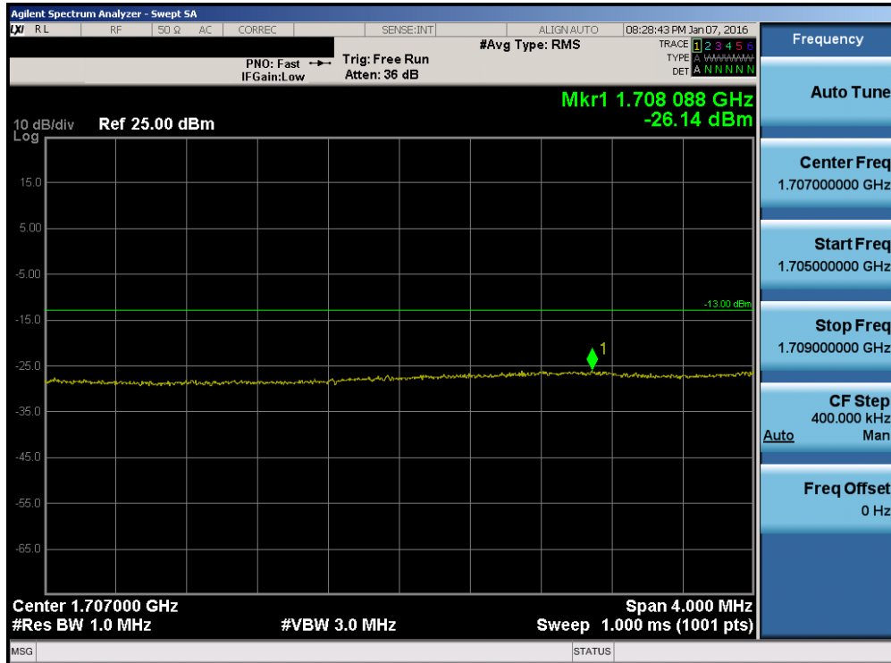
Plot 7-152. Lower Extended Band Edge Plot (Band 4 – 15.0MHz QPSK – RB Size 75)
