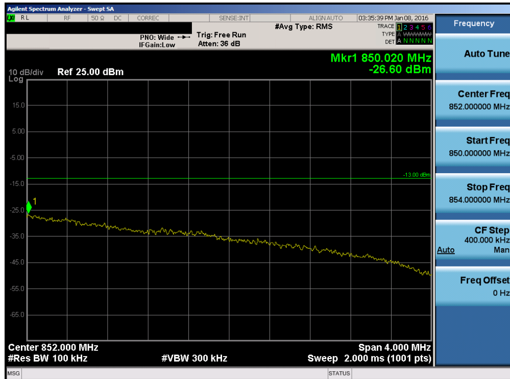
Plot 7-128. Upper Extended Band Edge Plot (Band 5 - Band 5 - 3.0MHz QPSK - RB Size 15)
