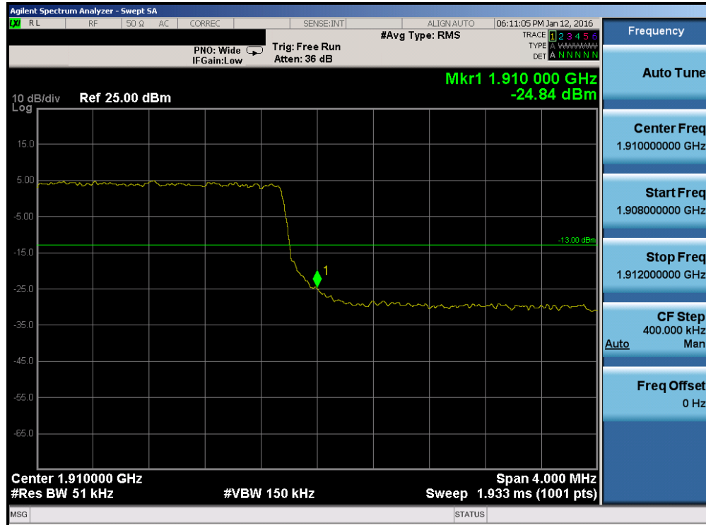
Plot 7-169. Upper Band Edge Plot (Band 2 – 5.0MHz QPSK – RB Size 25)
