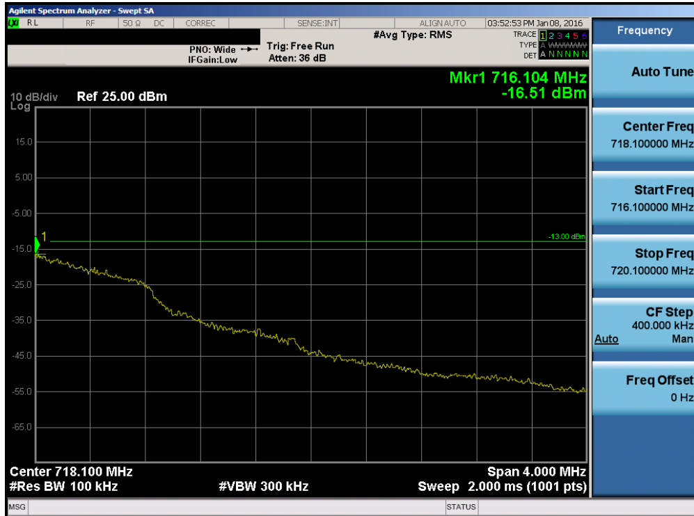
Plot 7-110. Upper Extended Band Edge Plot (Band 12 – 1.4MHz QPSK – RB Size 6)
