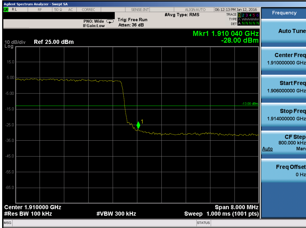
Plot 7-173. Upper Band Edge Plot (Band 2 – 10.0MHz QPSK – RB Size 50)
