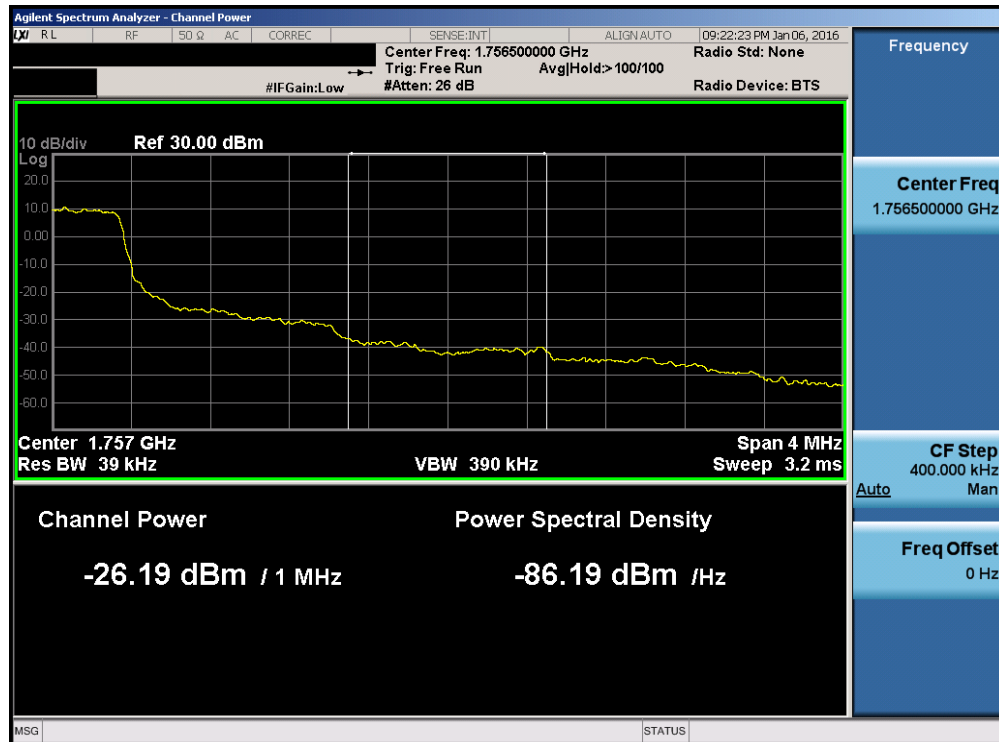
Plot 7-138. Upper Extended Band Edge Plot (Band 4 – 1.4MHz QPSK – RB Size 6)
