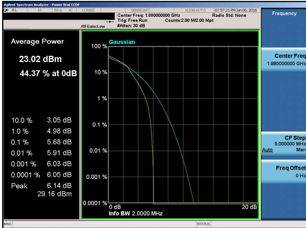
Plot 7-200. PAR Plot (Band 2 – 1.4MHz 16-QAM – RB Size 6)
