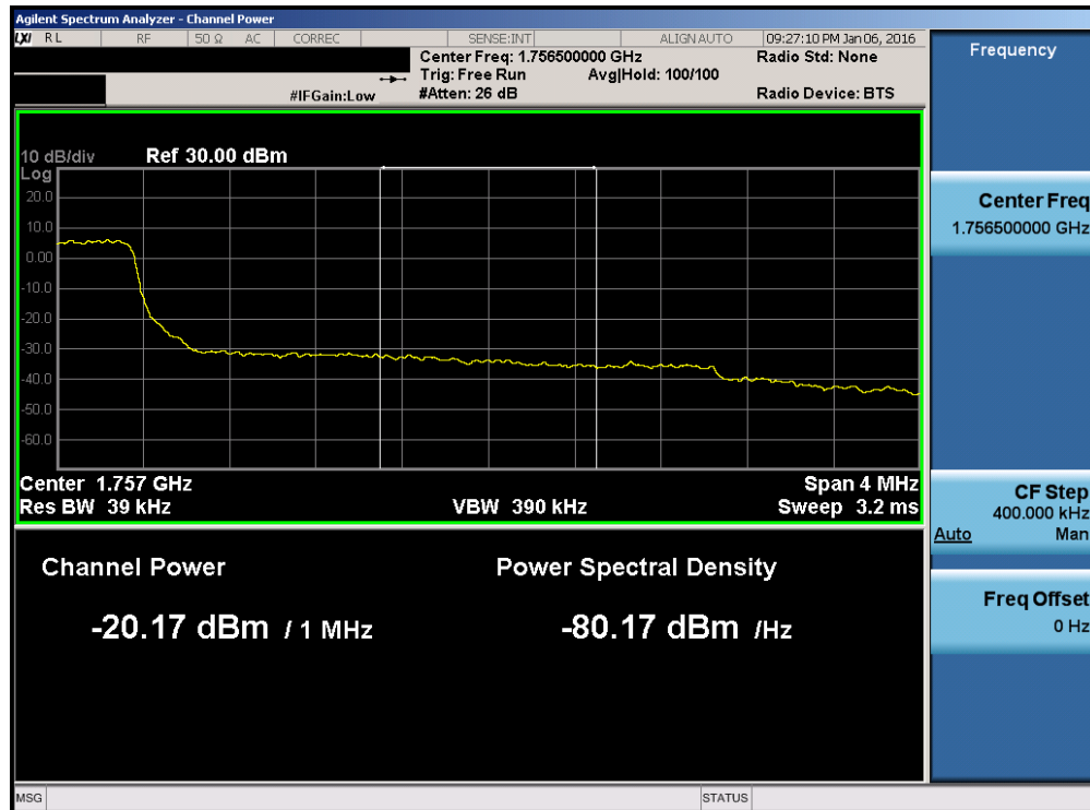
Plot 7-142. Upper Extended Band Edge Plot (Band 4 – 3.0MHz QPSK – RB Size 15)
