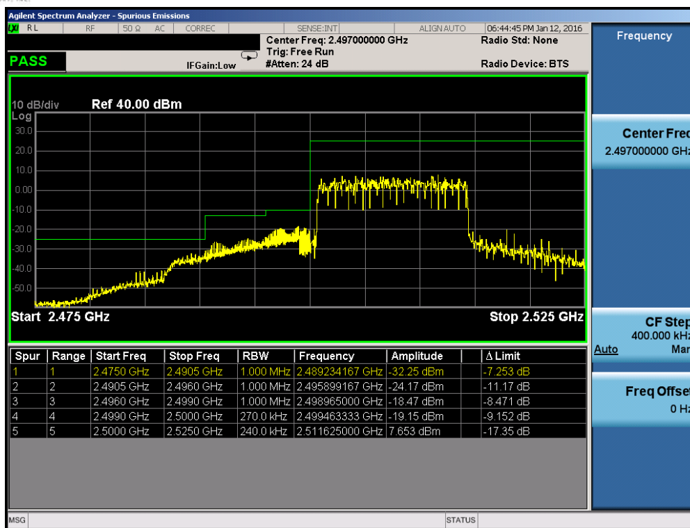
Plot 7-195. Lower ACP Plot (Band 7 – 15.0MHz QPSK – RB Size 75)
