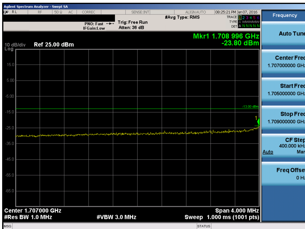
Plot 7-148. Lower Extended Band Edge Plot (Band 4 – 10.0MHz QPSK – RB Size 50)
