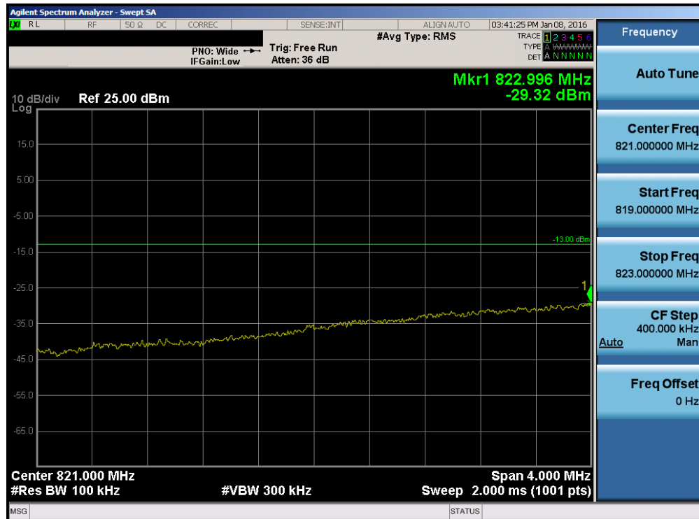
Plot 7-130. Lower Extended Band Edge Plot (Band 5 – 5.0MHz QPSK – RB Size 25)
