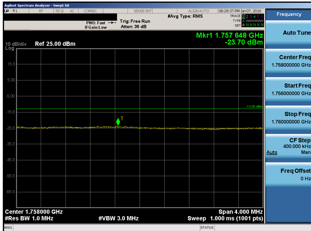
Plot 7-154. Upper Extended Band Edge Plot (Band 4 – 15.0MHz QPSK – RB Size 75)
