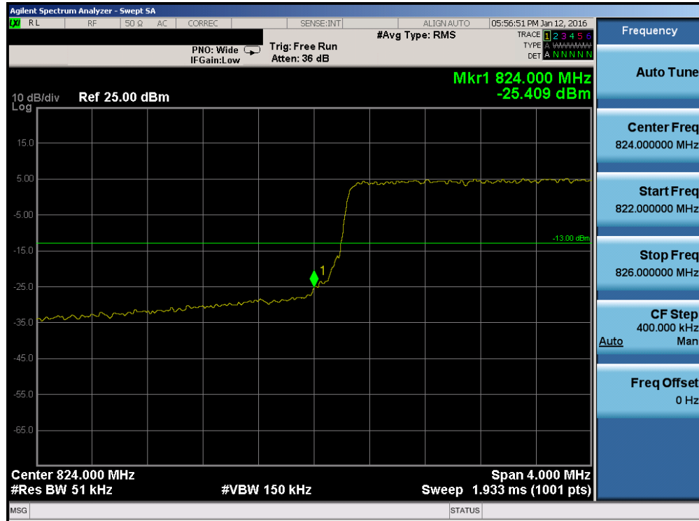
Plot 7-129. Lower Band Edge Plot (Band 5 – 5.0MHz QPSK – RB Size 25)
