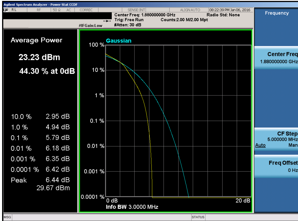
Plot 7-202. PAR Plot (Band 2 – 3.0MHz 16-QAM – RB Size 15)
