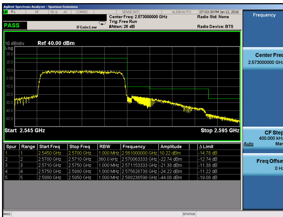
Plot 7-198. Upper ACP Plot (Band 7 – 20.0MHz QPSK – RB Size 100)
