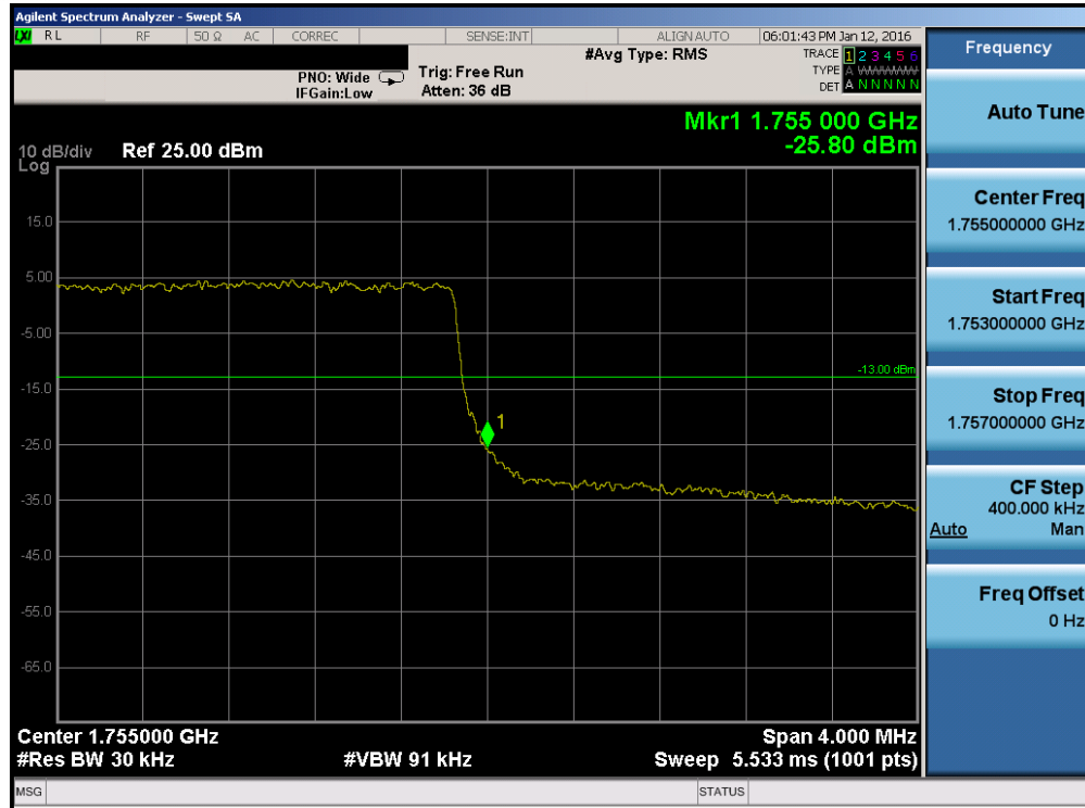
Plot 7-141. Upper Band Edge Plot (Band 4 – 3.0MHz QPSK – RB Size 15)
