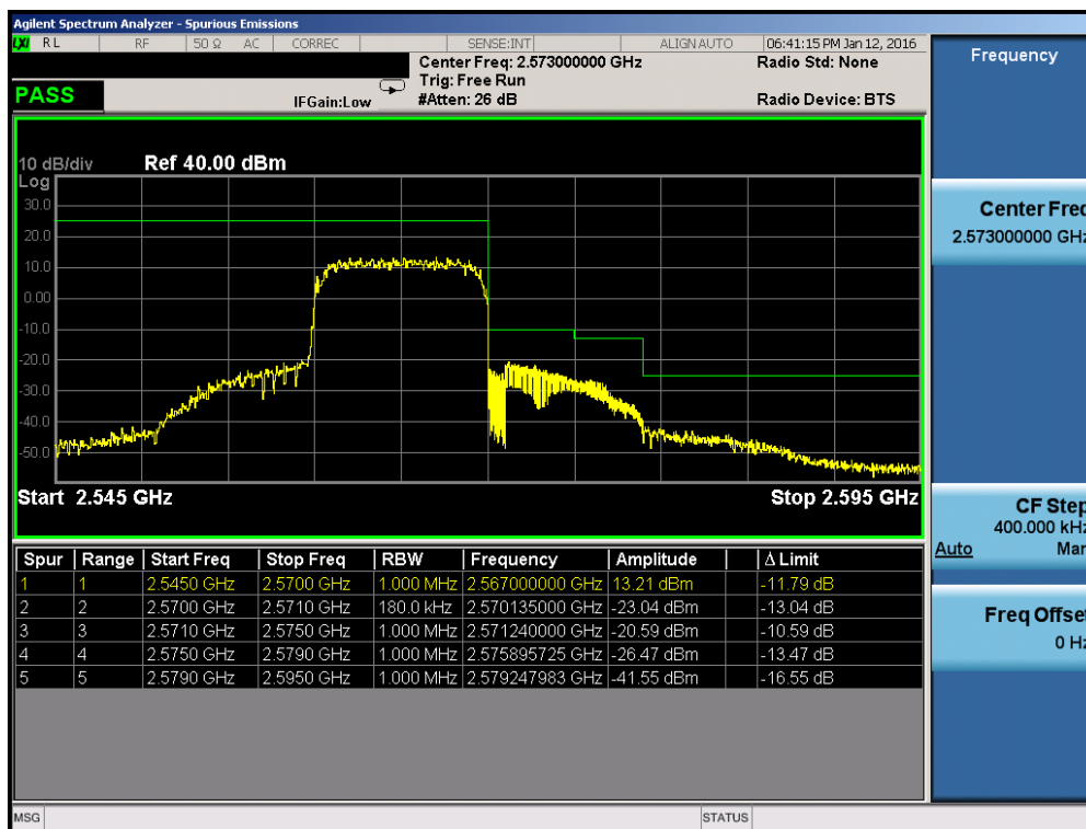
Plot 7-194. Upper ACP Plot (Band 7 – 10.0MHz QPSK – RB Size 50)
