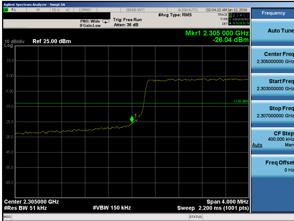
Plot 7-183. Lower Band Edge Plot (Band 30 – 5.0MHz QPSK – RB Size 25)
