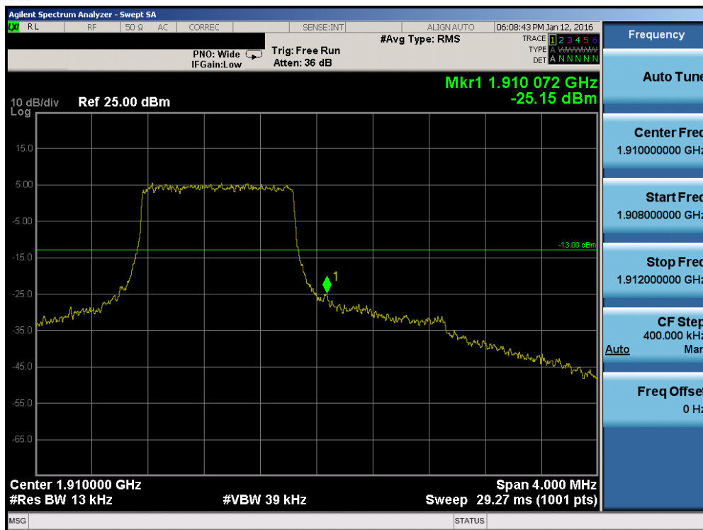
Plot 7-161. Upper Band Edge Plot (Band 2 – 1.4MHz QPSK – RB Size 6)
