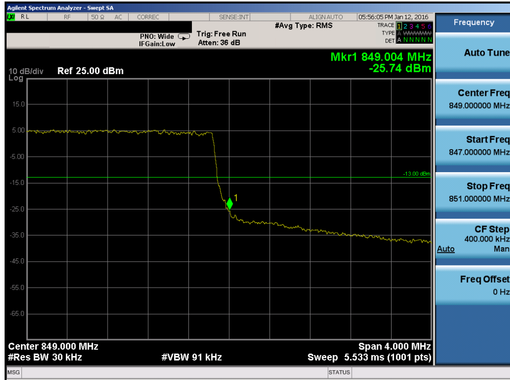
Plot 7-127. Upper Band Edge Plot (Band 5 - 3.0MHz QPSK - RB Size 15)
