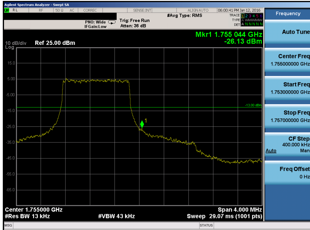
Plot 7-137. Upper Band Edge Plot (Band 4 – 1.4MHz QPSK – RB Size 6)
