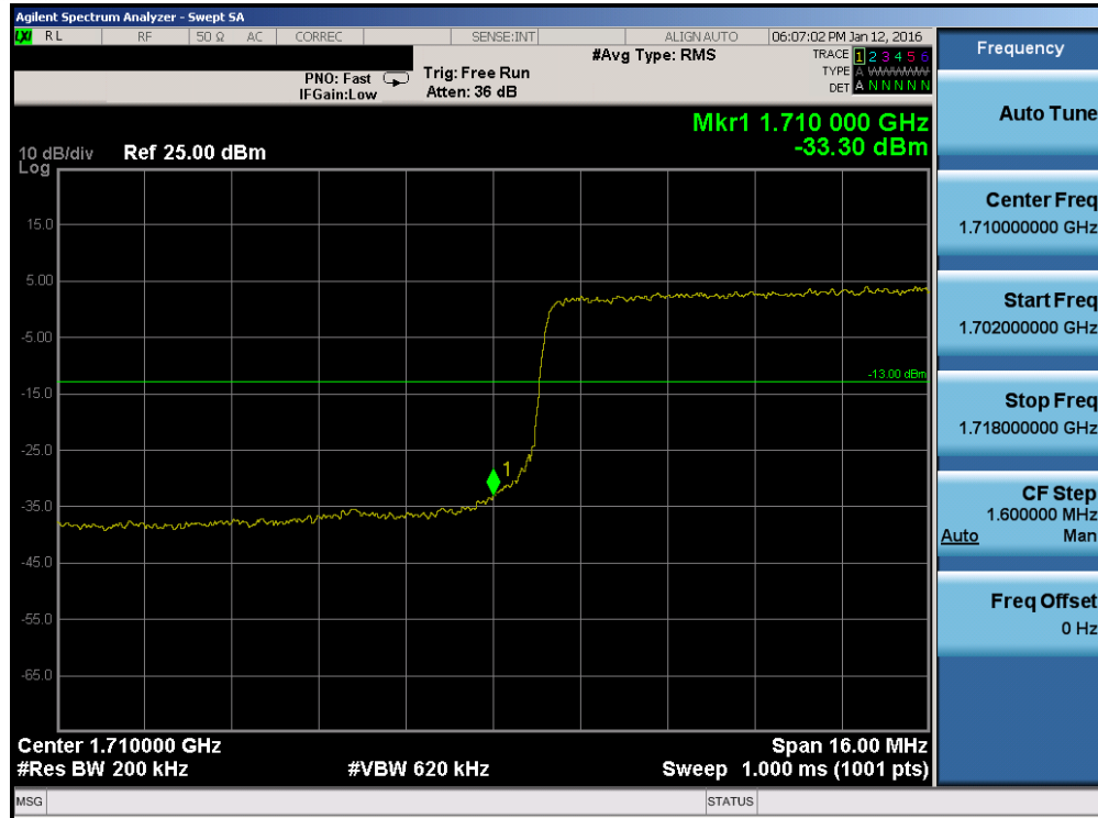
Plot 7-155. Lower Band Edge Plot (Band 4 – 20.0MHz QPSK – RB Size 100)
