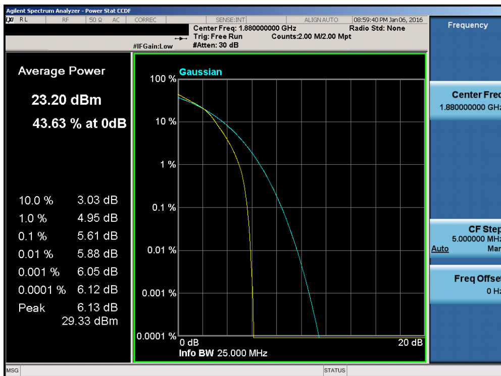
Plot 7-208. PAR Plot (Band 2 – 15.0MHz 16-QAM – RB Size 75)
