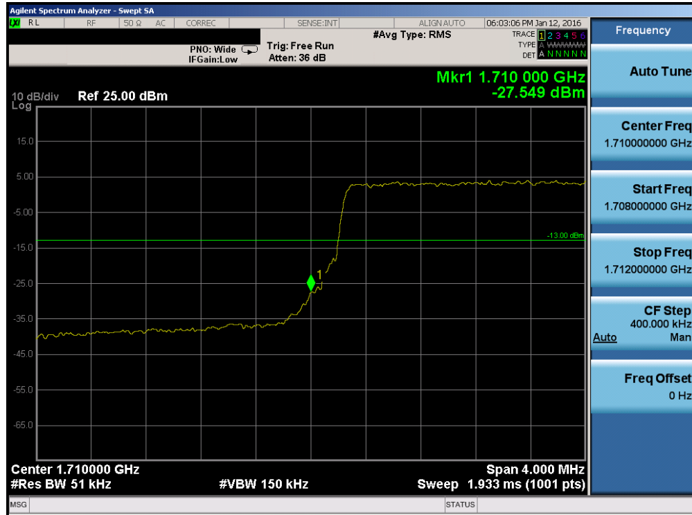
Plot 7-143. Lower Band Edge Plot (Band 4 – 5.0MHz QPSK – RB Size 25)
