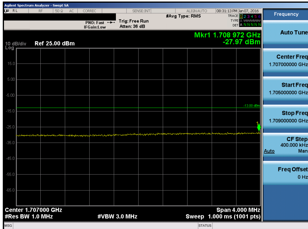
Plot 7-156. Lower Extended Band Edge Plot (Band 4 – 20.0MHz QPSK – RB Size 100)
