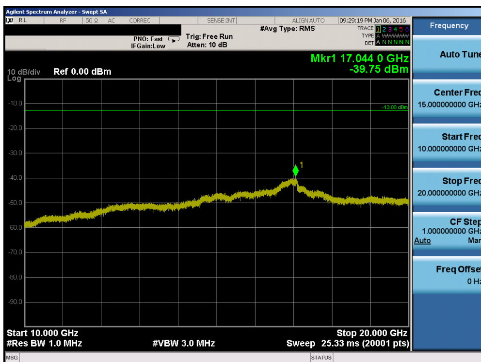
Plot 7-76. Conducted Spurious Plot (Band 4 – 5.0MHz QPSK – RB Size 1, RB Offset 0 – Mid Channel)
