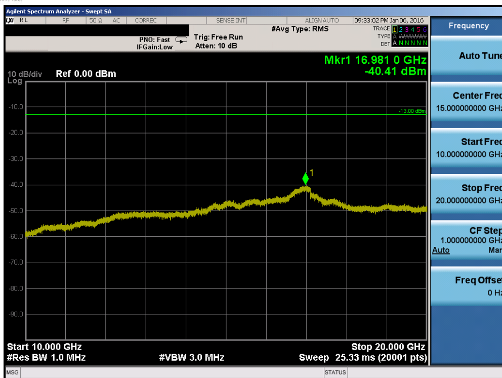
Plot 7-79. Conducted Spurious Plot (Band 4 – 5.0MHz QPSK – RB Size 1, RB Offset 0 – High Channel)
