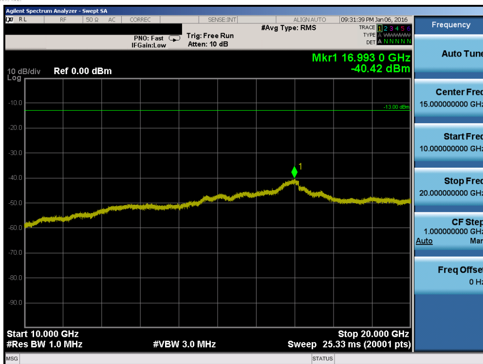
Plot 7-73. Conducted Spurious Plot (Band 4 – 5.0MHz QPSK – RB Size 1, RB Offset 0 – Low Channel)
