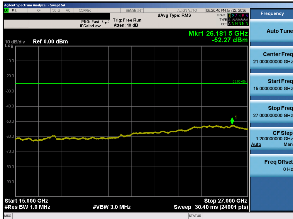
Plot 7-106. Conducted Spurious Plot (Band 7 – 5.0MHz QPSK – RB Size 1, RB Offset 0 – High Channel)
