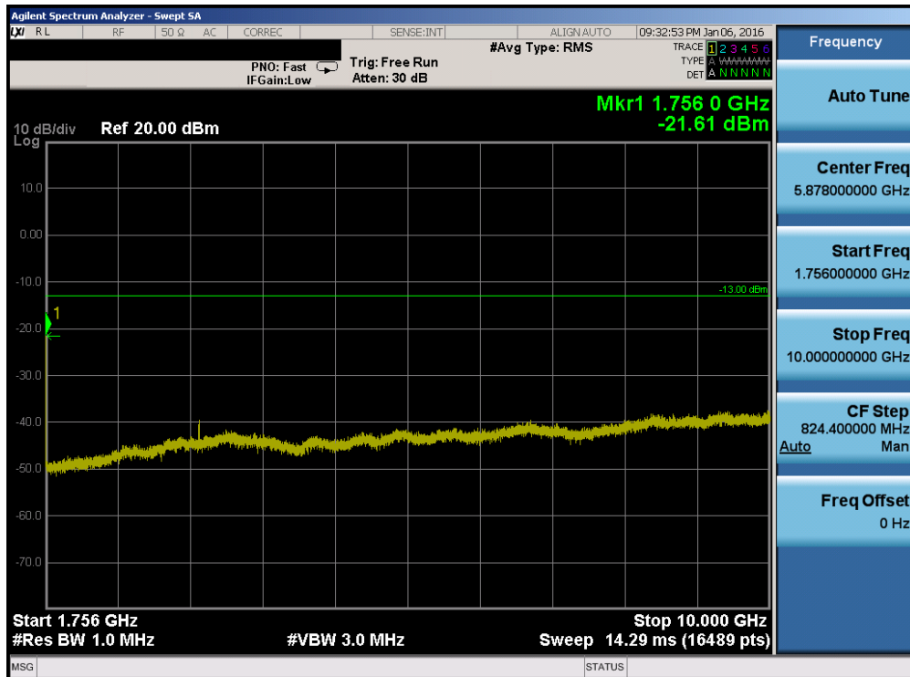
Plot 7-78. Conducted Spurious Plot (Band 4 – 5.0MHz QPSK – RB Size 1, RB Offset 0 – High Channel)
