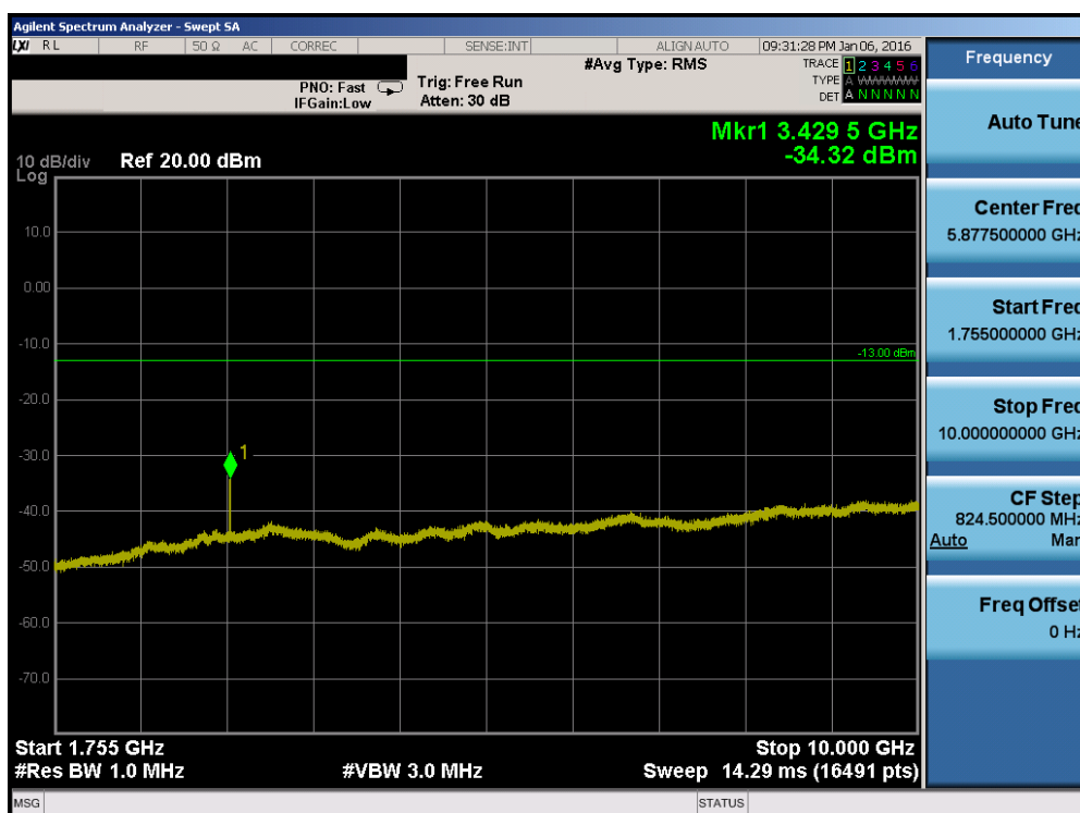
Plot 7-72. Conducted Spurious Plot (Band 4 – 5.0MHz QPSK – RB Size 1, RB Offset 0 – Low Channel)
