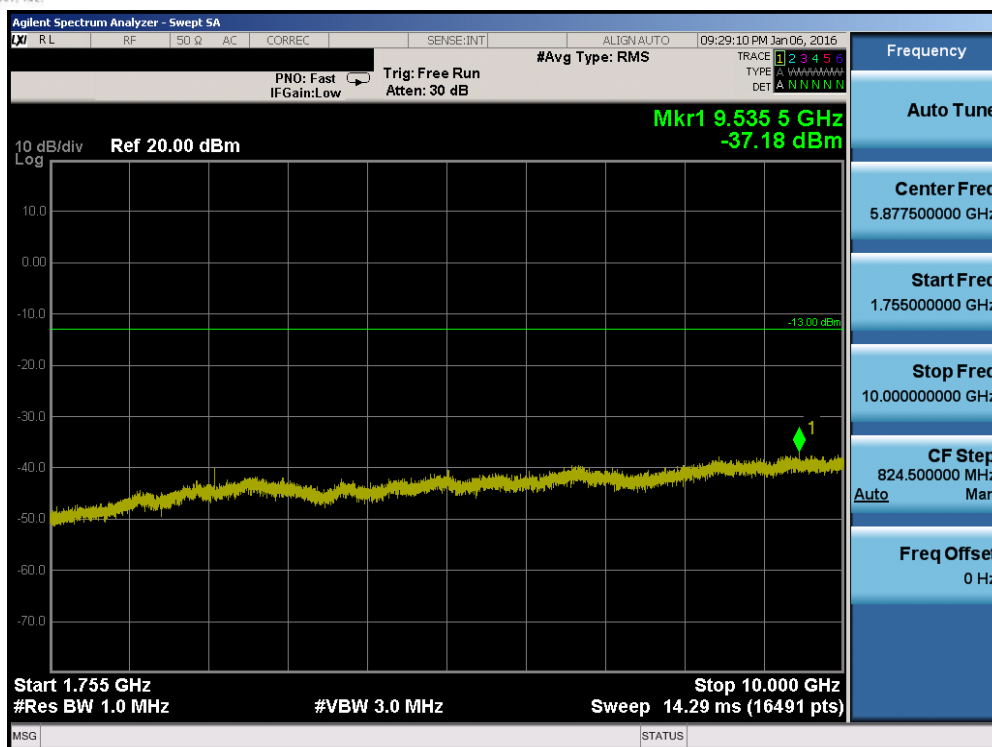
Plot 7-75. Conducted Spurious Plot (Band 4 – 5.0MHz QPSK – RB Size 1, RB Offset 0 – Mid Channel)
