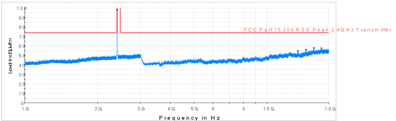
Plot 6-35. Radiated Spurious Plot above 1GHz (802.11b – Ch. 11, Ant. Pol. H)
