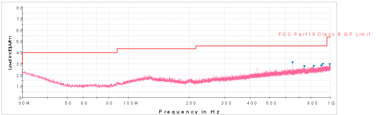
Plot 6-44. Radiated Spurious Plot below 1GHz (Pol. V)
