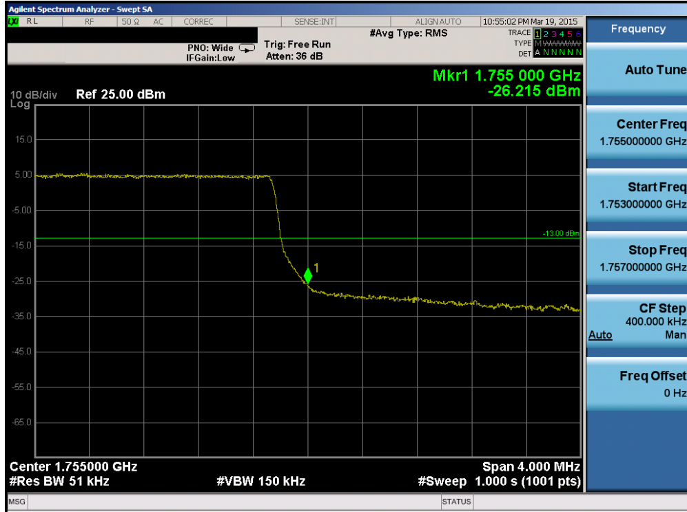
Plot 6-86. Upper Band Edge Plot (Band 4 – 5.0MHz QPSK – RB Size 25)
