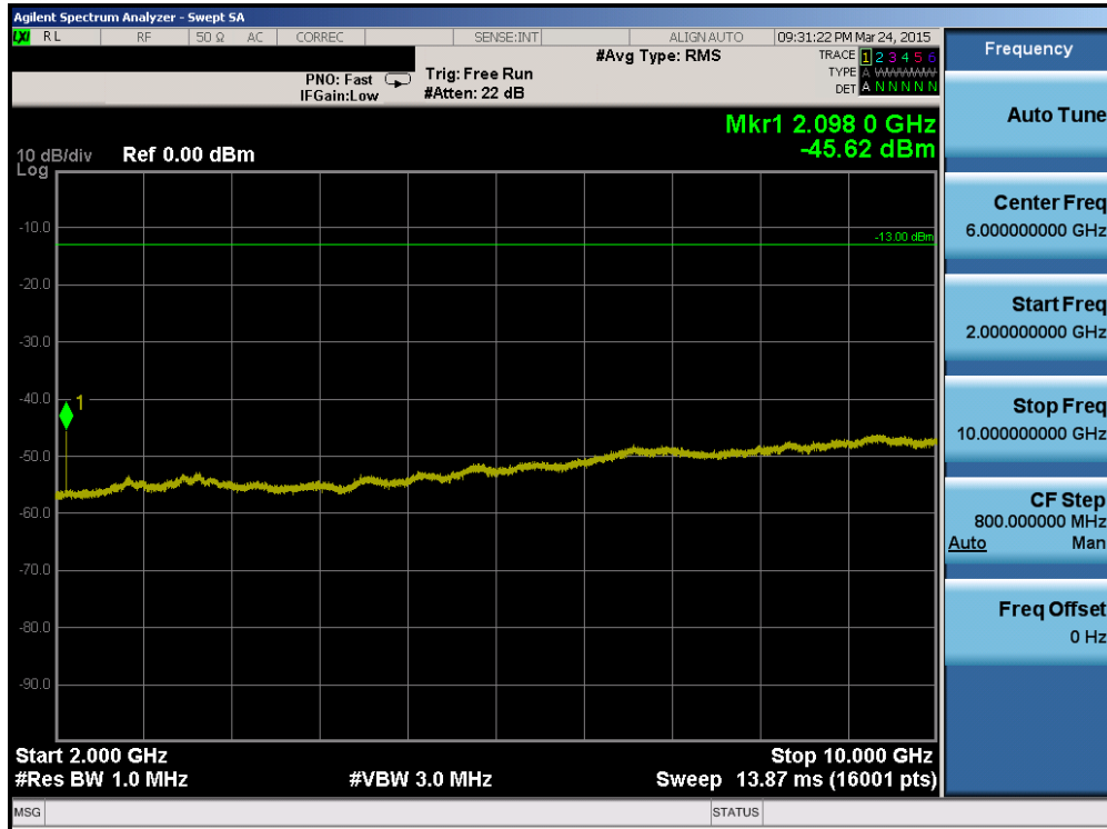
Plot 6-35. Conducted Spurious Plot (Band 12 – 3.0MHz QPSK – RB Size 1, RB Offset 0 – Low Channel)
