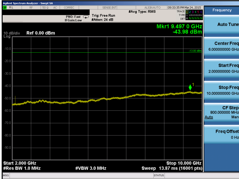
Plot 6-41. Conducted Spurious Plot (Band 12 – 3.0MHz QPSK – RB Size 1, RB Offset 0 – High Channel)
