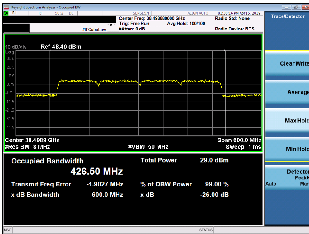
Plot 7-48. Occupied Bandwidth Plot (4CC-100MHz Bandwidth 64QAM Mid Channel)
