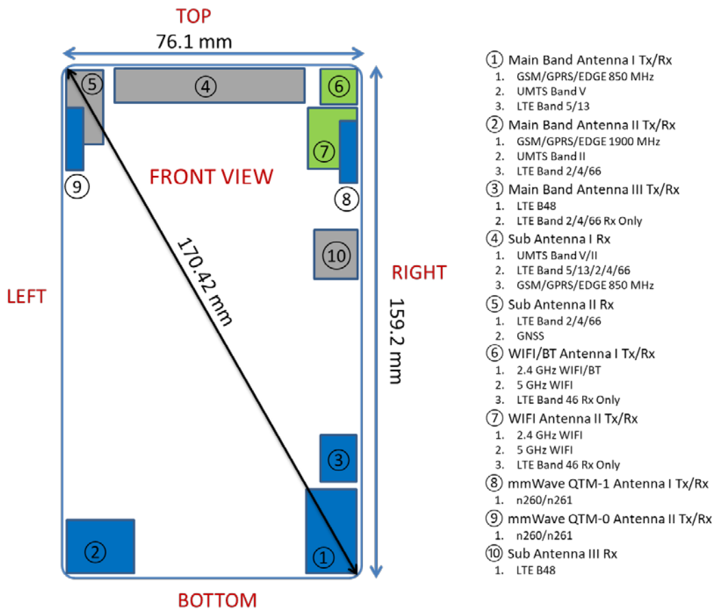
Figure D-1 DUT Antenna Locations
