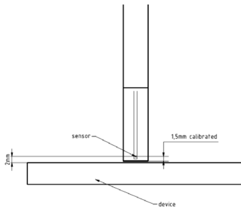
Figure D-2 EUmWV3 Probe
