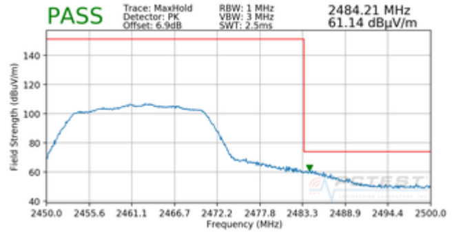
Plot 7-14. Radiated Restricted Band Edge Measurement SISO ANT1 with WCP (Peak)
