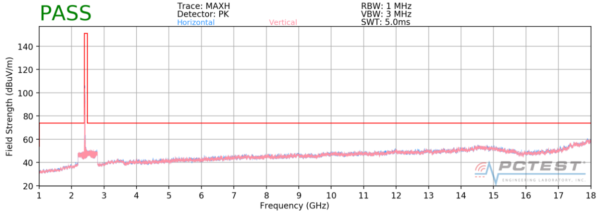
Plot 7-9. Radiated Spurious Plot above 1GHz SISO ANT2 (802.11b – Ch. 1)
