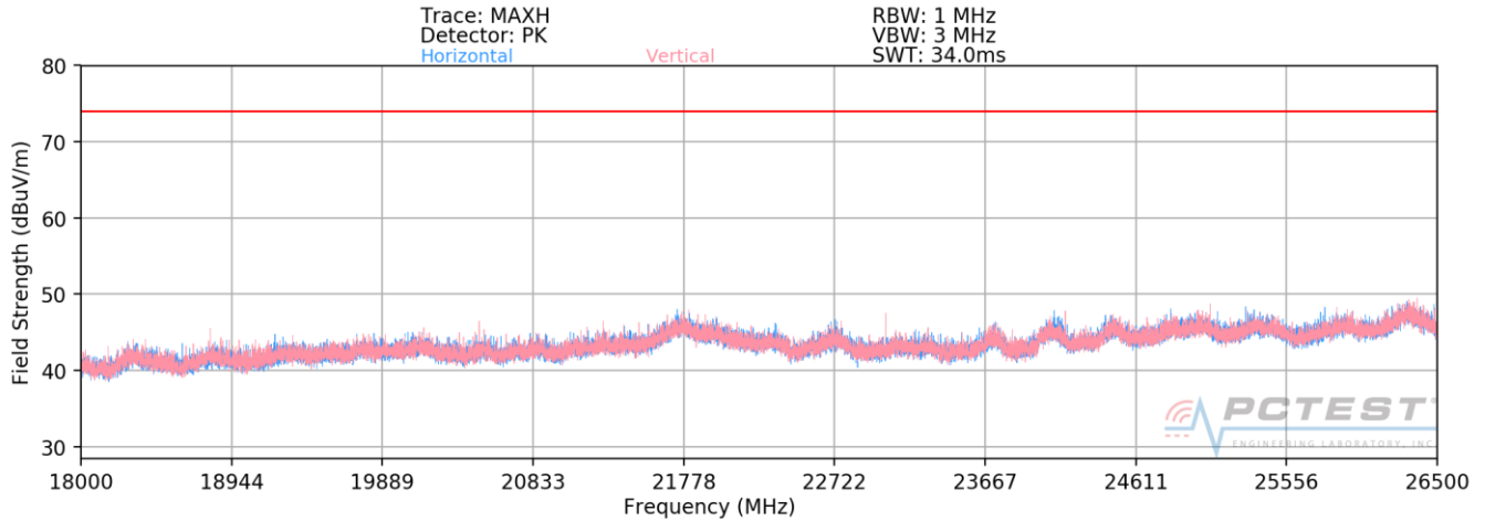
Plot 7-12. Radiated Spurious Plot above 18GHz SISO ANT2
