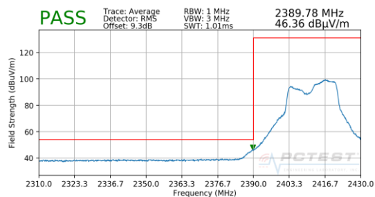
Plot 7-33. Radiated Restricted Lower Band Edge Measurement MIMO (Average)
