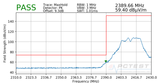
Plot 7-34. Radiated Restricted Lower Band Edge Measurement MIMO (Peak)
