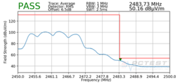
Plot 7-29. Radiated Restricted Upper Band Edge Measurement CDD (Average)
