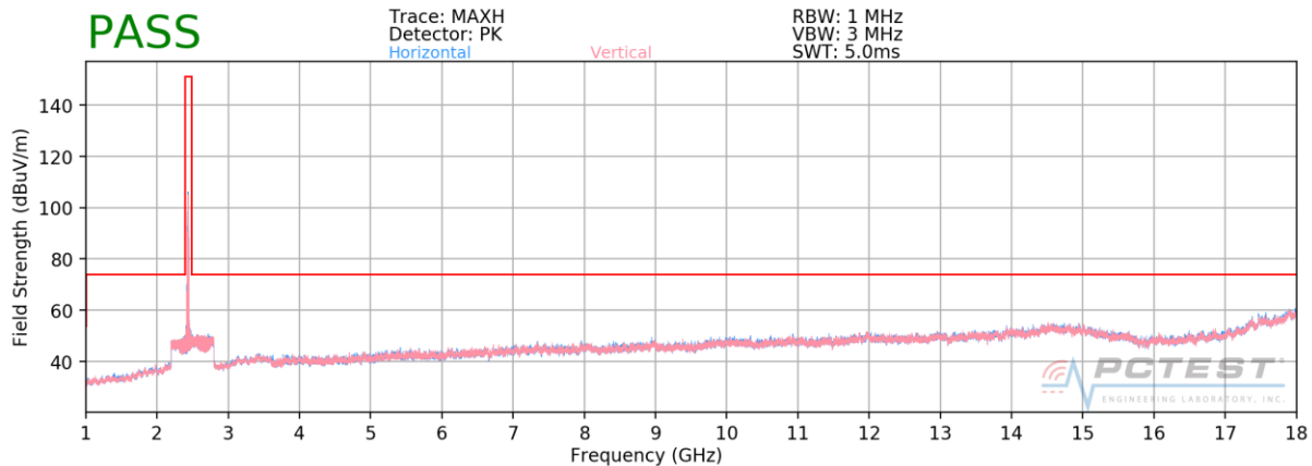
Plot 7-10. Radiated Spurious Plot above 1GHz SISO ANT2 (802.11b – Ch. 6)
