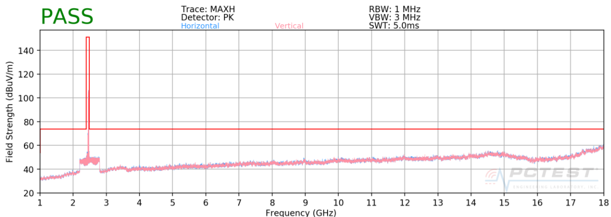
Plot 7-11. Radiated Spurious Plot above 1GHz SISO ANT2 (802.11b – Ch. 11)
