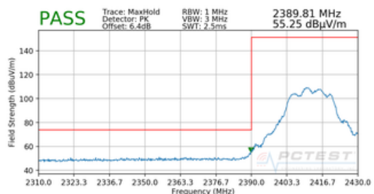
Plot 7-26. Radiated Restricted Lower Band Edge Measurement CDD (Peak)
