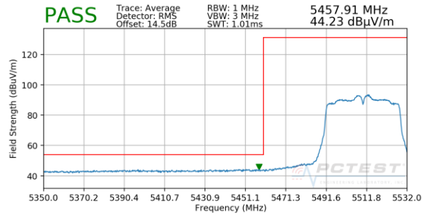
Plot 7-29. Radiated Lower Band Edge Plot SISO ANT1 (Average – UNII Band 2C)
