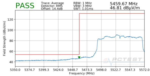
Plot 7-102. Radiated Band Edge Plot MIMO (Average – WCP)
