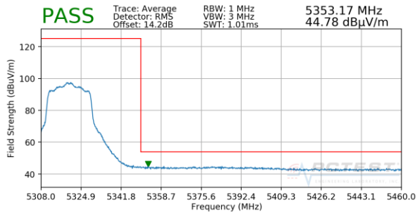
Plot 7-45. Radiated Upper Band Edge Plot SISO ANT2 (Average – UNII Band 2A)
