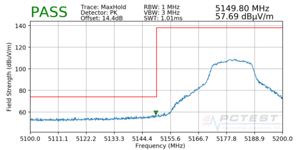
Plot 7-44. Radiated Lower Band Edge Plot SISO ANT2 (Peak – UNII Band 1)
