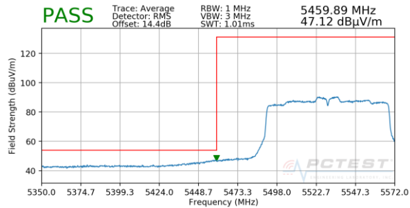
Plot 7-38. Radiated Lower Band Edge Plot SISO ANT1 (Average – UNII Band 2C)
