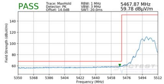
Plot 7-230. Radiated Band Edge Plot (Peak – WCP)
