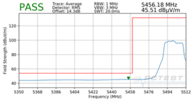
Plot 7-235. Radiated Lower Band Edge Plot (Average – UNII Band 2C)
