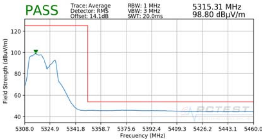
Plot 7-238. Radiated Band Edge Plot (Average – WCP)
