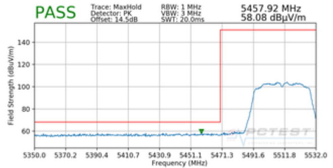
Plot 7-245. Radiated Lower Band Edge Plot (Peak – UNII Band 2C)
