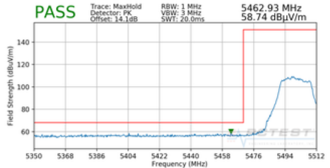
Plot 7-236. Radiated Lower Band Edge Plot (Peak – UNII Band 2C)
