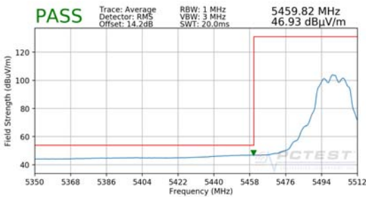
Plot 7-226. Radiated Lower Band Edge Plot (Average – UNII Band 2C)
