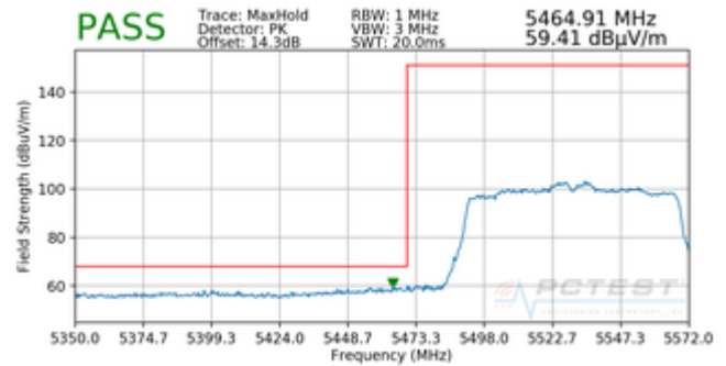
Plot 7-254. Radiated Lower Band Edge Plot (Peak – UNII Band 2C)
