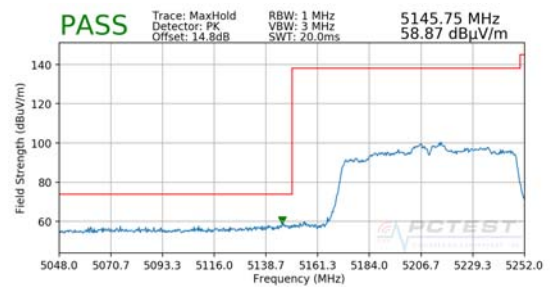
Plot 7-257. Radiated Band Edge Plot (Peak – WCP)
