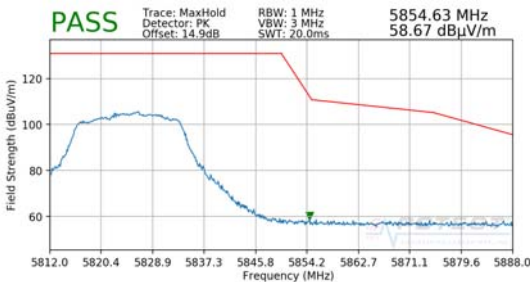
Plot 7-237. Radiated Upper Band Edge Plot (Peak – UNII Band 3)
