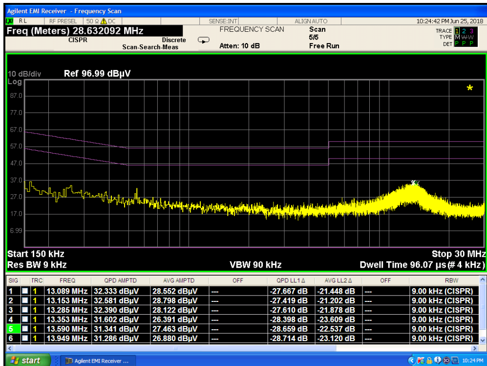
Plot 7-267. Line Conducted Plot with 802.11a UNII Band 3 (N)
