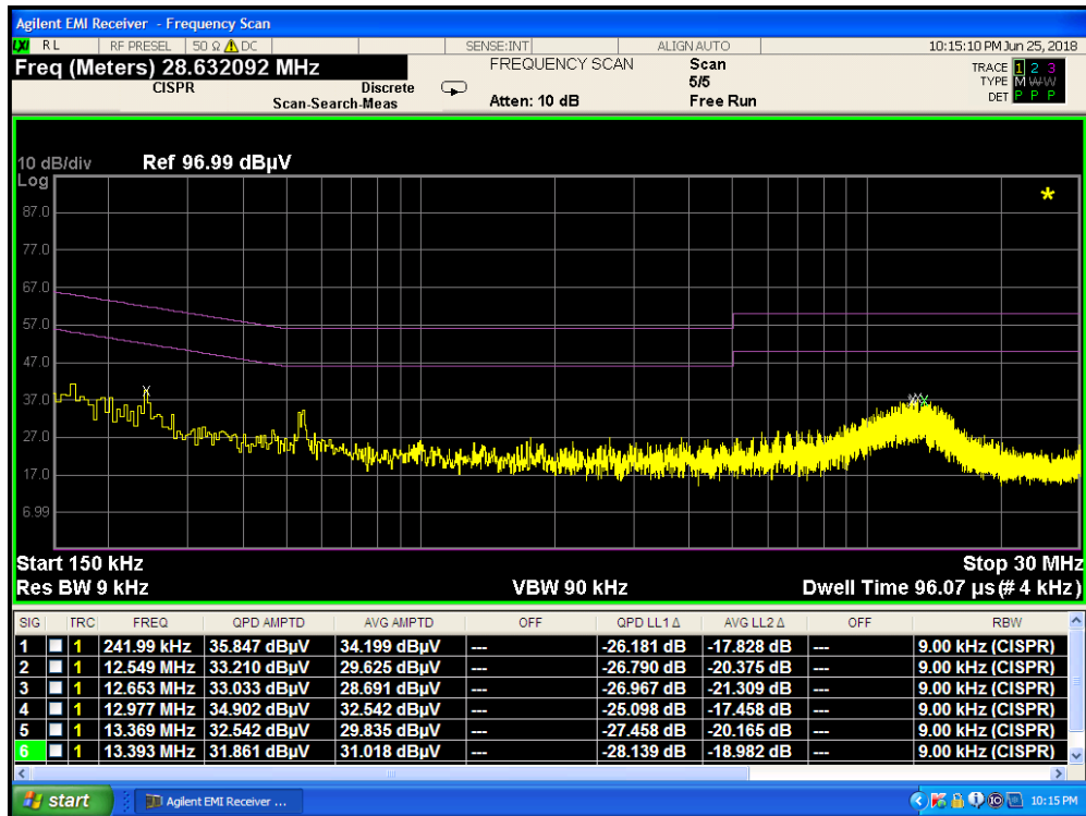
Plot 7-262. Line Conducted Plot with 802.11a UNII Band 2A (L1)
