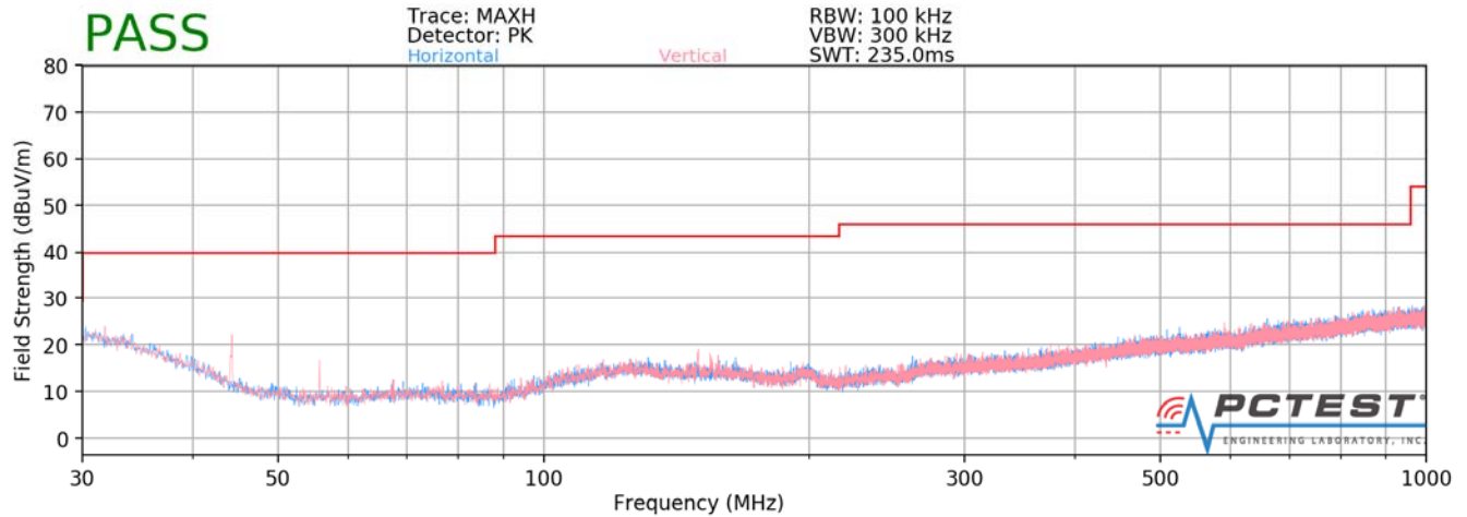
Plot 7-258. Radiated Spurious Plot below 1GHz (802.11a – U3 Ch. 157)
