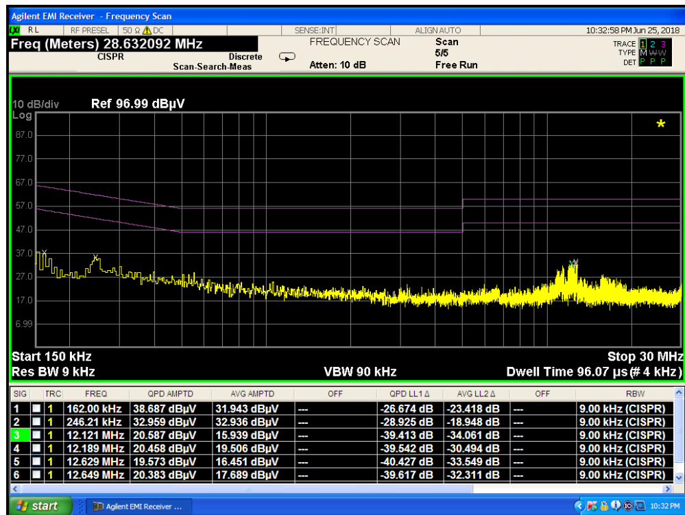
Plot 7-261. Line Conducted Plot with 802.11a UNII Band 1 (N)
