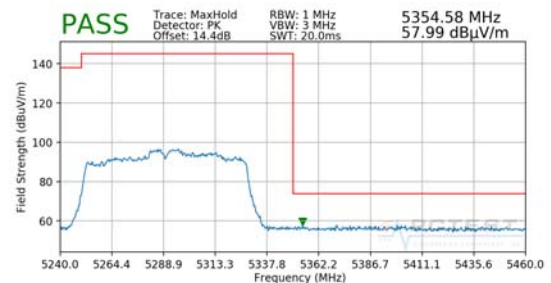
Plot 7-252. Radiated Upper Band Edge Plot (Peak – UNII Band 2A)
