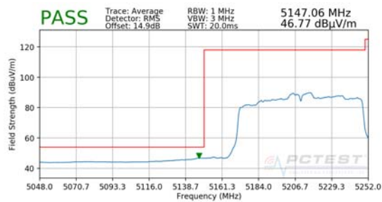
Plot 7-256. Radiated Band Edge Plot (Average – WCP)
