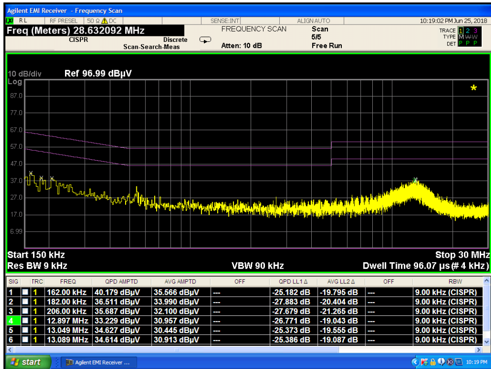
Plot 7-264. Line Conducted Plot with 802.11a UNII Band 2C (L1)
