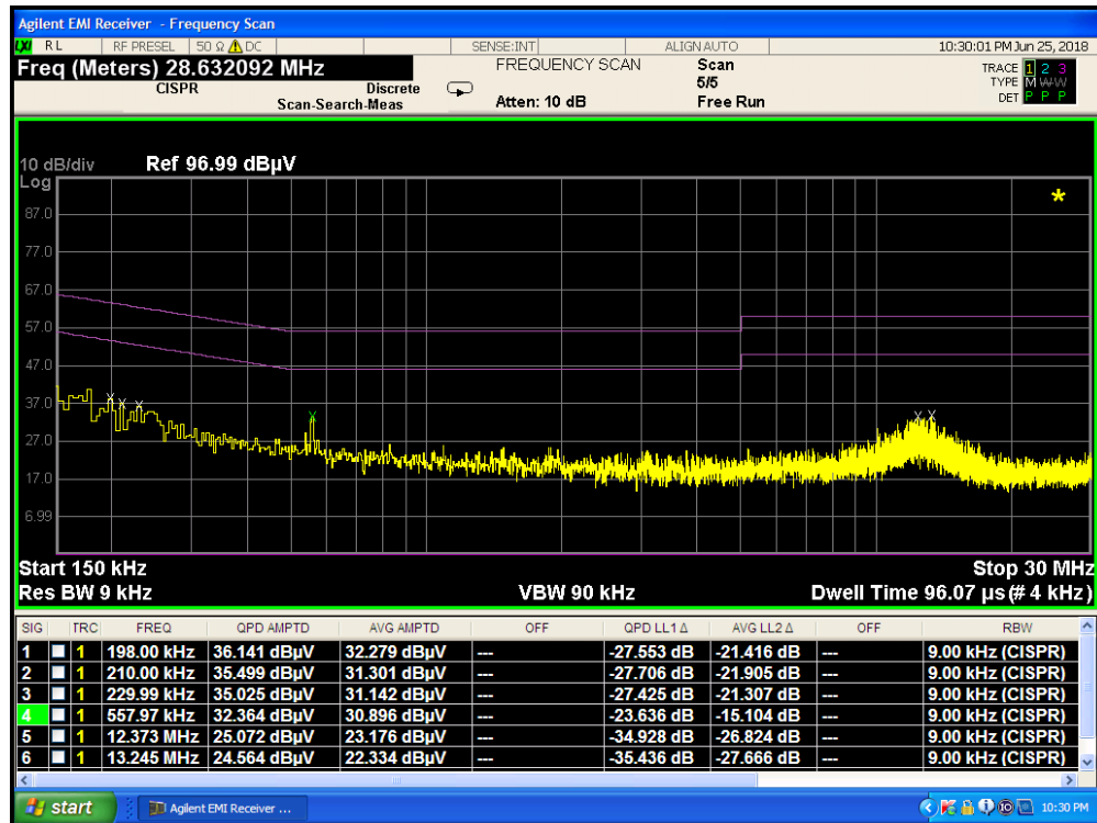
Plot 7-260. Line Conducted Plot with 802.11a UNII Band 1 (L1)
