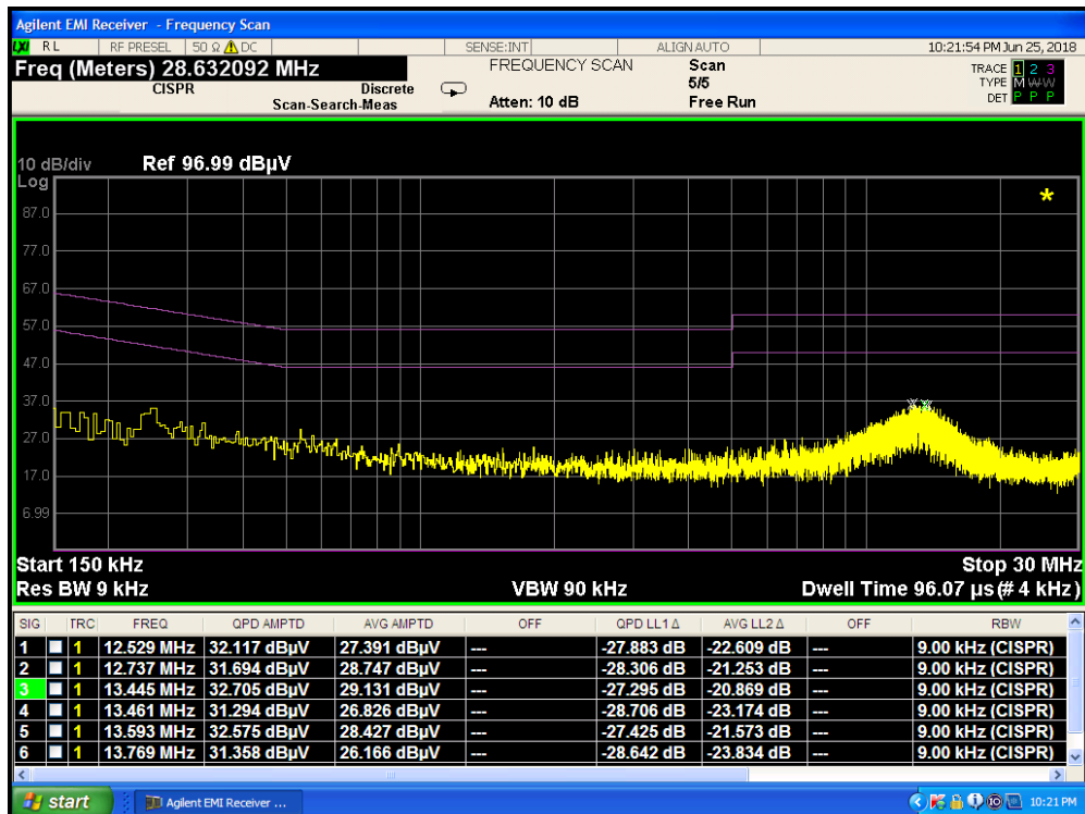
Plot 7-265. Line Conducted Plot with 802.11a UNII Band 2C (N)
