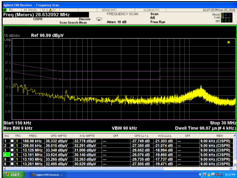
Plot 7-266. Line Conducted Plot with 802.11a UNII Band 3 (L1)
