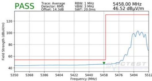
Plot 7-229. Radiated Band Edge Plot (Average – WCP)
