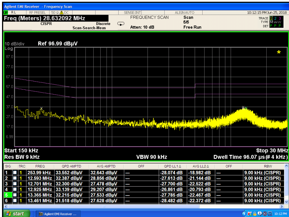
Plot 7-263. Line Conducted Plot with 802.11a UNII Band 2A (N)
