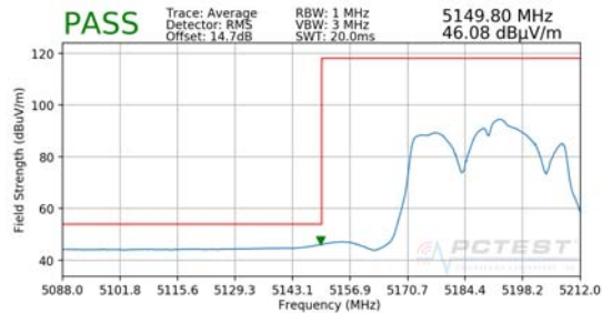
Plot 7-247. Radiated Band Edge Plot (Average – WCP)
