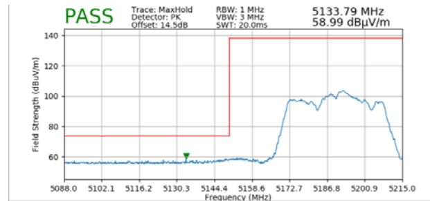
Plot 7-241. Radiated Lower Band Edge Plot (Peak – UNII Band 1)
