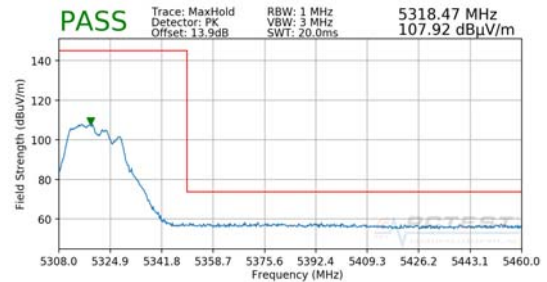
Plot 7-239. Radiated Band Edge Plot (Peak – WCP)
