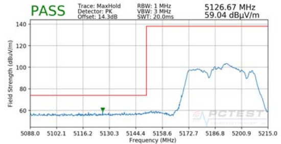
Plot 7-248. Radiated Band Edge Plot (Peak – WCP)
