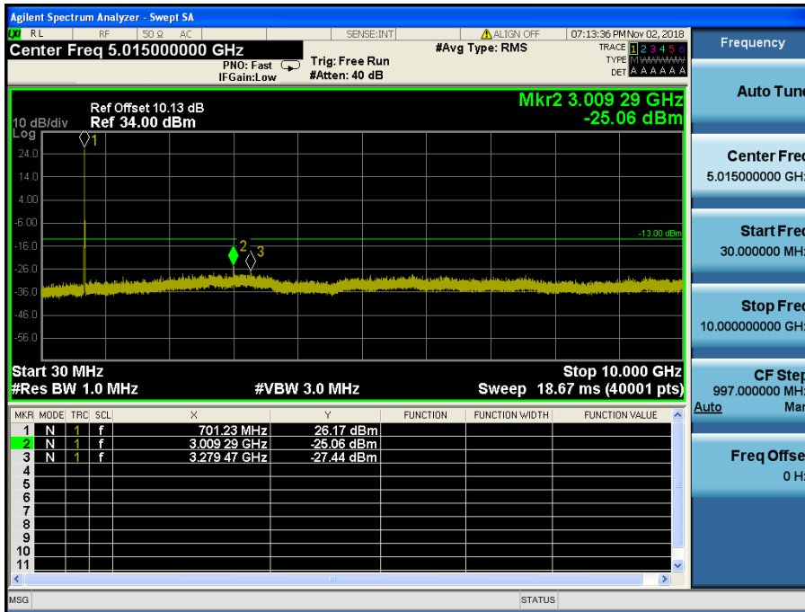
LTE Band 12,17 / 10MHz / 16QAM - RB Size/Offset (25/0) – Low Channel
