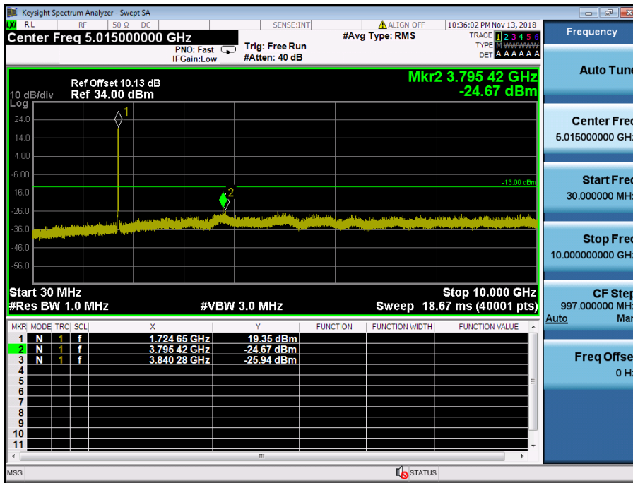
LTE Band 4 / 20MHz / 64QAM - RB Size/Offset (50/50) –Low Channel
