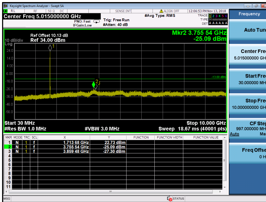
LTE Band 4 / 10MHz / QPSK - RB Size/Offset (25/0) – Low Channel
