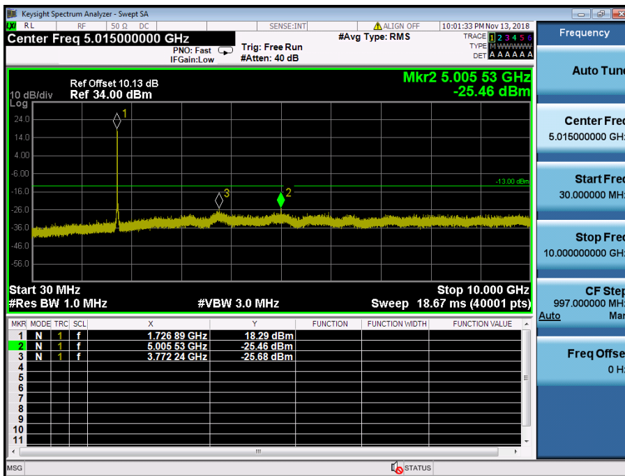
LTE Band 4 / 15MHz / 64QAM - RB Size/Offset (75/0) – Mid Channel
