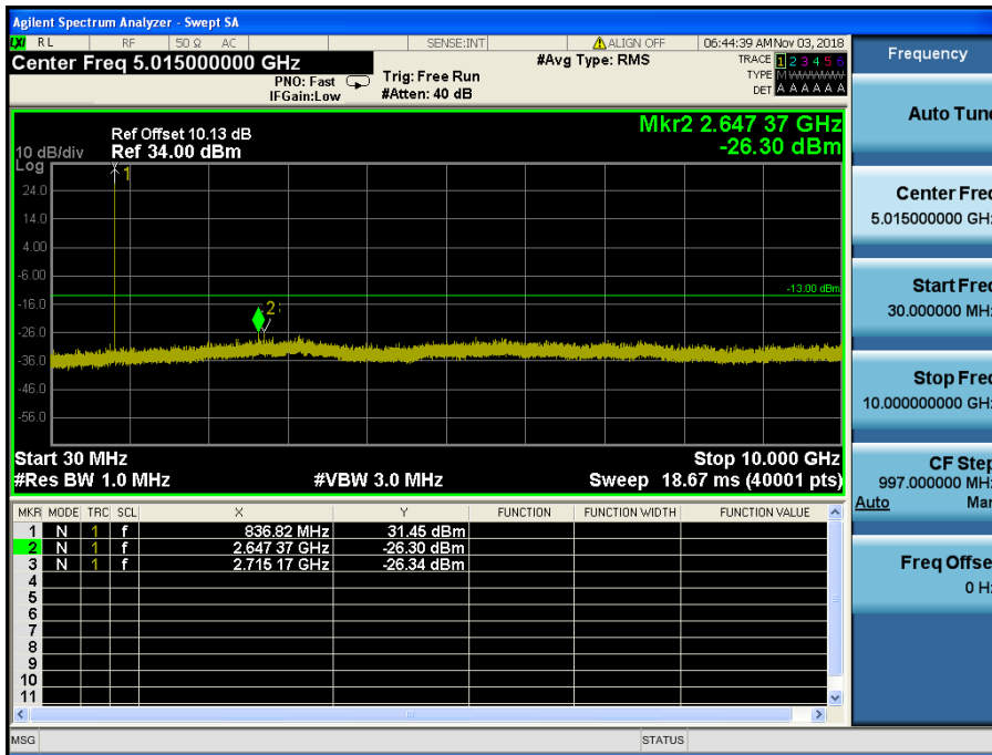
LTE Band 5 / 1.4MHz / 64QAM - RB Size/Offset (1/2) – Mid Channel
