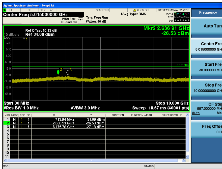
LTE Band 12,17 / 5MHz / QPSK - RB Size/Offset (1/12) – High Channel
